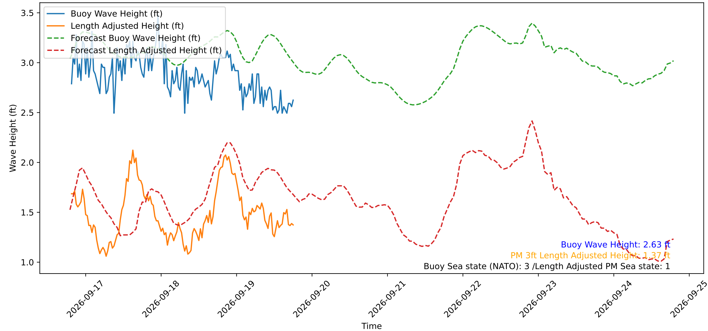
Wave Heights over Time for Green Beach at 2026-09-19 19:01:12
