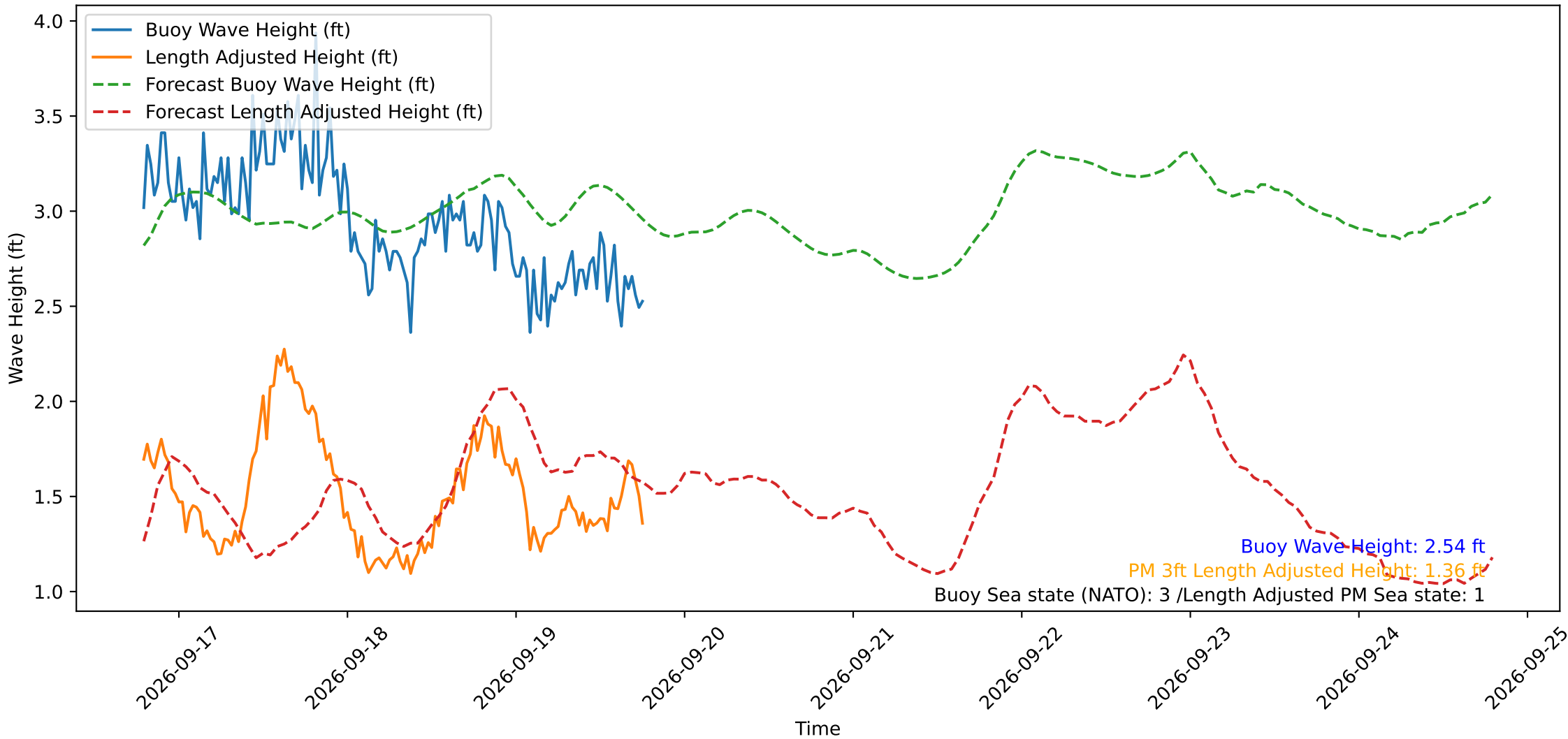
Wave Heights over Time for Oceanside Harbor at 2026-09-19 19:00:30
