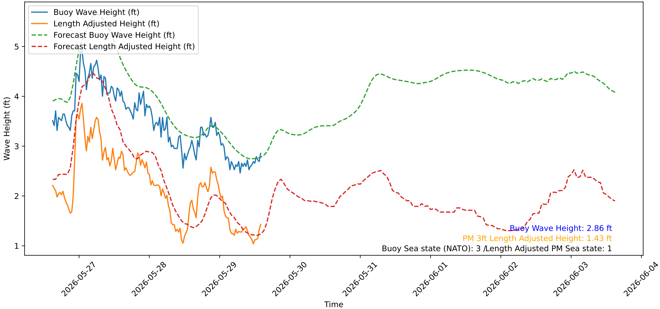
Wave Heights over Time for Green Beach at 2026-05-29 15:01:03
