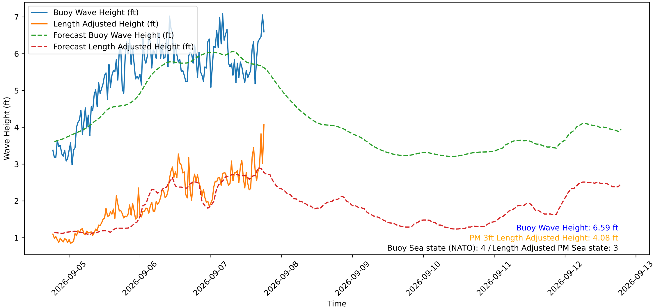
Wave Heights over Time for Oceanside Harbor at 2026-09-07 18:40:29
