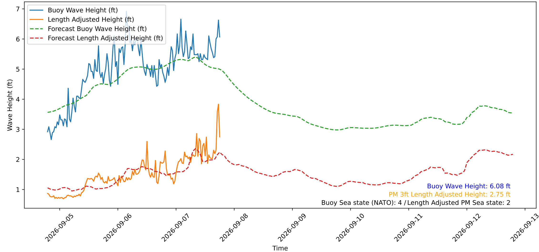
Wave Heights over Time for Red Beach at 2026-09-07 18:40:48
