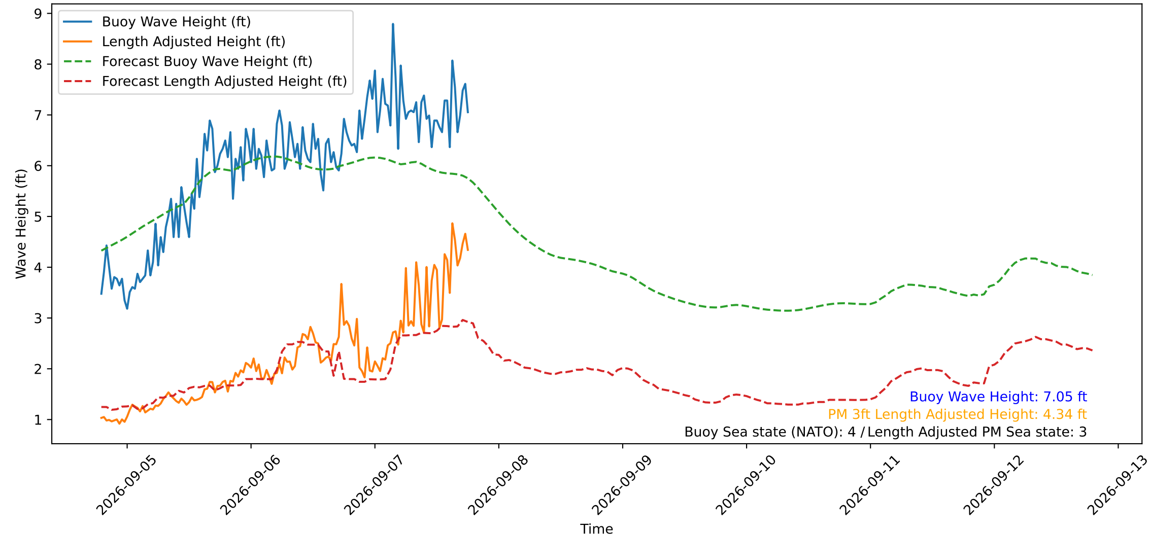
Wave Heights over Time for Green Beach at 2026-09-07 18:41:11
