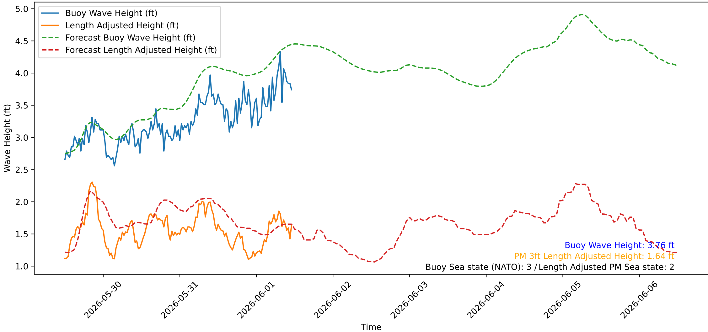
Wave Heights over Time for Green Beach at 2026-06-01 12:01:08
