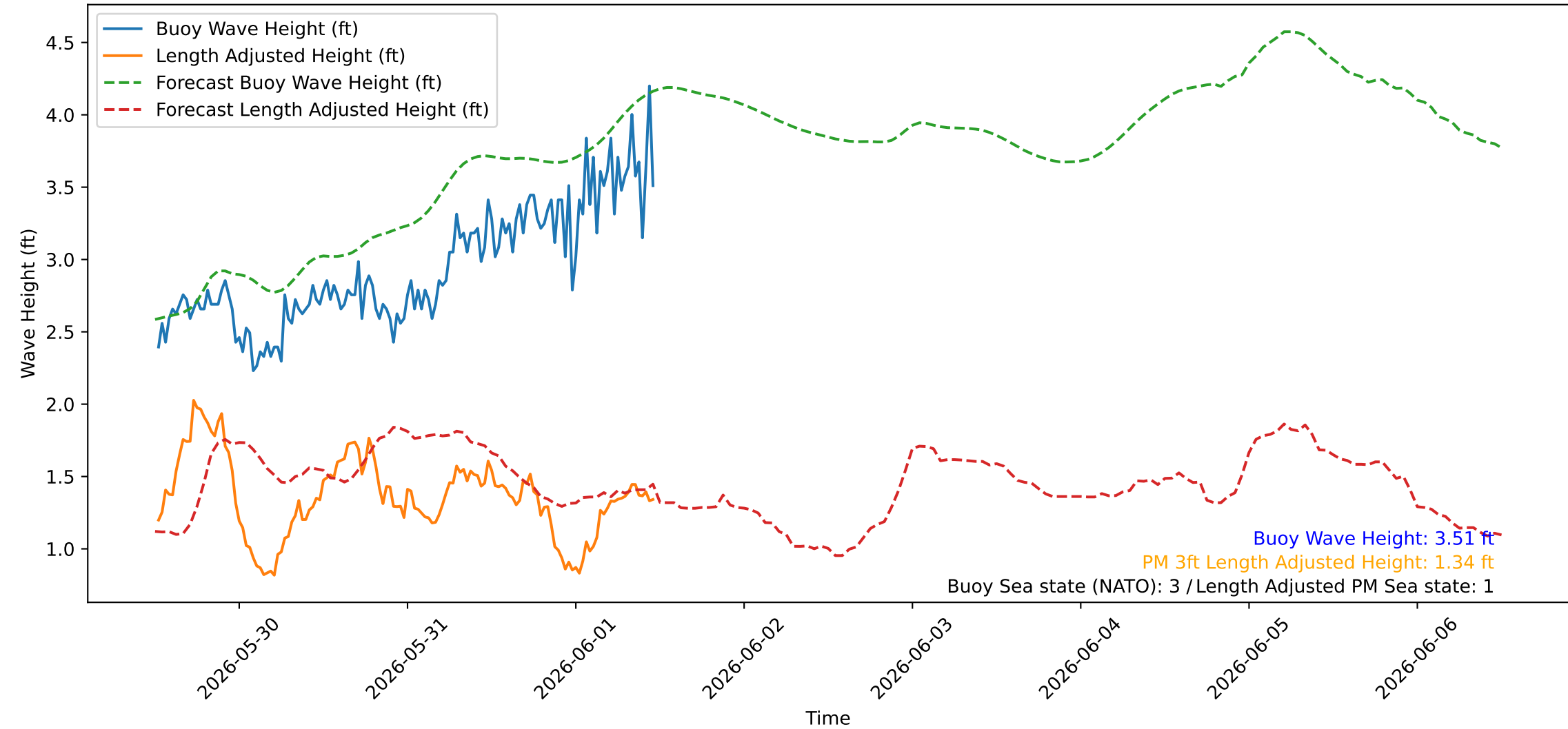
Wave Heights over Time for Red Beach at 2026-06-01 12:00:45
