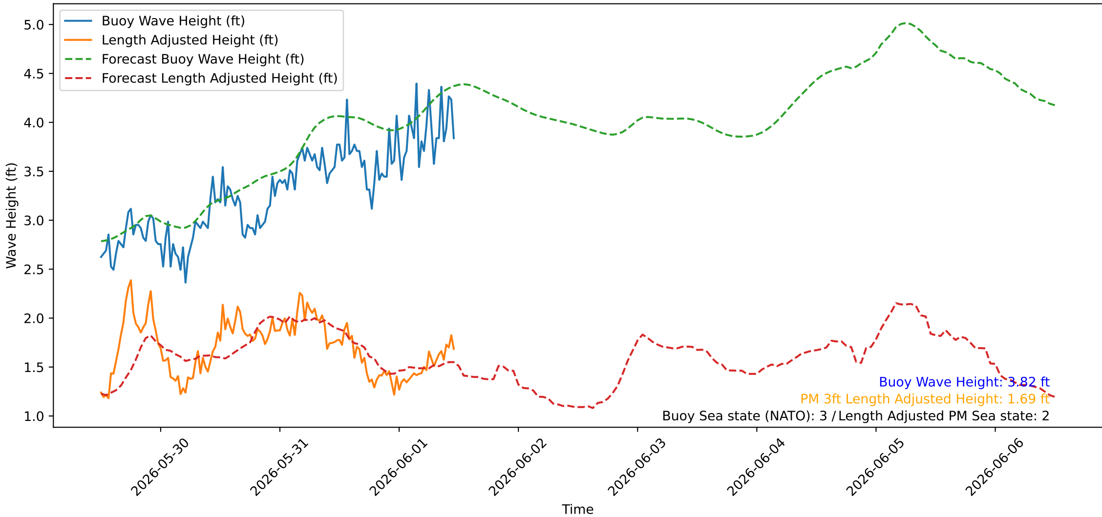
Wave Heights over Time for Oceanside Harbor at 2026-06-01 12:00:25
