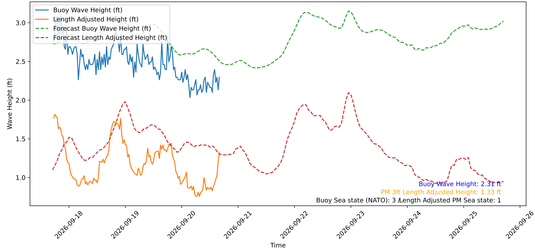
Wave Heights over Time for Red Beach at 2026-09-20 17:00:49
