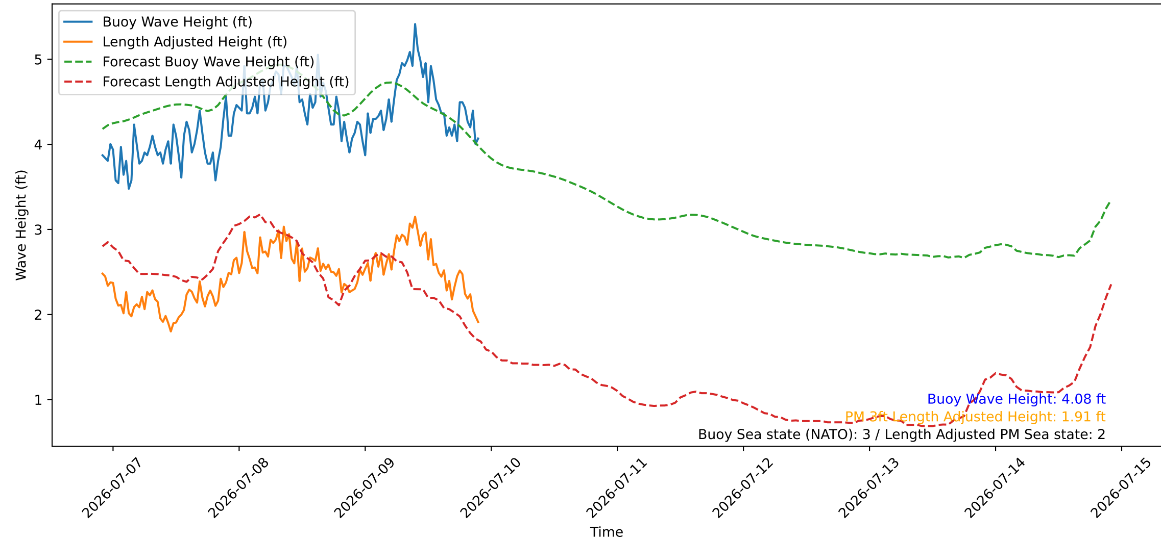
Wave Heights over Time for Oceanside Harbor at 2026-07-09 22:10:25
