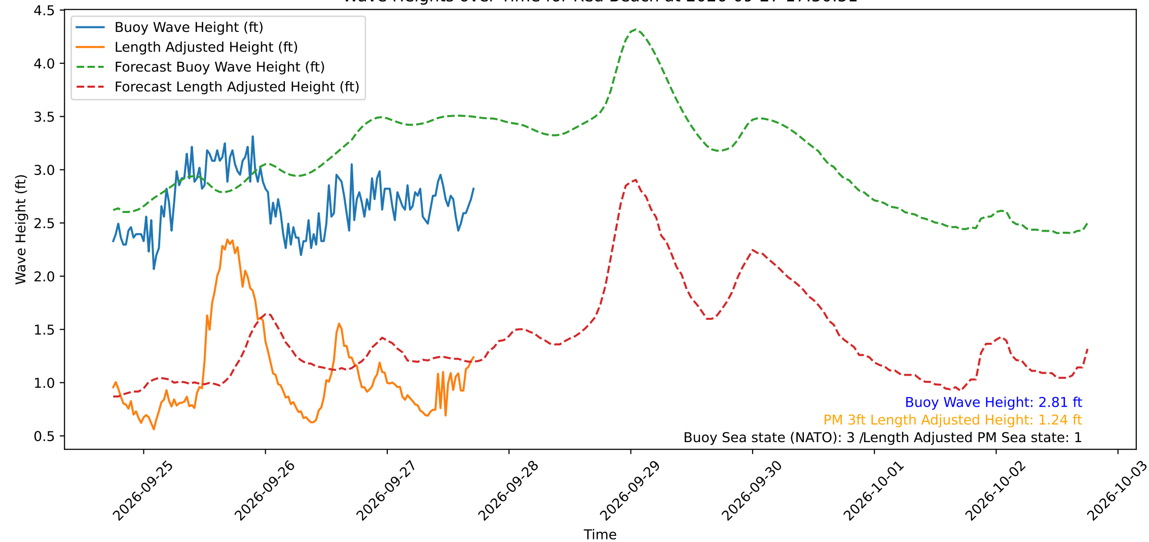
Wave Heights over Time for Red Beach at 2026-09-27 17:50:51
