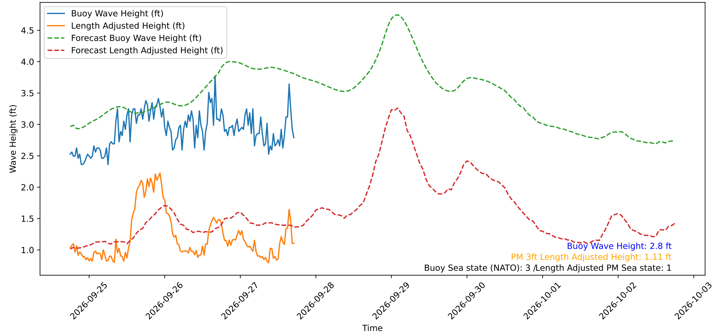
Wave Heights over Time for Oceanside Harbor at 2026-09-27 17:50:30
