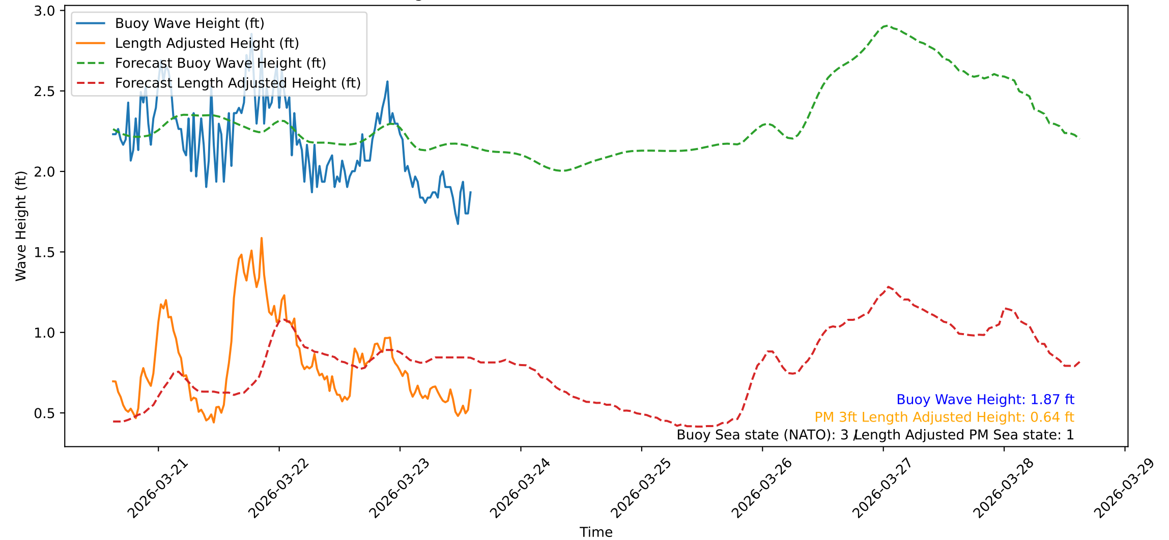
Wave Heights over Time for Red Beach at 2026-03-23 14:40:48
