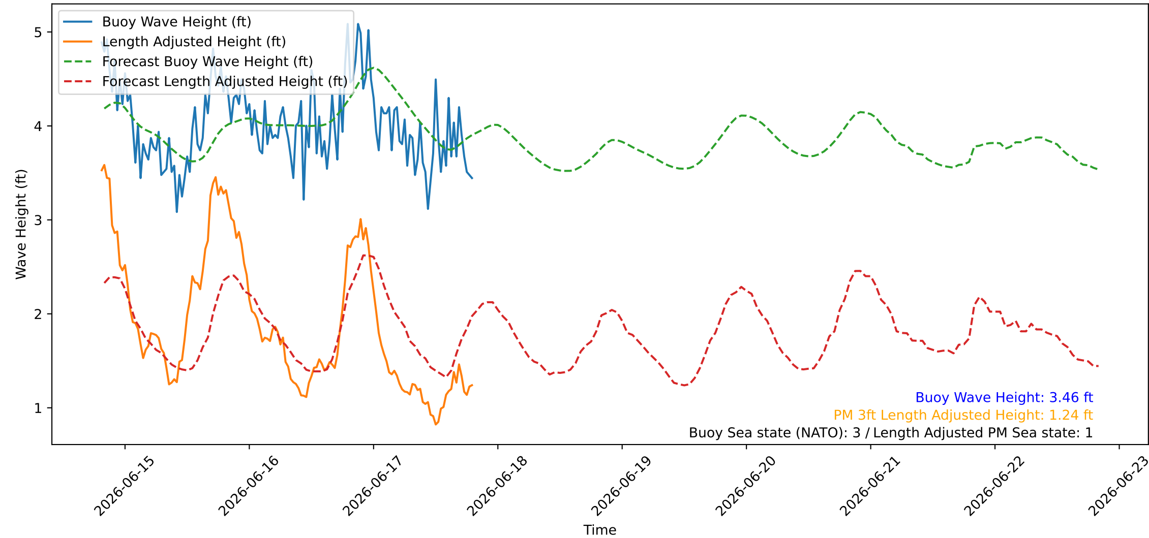
Wave Heights over Time for Green Beach at 2026-06-17 19:41:09
