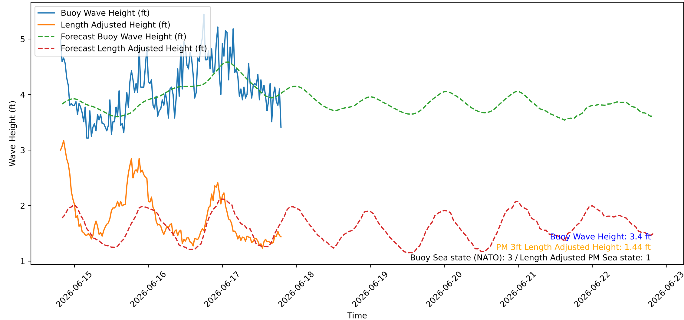
Wave Heights over Time for Oceanside Harbor at 2026-06-17 19:40:26
