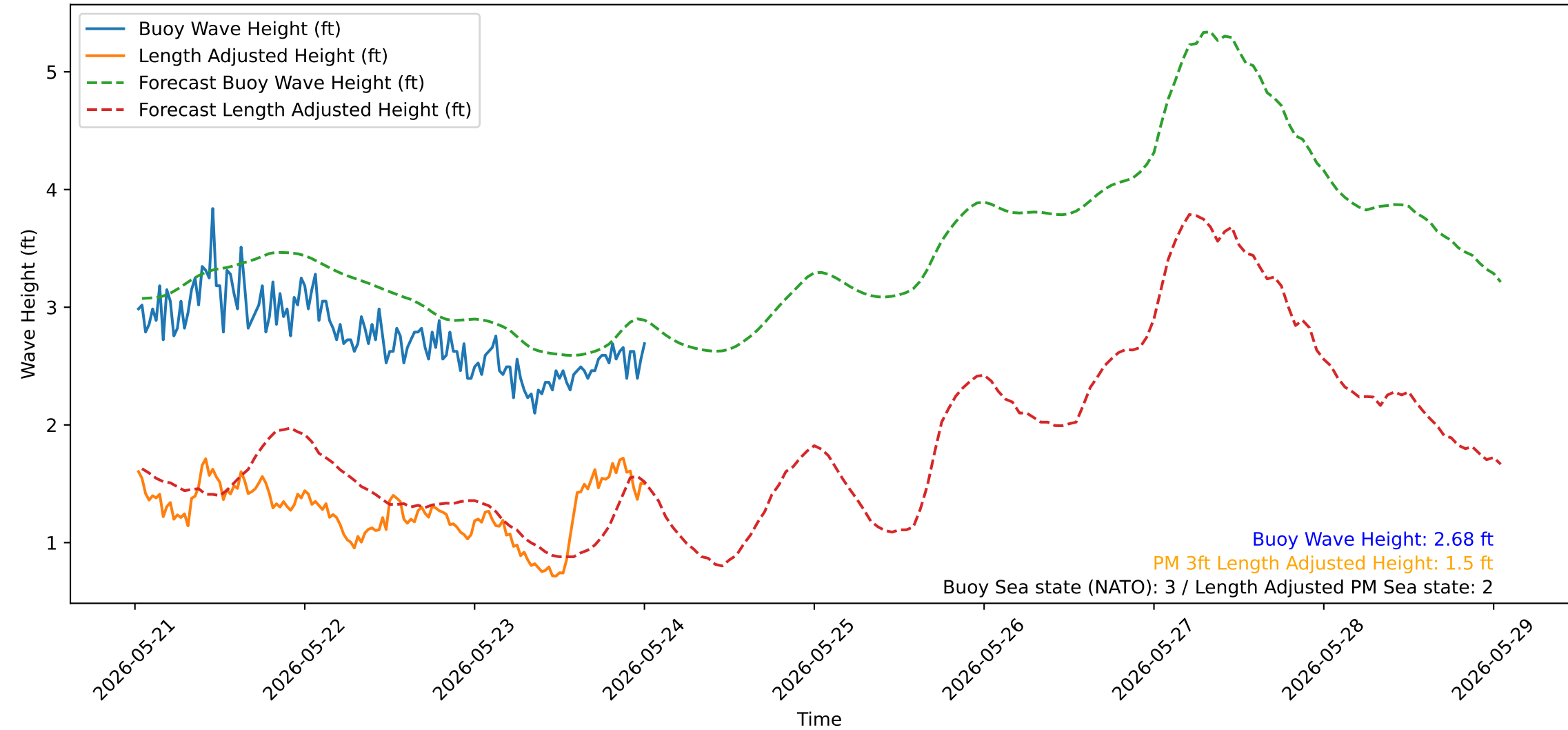
Wave Heights over Time for Oceanside Harbor at 2026-05-24 00:30:31
