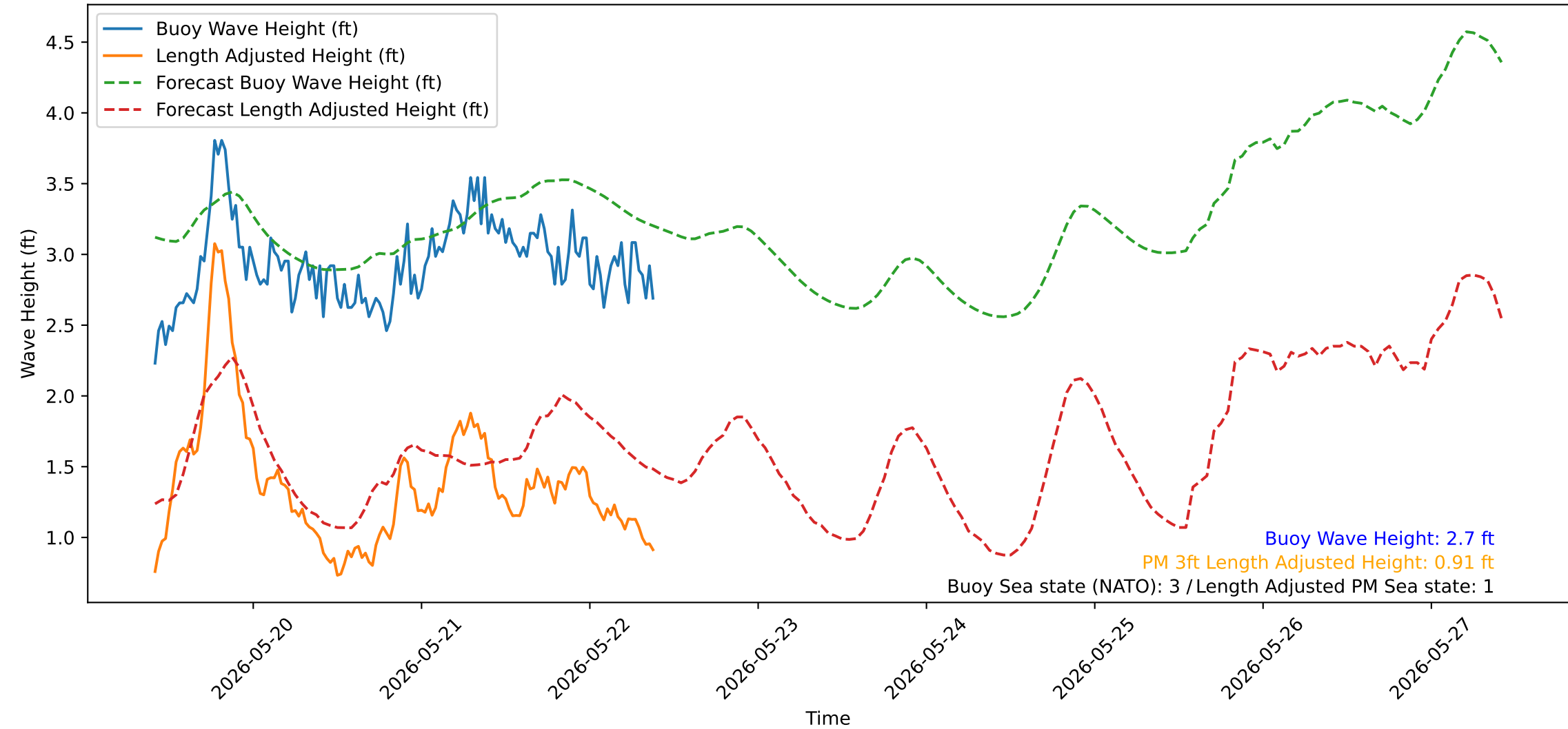
Wave Heights over Time for Green Beach at 2026-05-22 10:01:14
