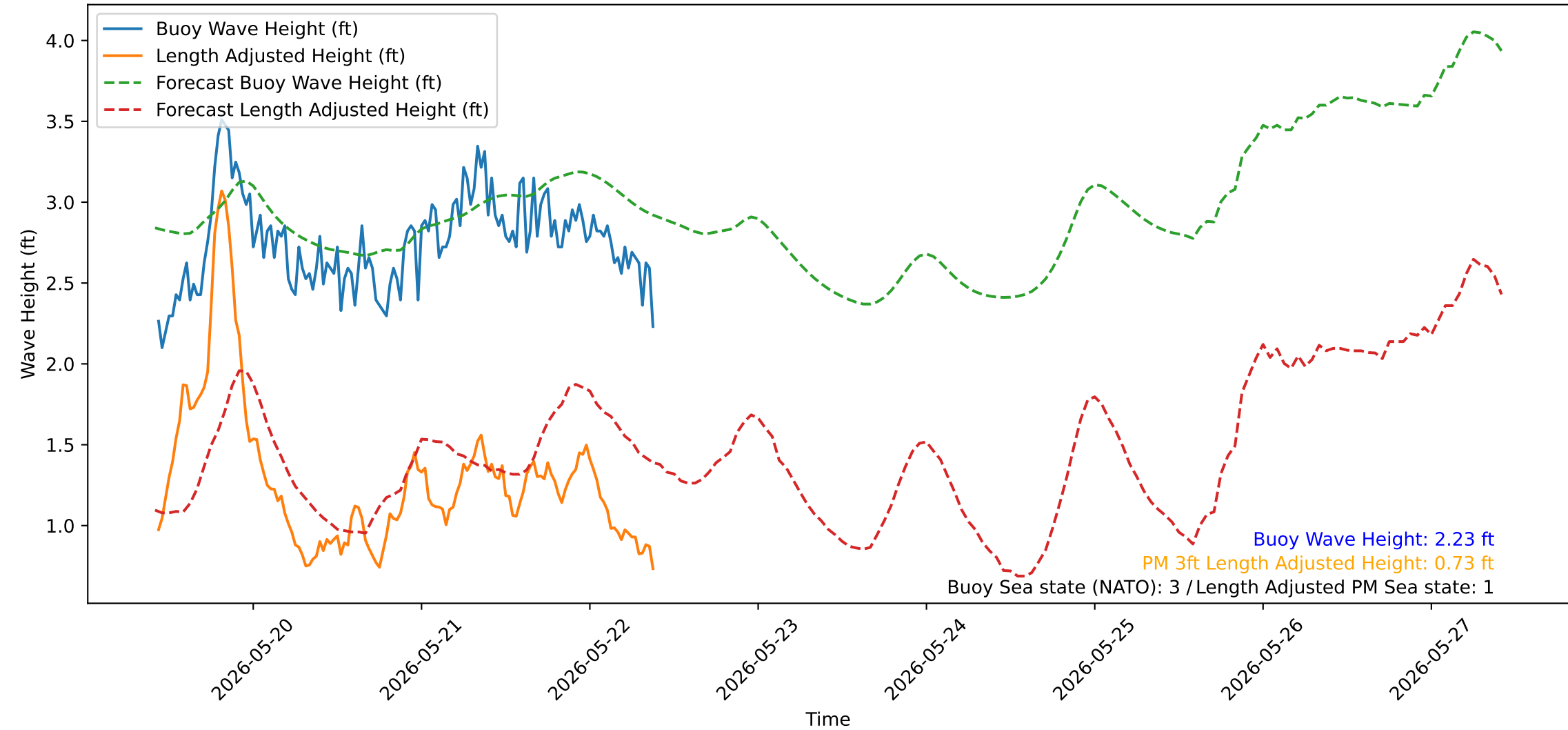
Wave Heights over Time for Red Beach at 2026-05-22 10:00:51
