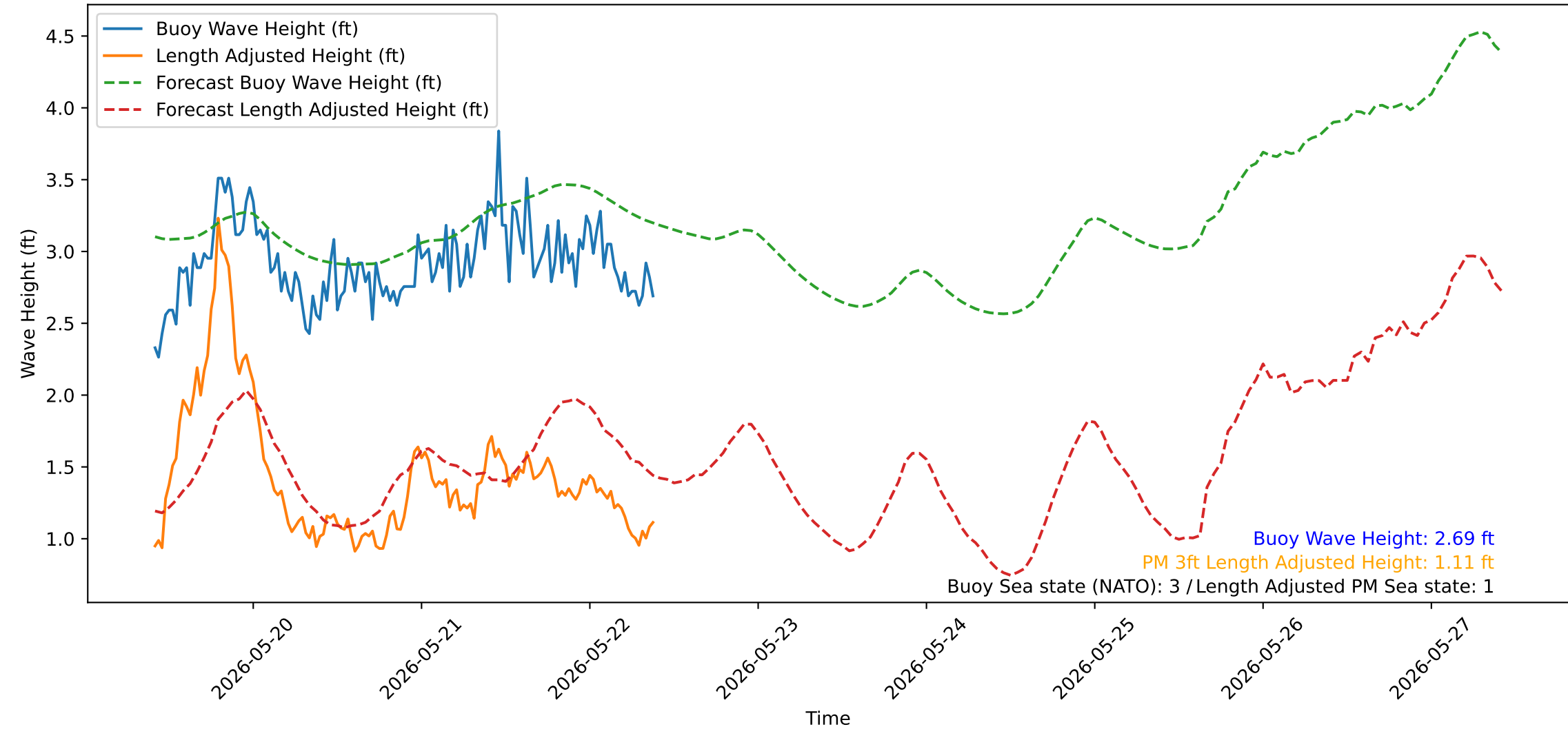
Wave Heights over Time for Oceanside Harbor at 2026-05-22 10:00:32
