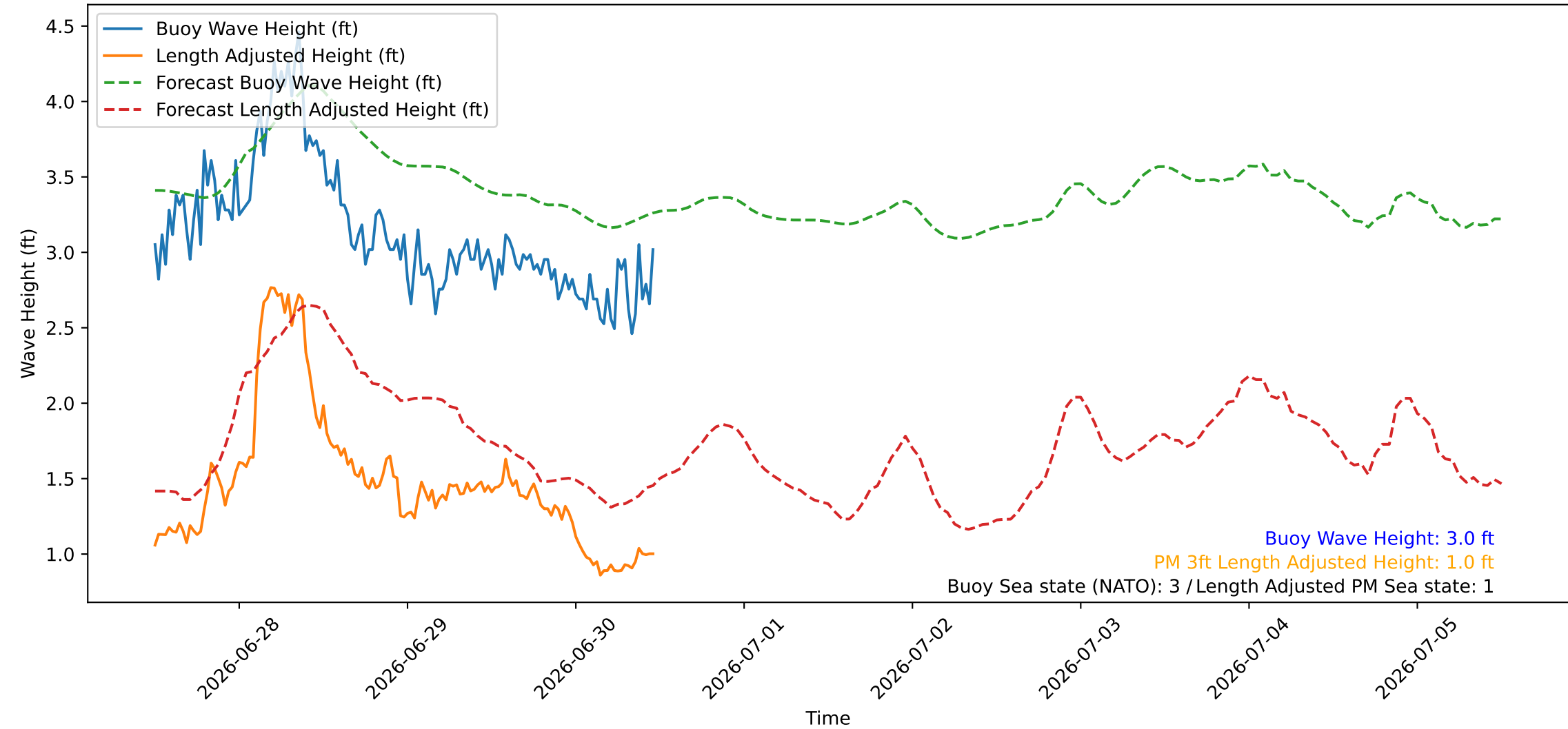
Wave Heights over Time for Red Beach at 2026-06-30 11:50:47
