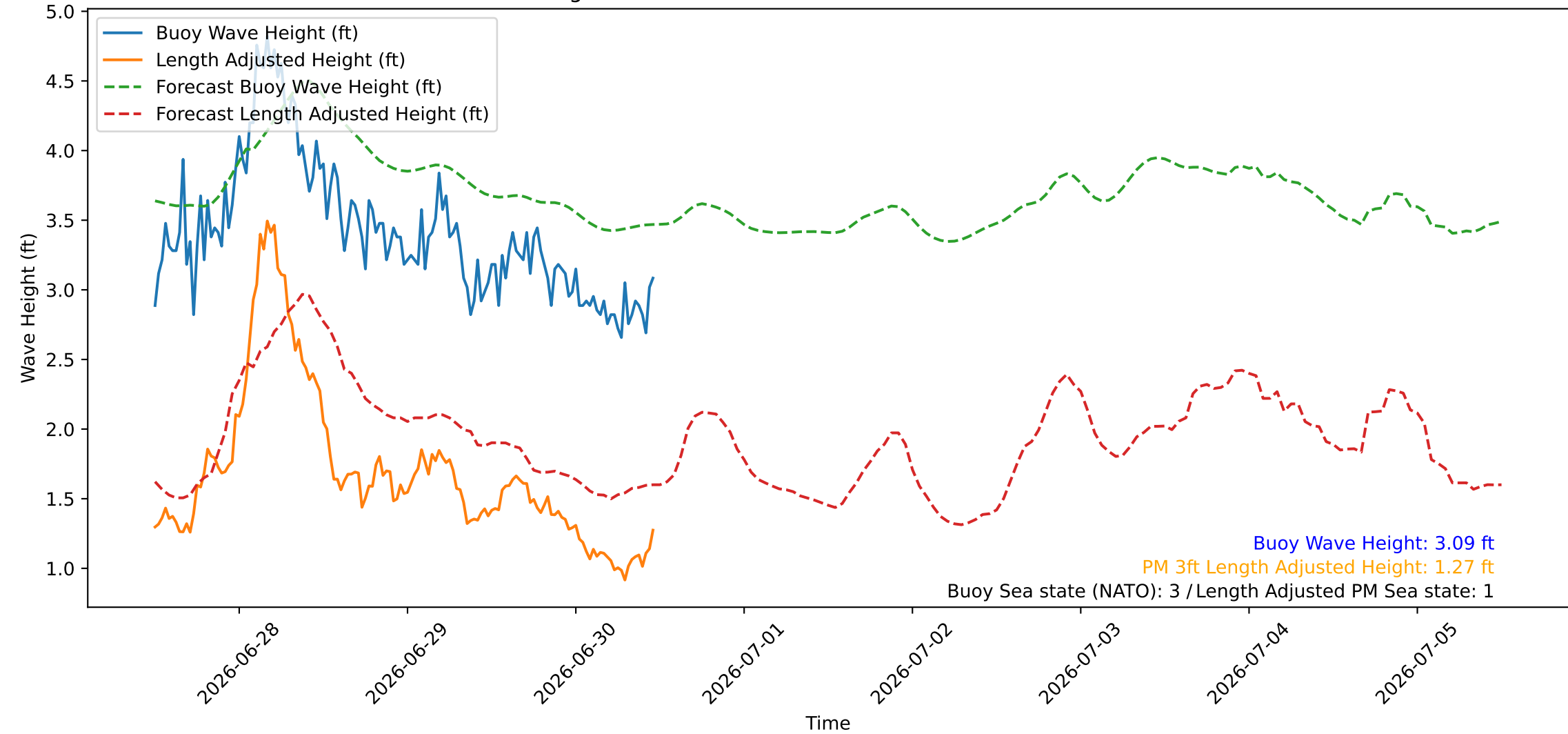
Wave Heights over Time for Green Beach at 2026-06-30 11:51:10
