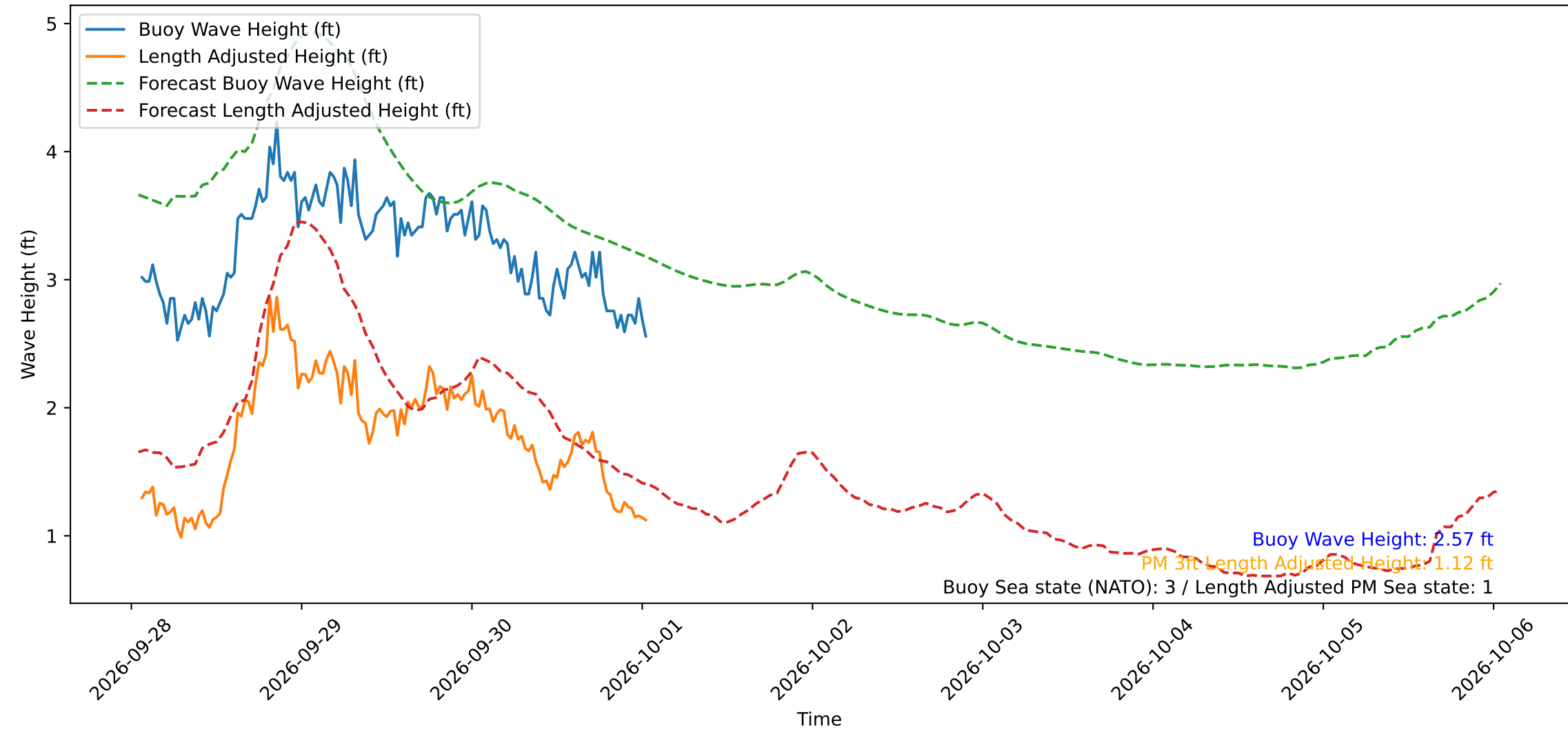
Wave Heights over Time for Oceanside Harbor at 2026-10-01 01:20:30
