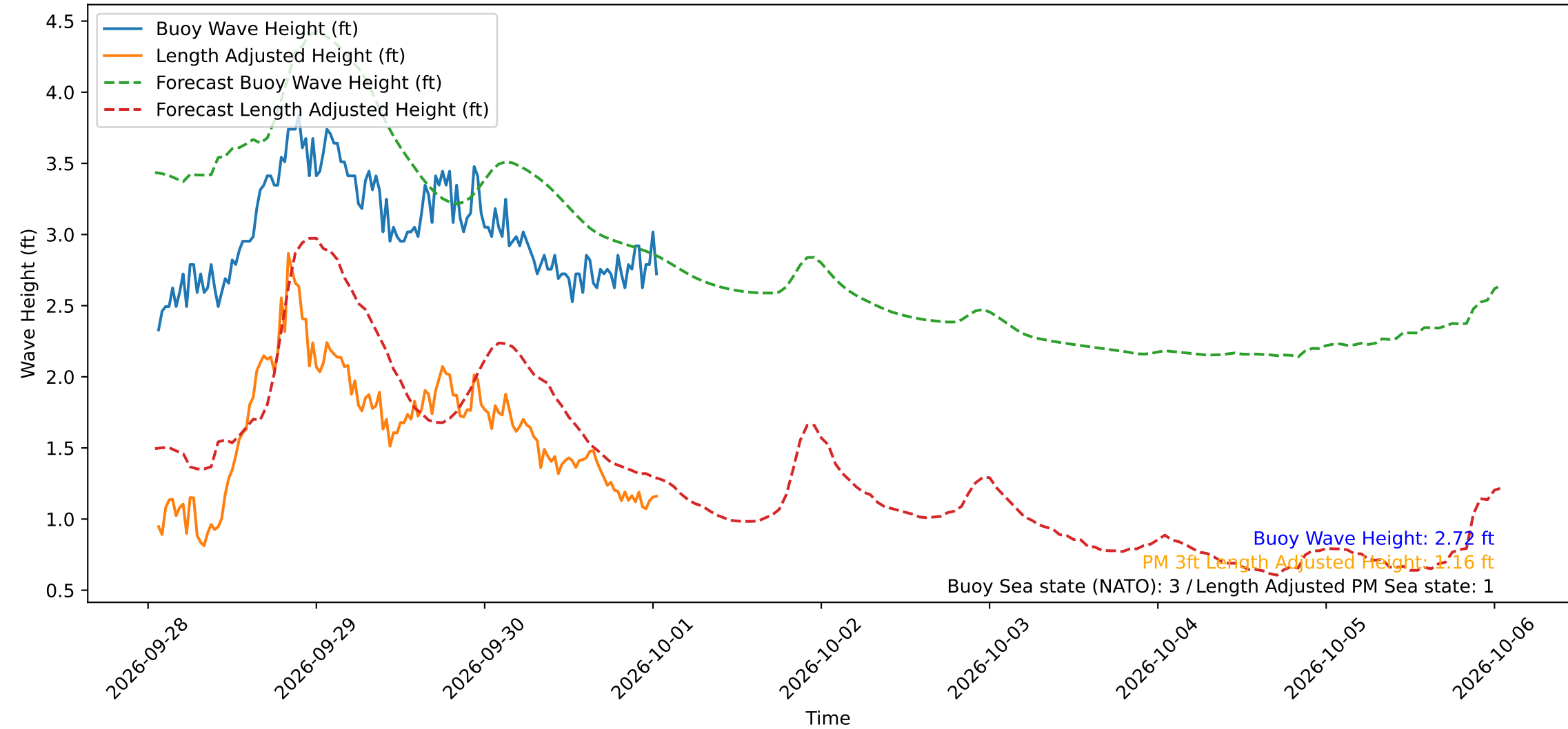
Wave Heights over Time for Red Beach at 2026-10-01 01:20:51
