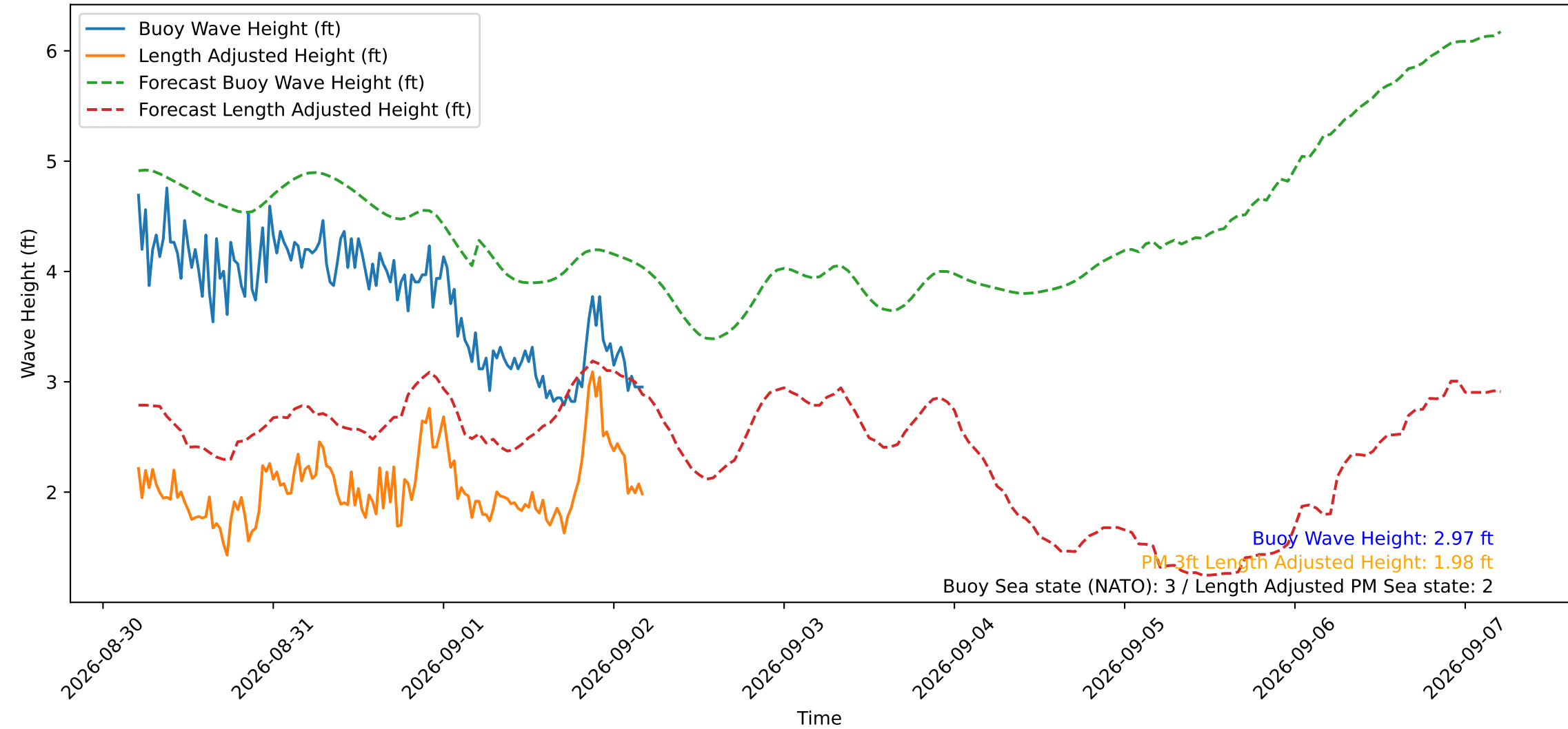
Wave Heights over Time for Green Beach at 2026-09-02 04:51:15
