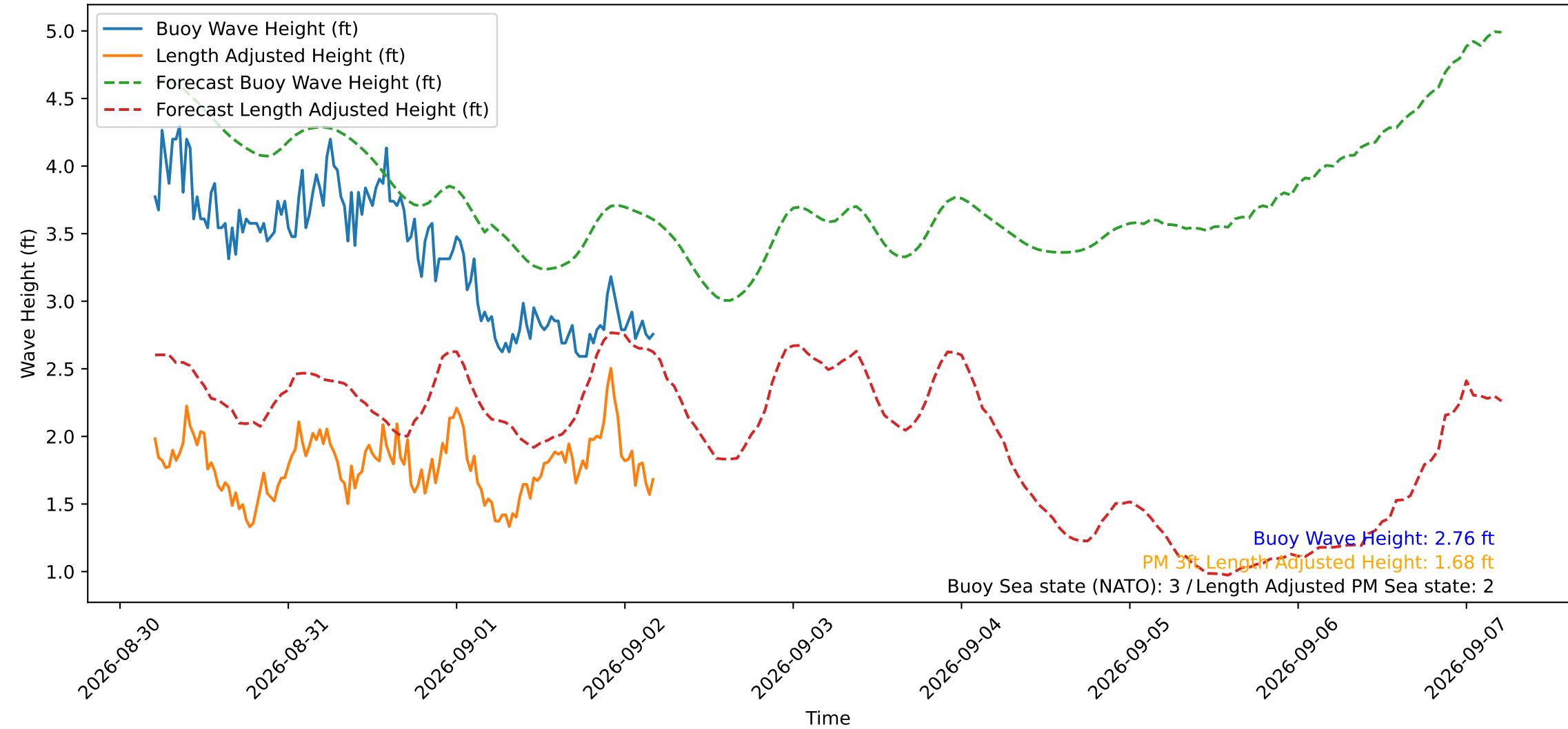
Wave Heights over Time for Red Beach at 2026-09-02 04:50:51
