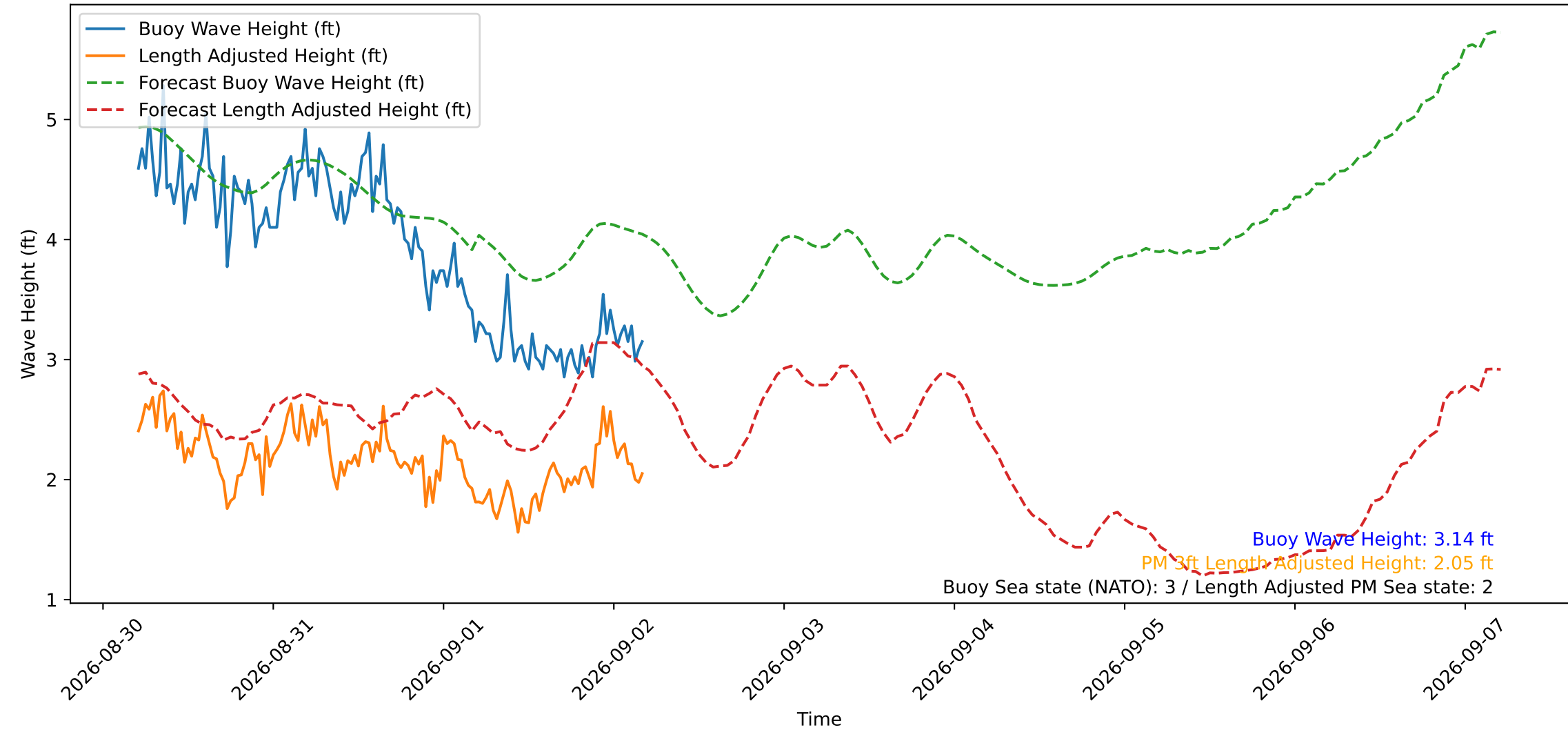
Wave Heights over Time for Oceanside Harbor at 2026-09-02 04:50:30
