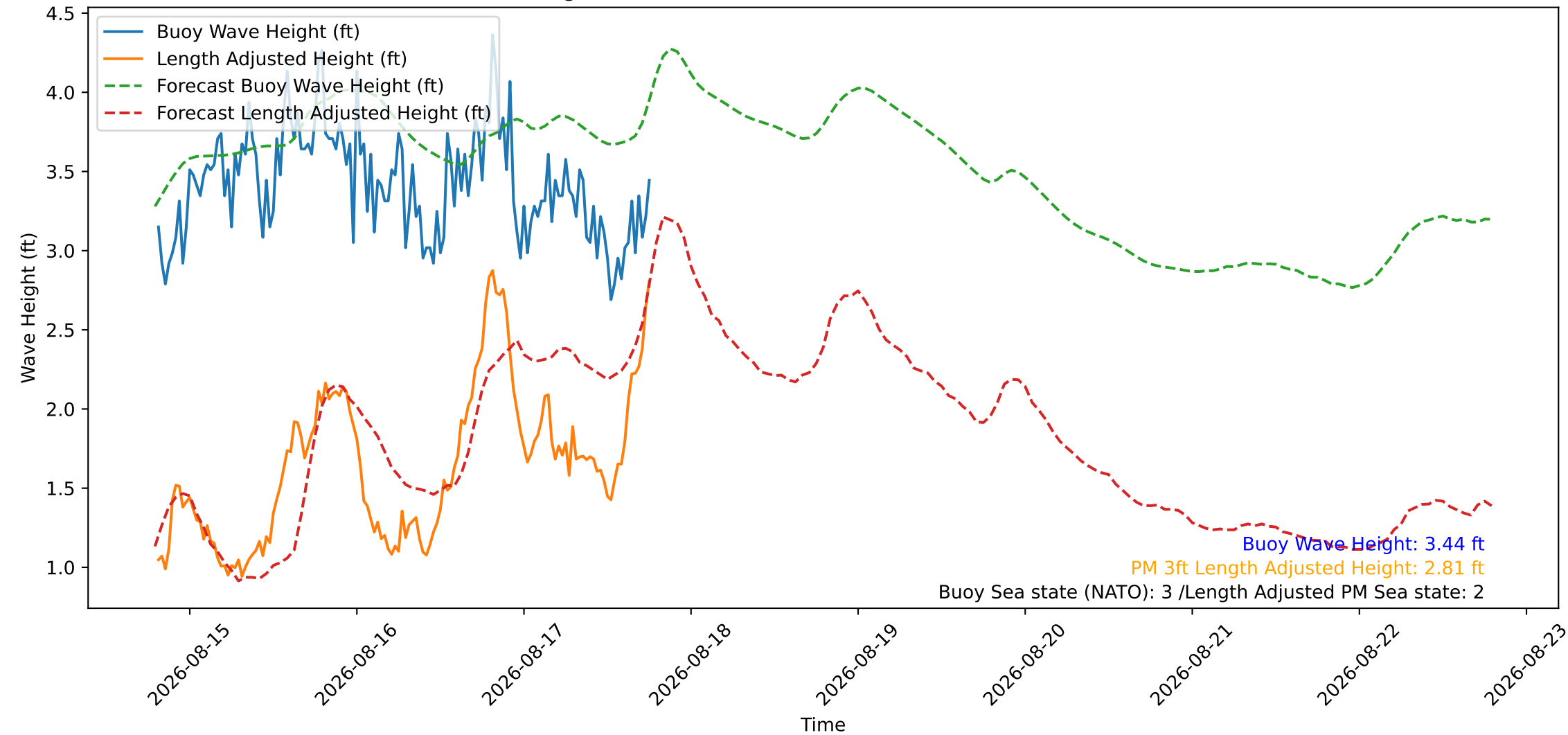
Wave Heights over Time for Green Beach at 2026-08-17 19:01:09
