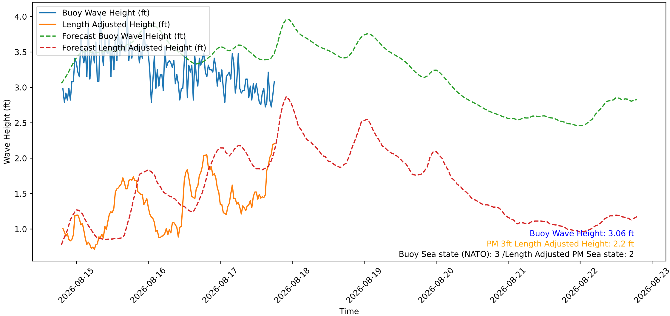
Wave Heights over Time for Red Beach at 2026-08-17 19:00:46
