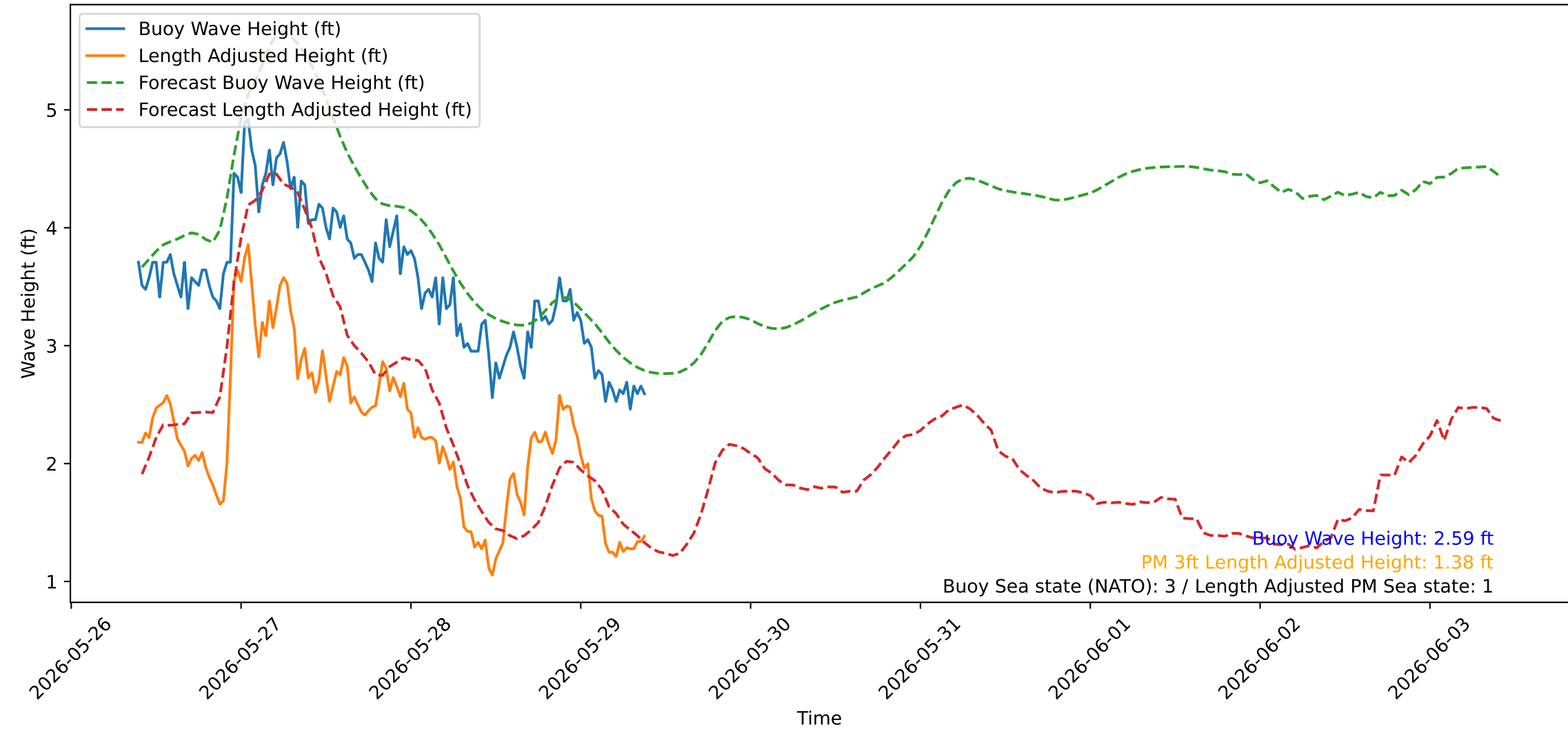
Wave Heights over Time for Green Beach at 2026-05-29 09:41:04
