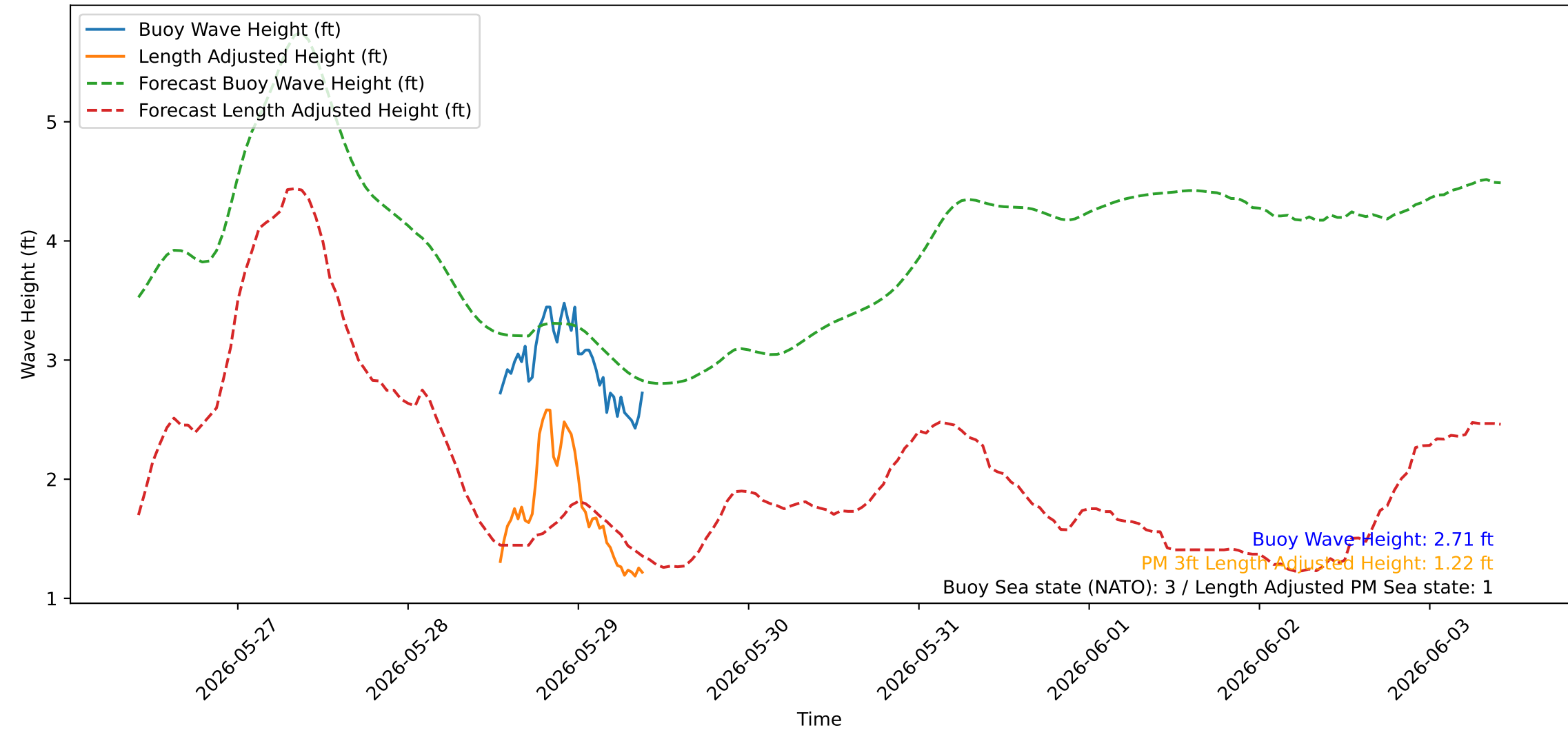
Wave Heights over Time for Oceanside Harbor at 2026-05-29 09:40:21
