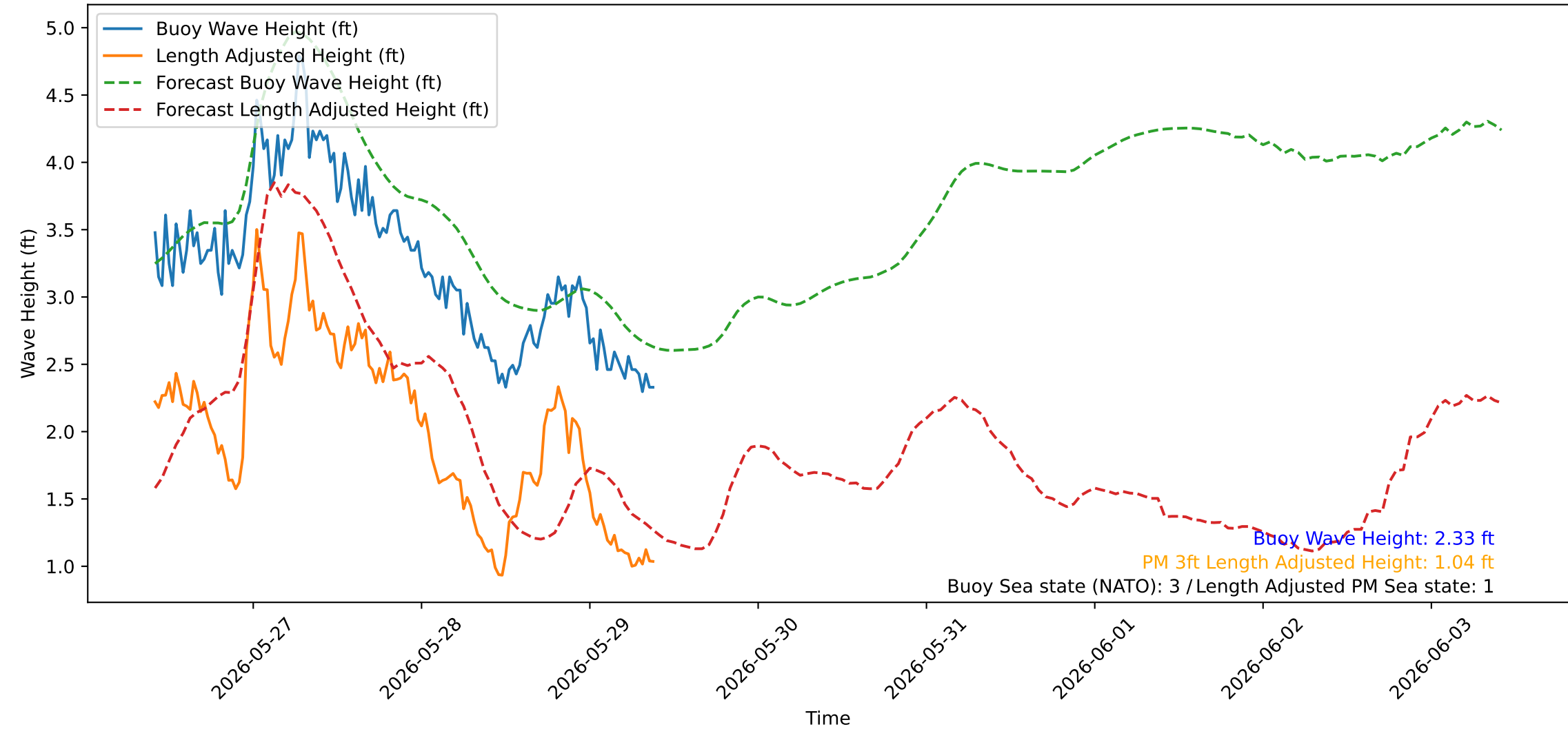
Wave Heights over Time for Red Beach at 2026-05-29 09:40:41
