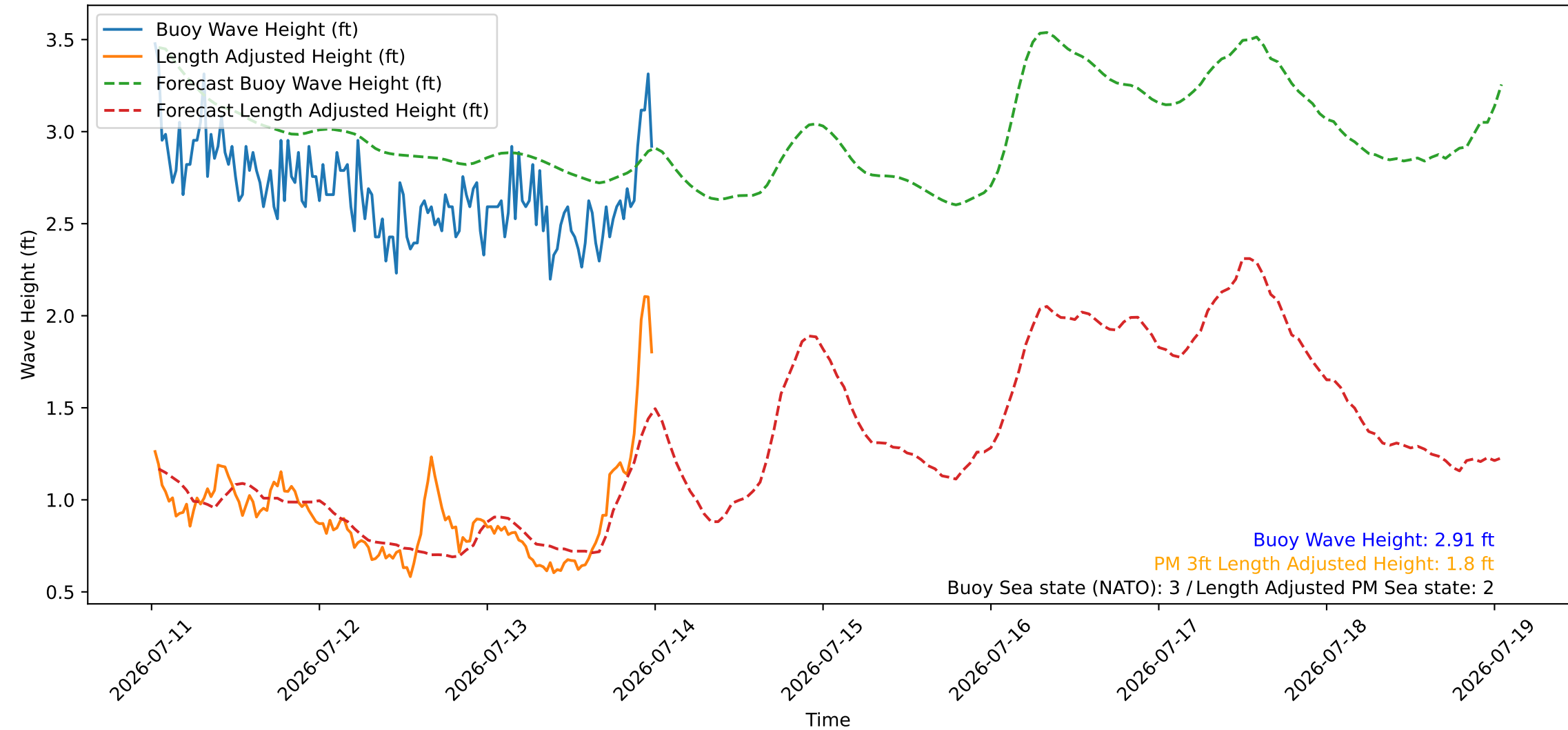
Wave Heights over Time for Green Beach at 2026-07-14 00:31:09
