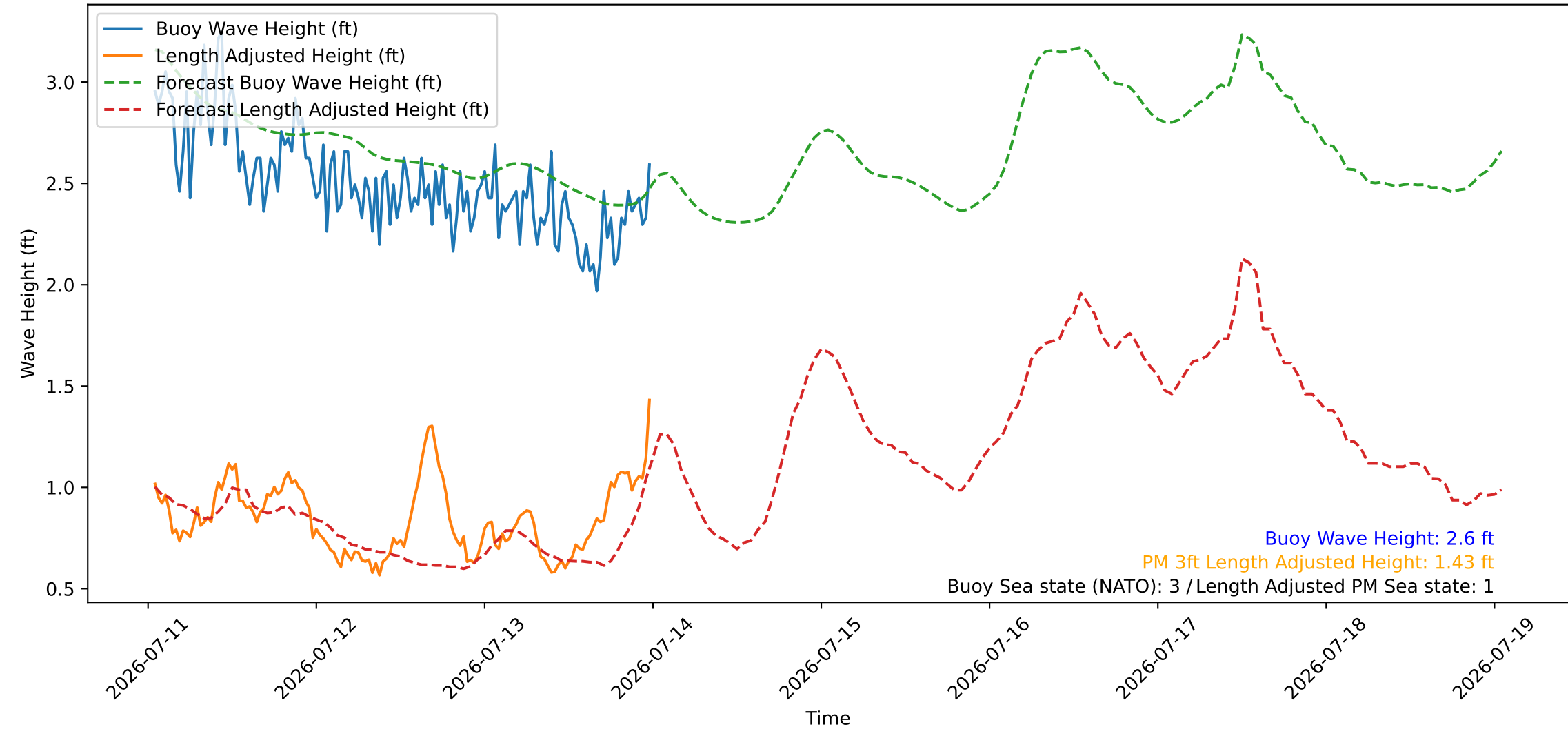
Wave Heights over Time for Red Beach at 2026-07-14 00:30:46
