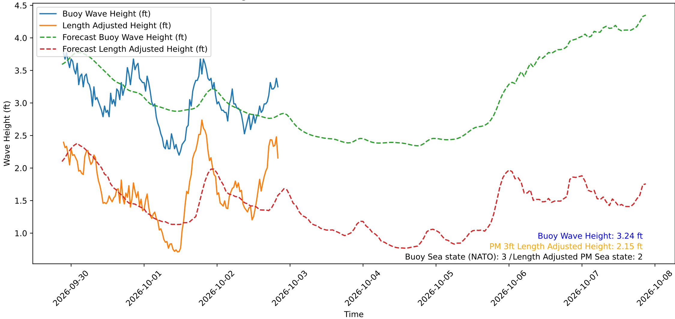
Wave Heights over Time for Green Beach at 2026-10-02 21:01:12
