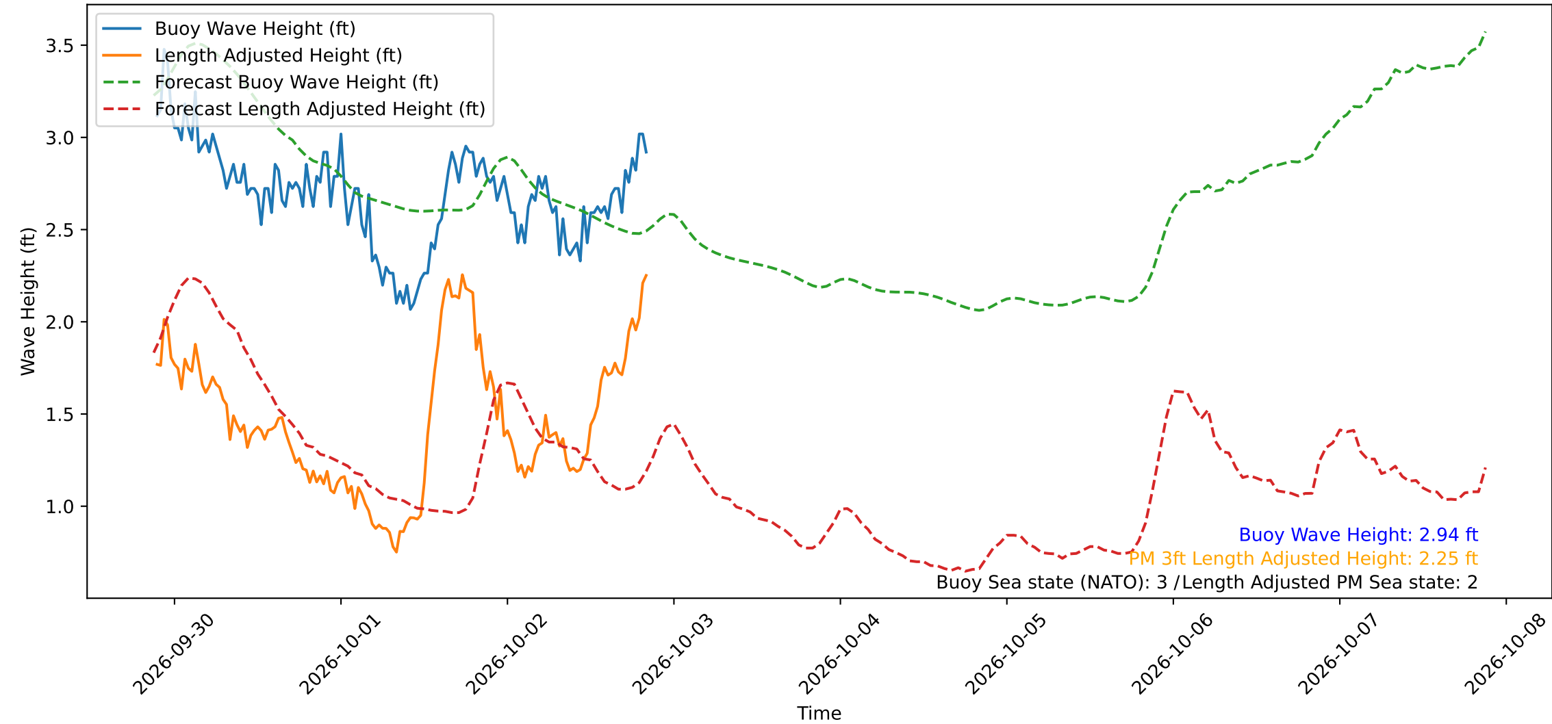
Wave Heights over Time for Red Beach at 2026-10-02 21:00:49
