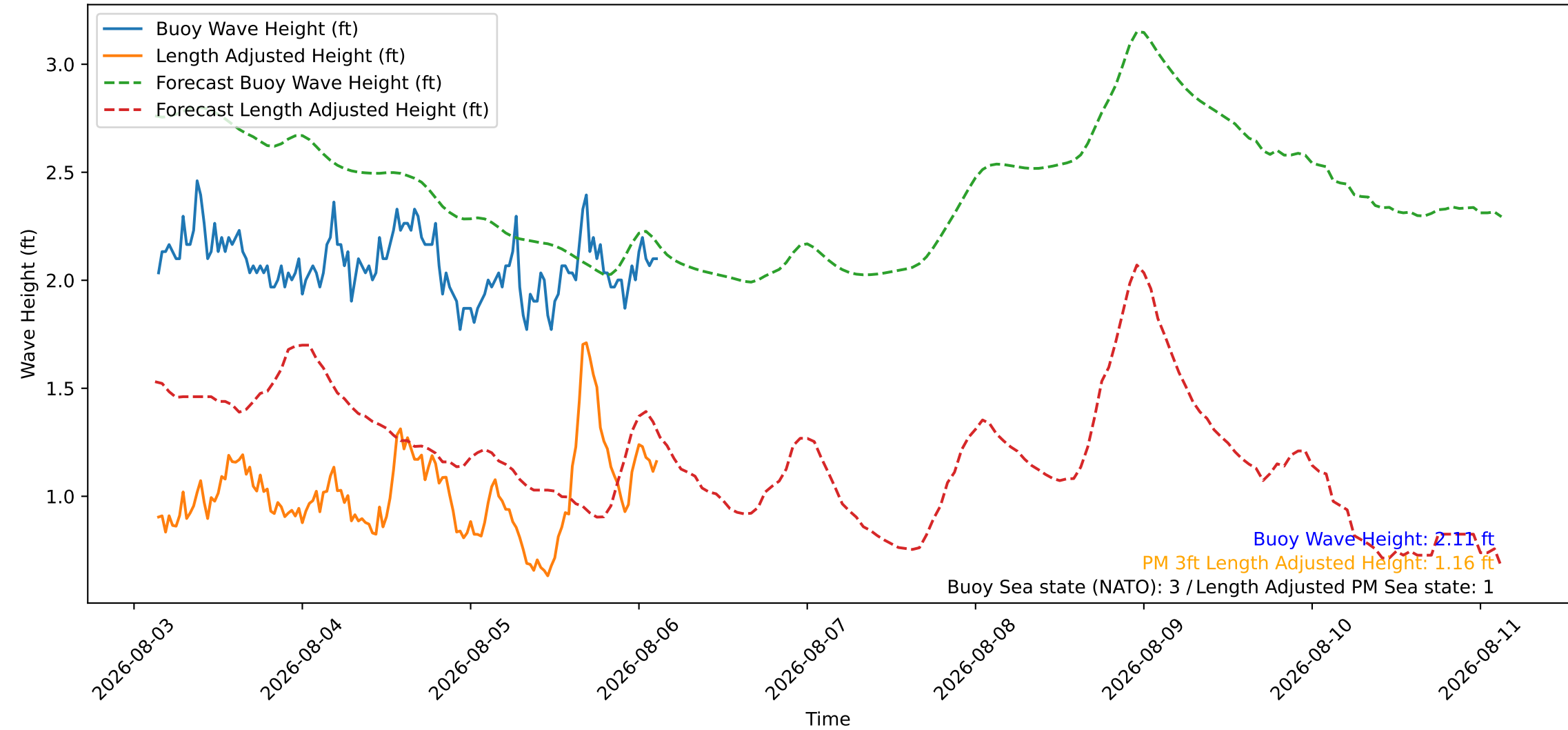
Wave Heights over Time for Red Beach at 2026-08-06 03:10:45
