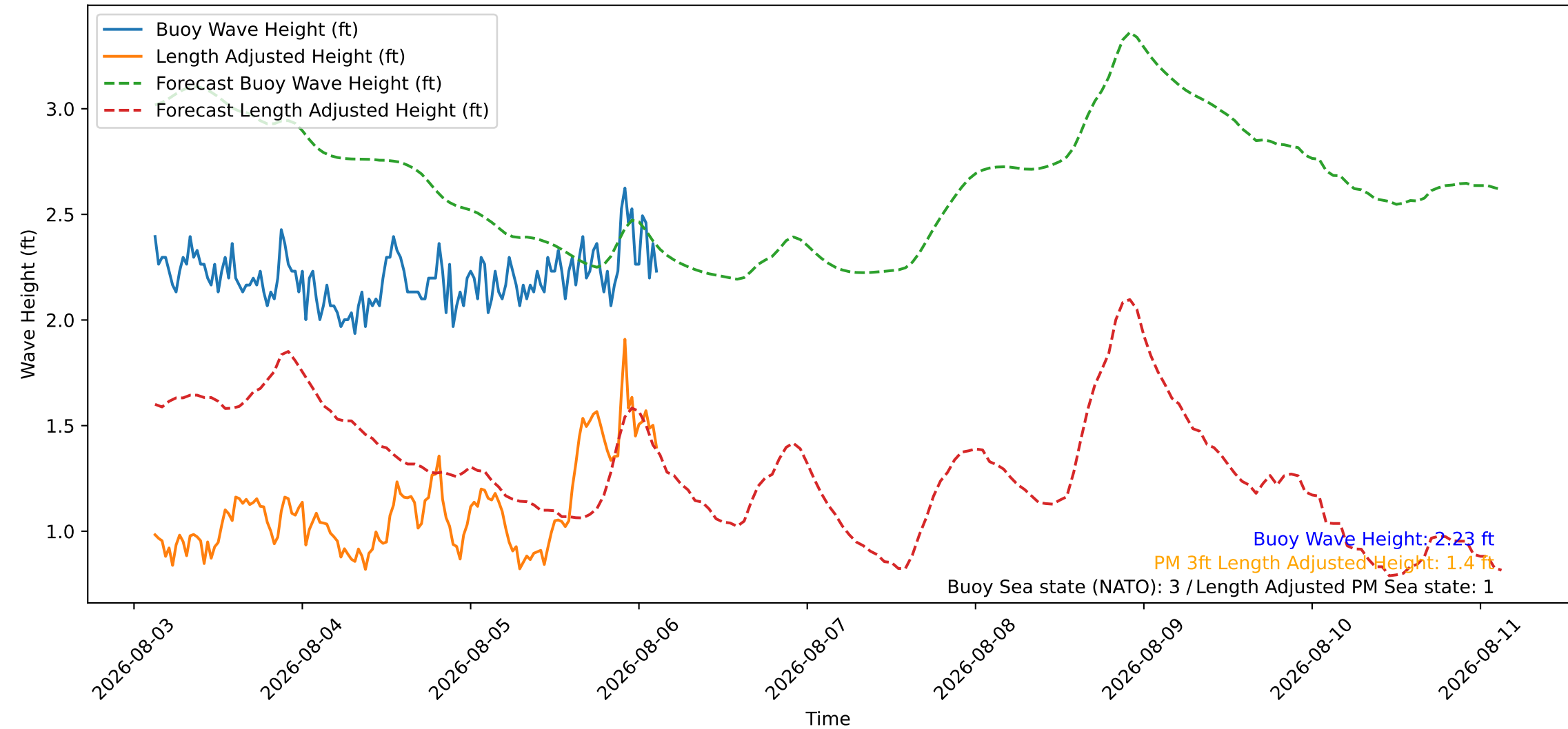
Wave Heights over Time for Green Beach at 2026-08-06 03:11:07
