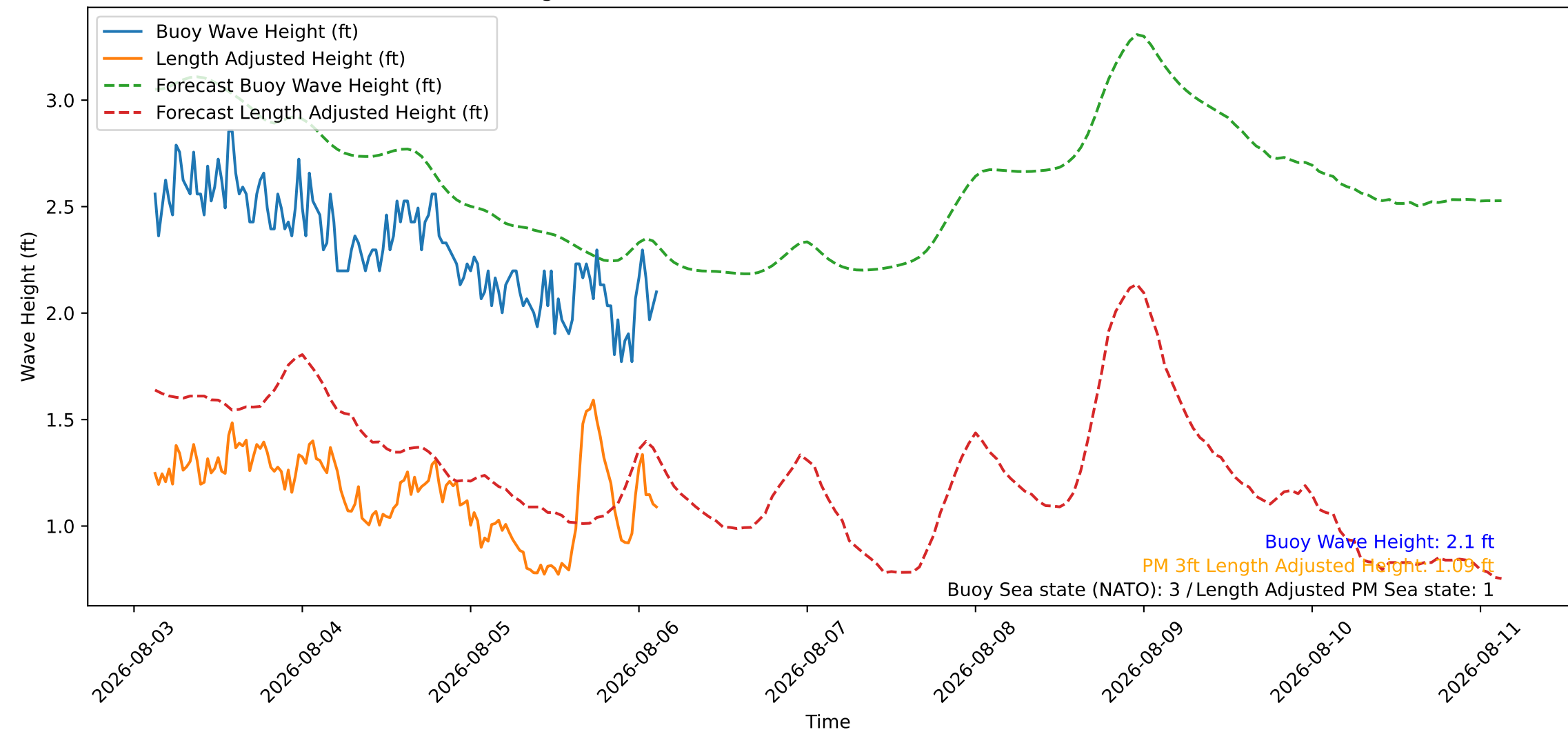
Wave Heights over Time for Oceanside Harbor at 2026-08-06 03:10:27
