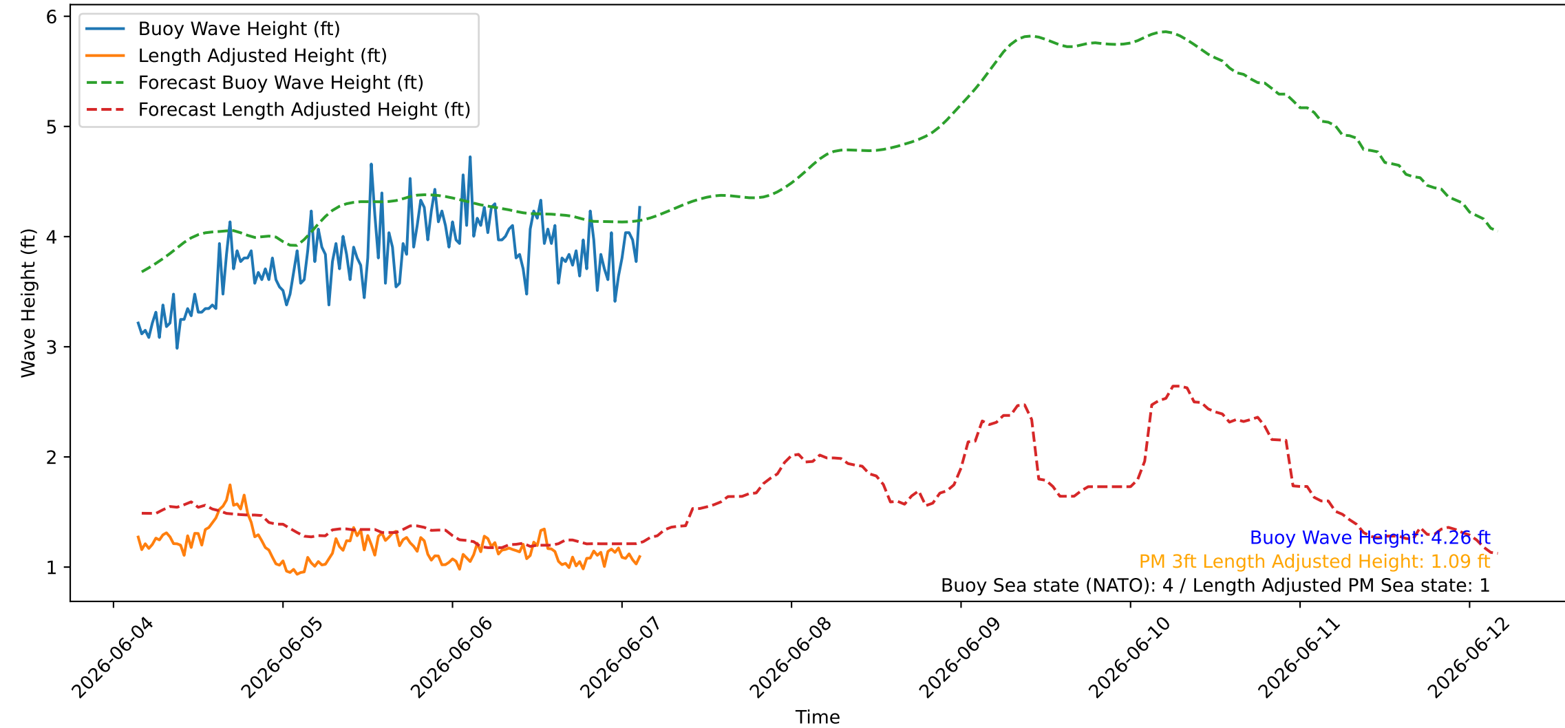
Wave Heights over Time for Green Beach at 2026-06-07 03:31:08
