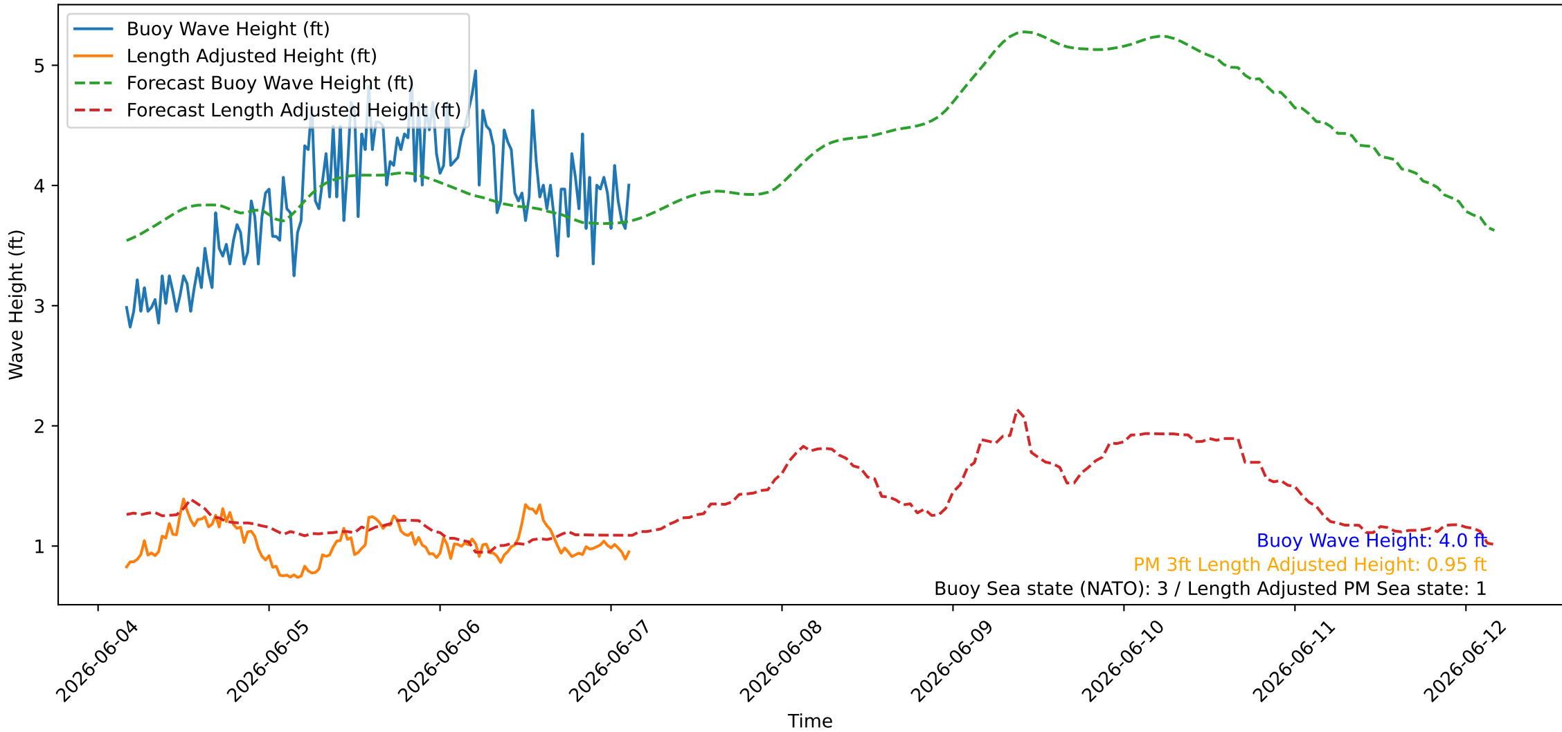
Wave Heights over Time for Red Beach at 2026-06-07 03:30:45
