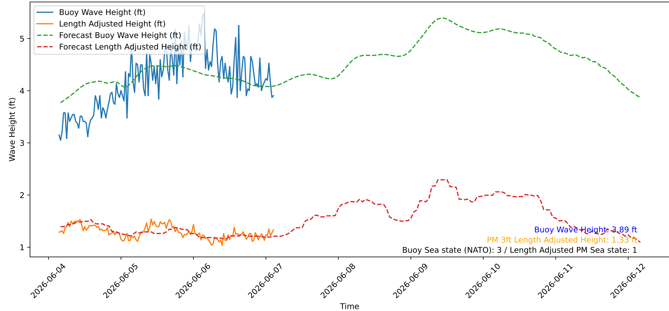
Wave Heights over Time for Oceanside Harbor at 2026-06-07 03:30:26
