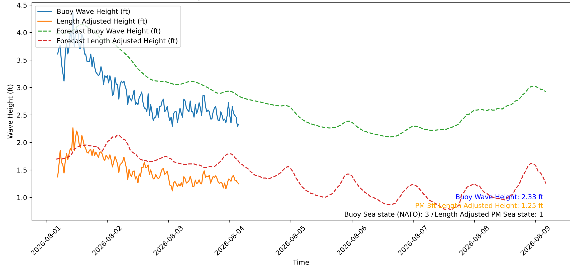
Wave Heights over Time for Oceanside Harbor at 2026-08-04 04:20:26
