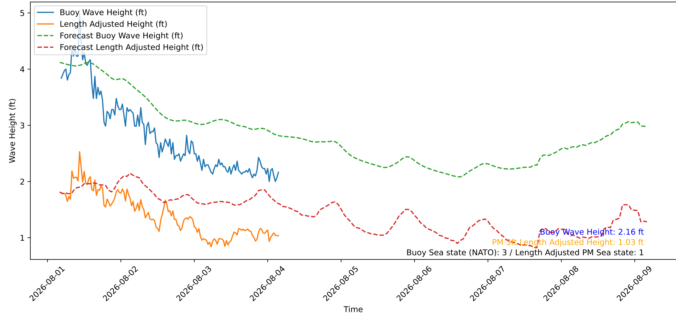
Wave Heights over Time for Green Beach at 2026-08-04 04:21:09
