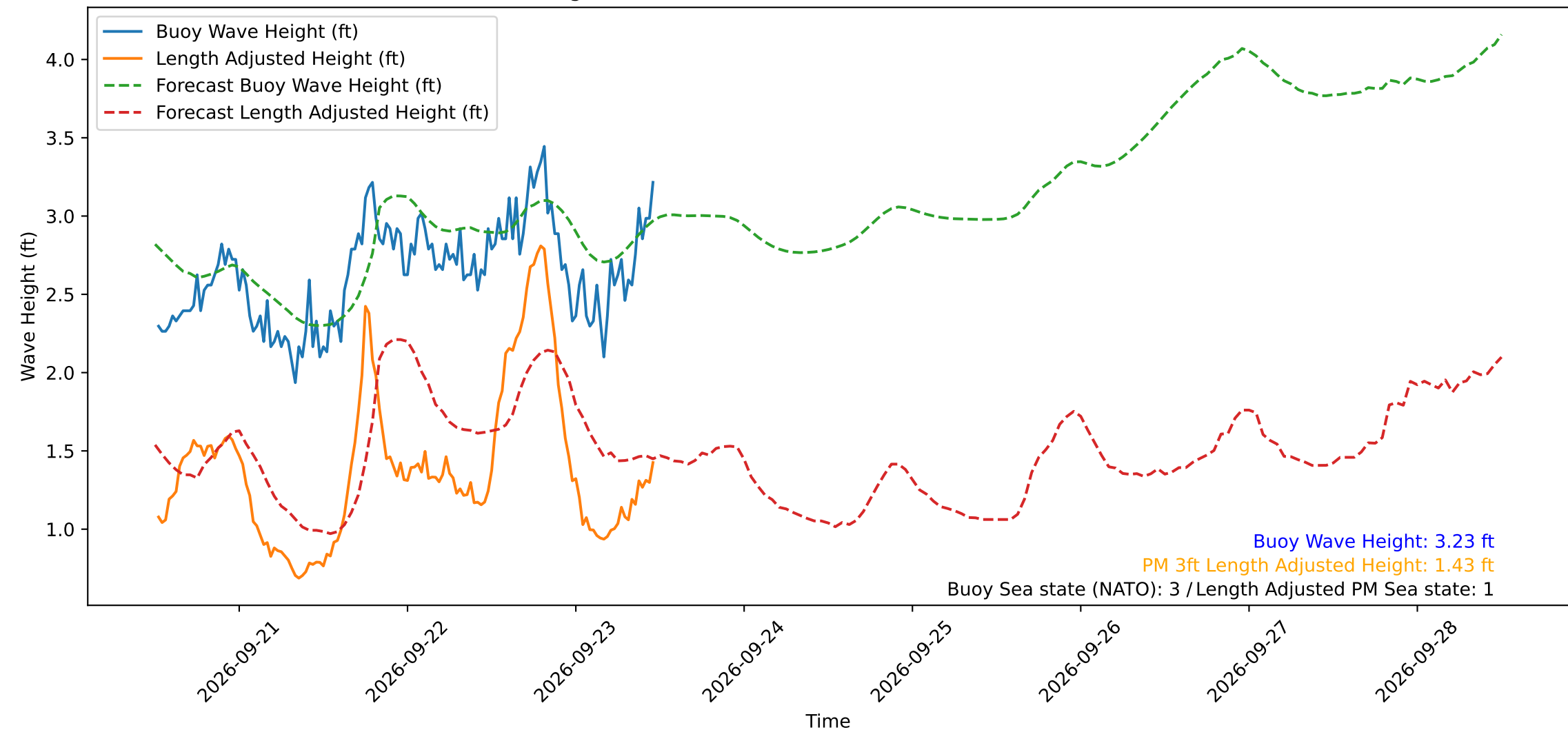
Wave Heights over Time for Green Beach at 2026-09-23 12:01:11
