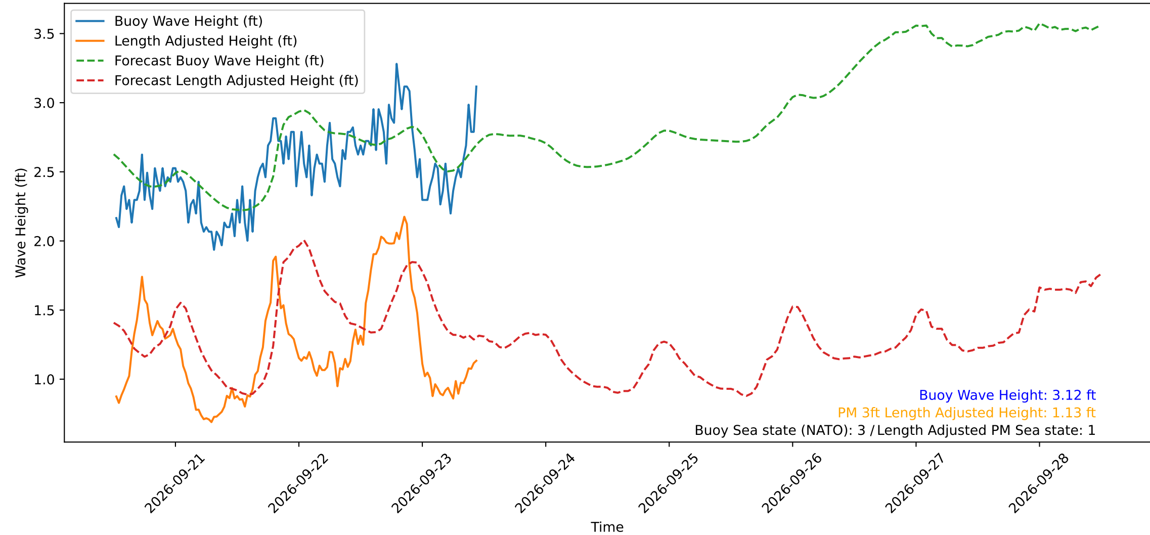
Wave Heights over Time for Red Beach at 2026-09-23 12:00:49
