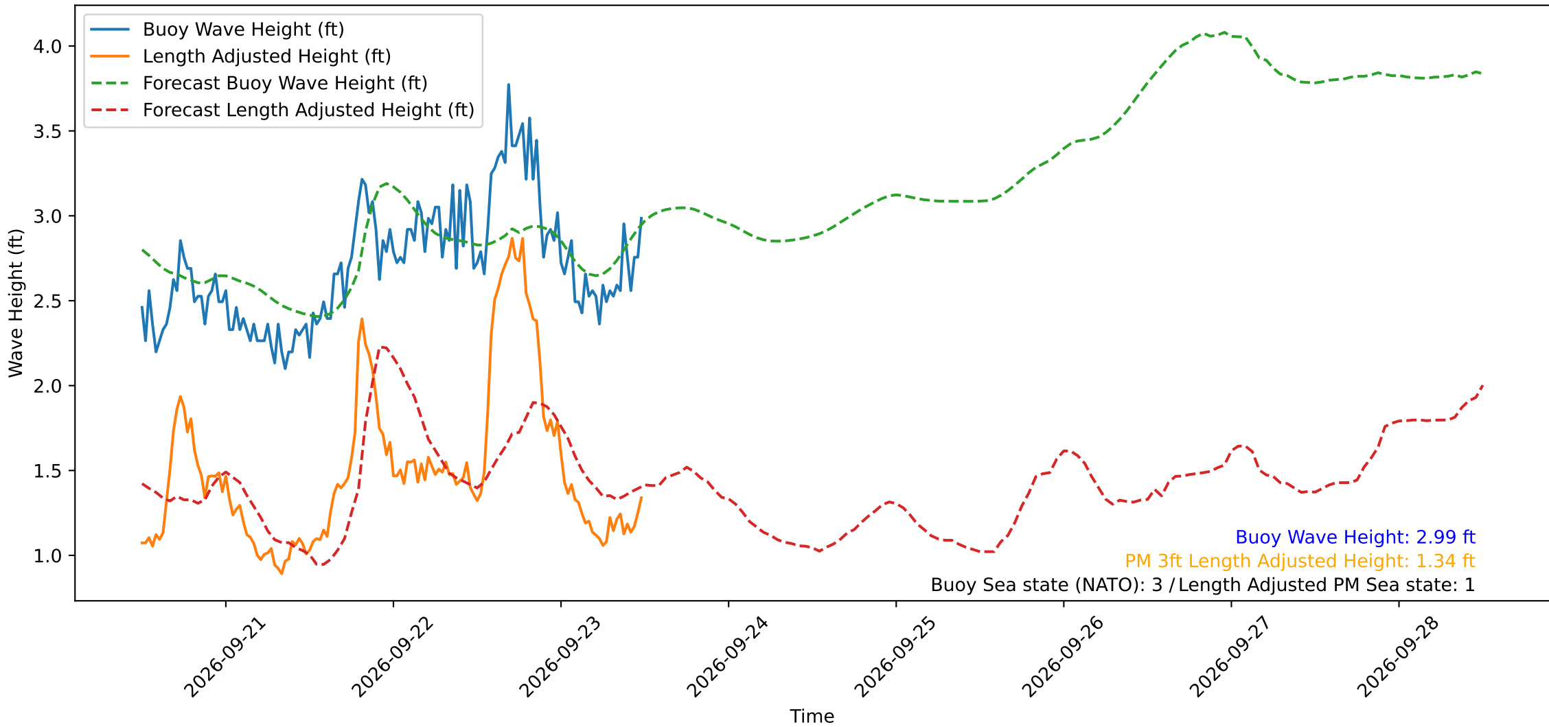
Wave Heights over Time for Oceanside Harbor at 2026-09-23 12:00:29
