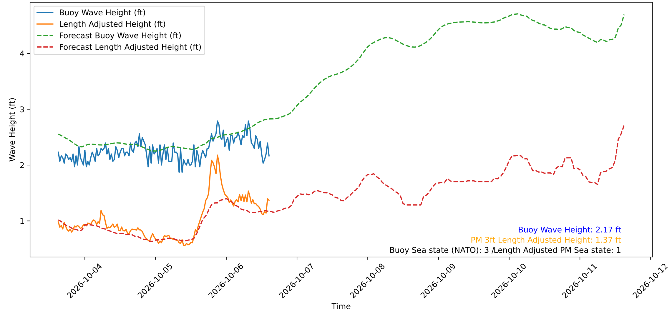
Wave Heights over Time for Oceanside Harbor at 2026-10-06 15:10:29
