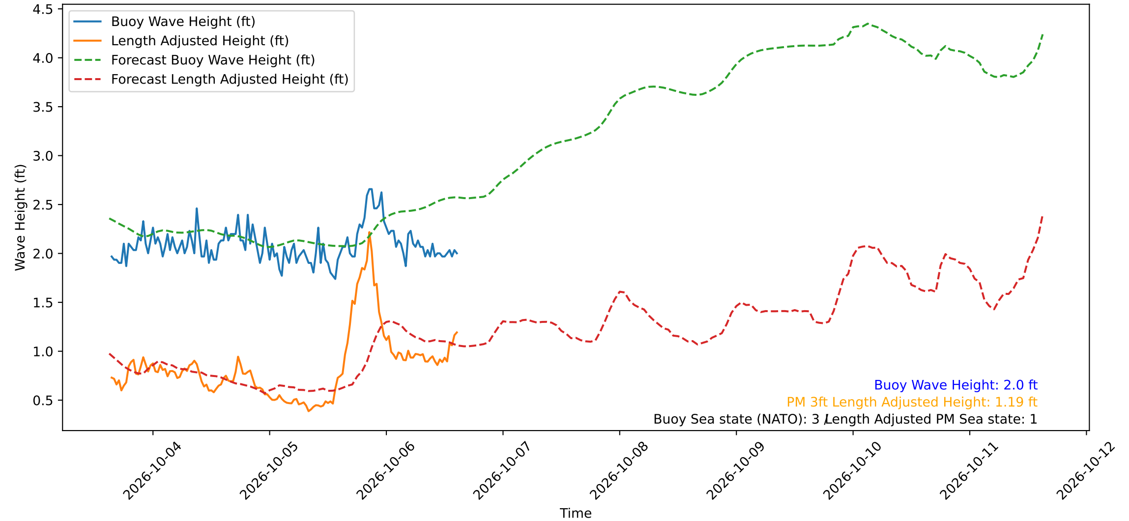
Wave Heights over Time for Red Beach at 2026-10-06 15:10:49
