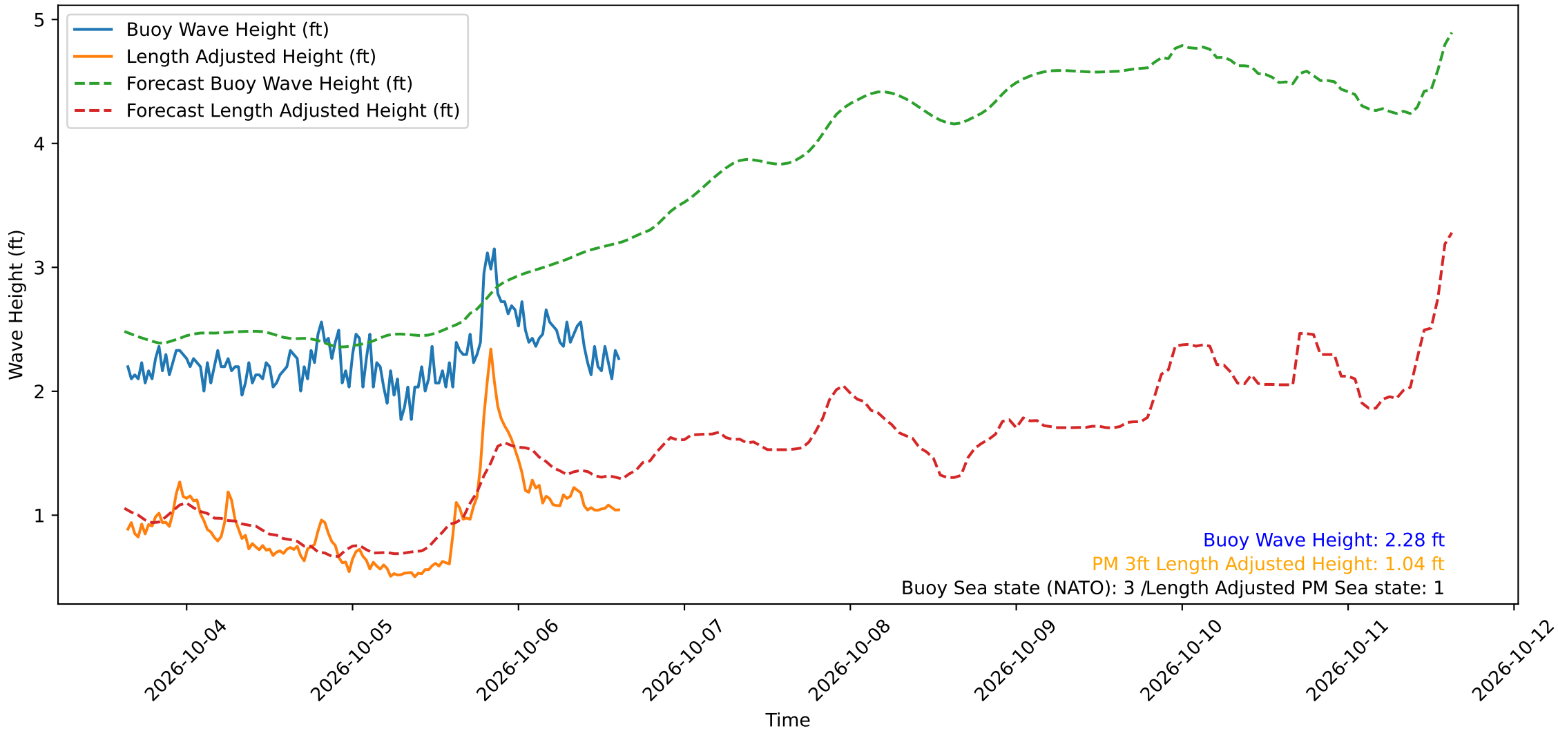
Wave Heights over Time for Green Beach at 2026-10-06 15:11:11
