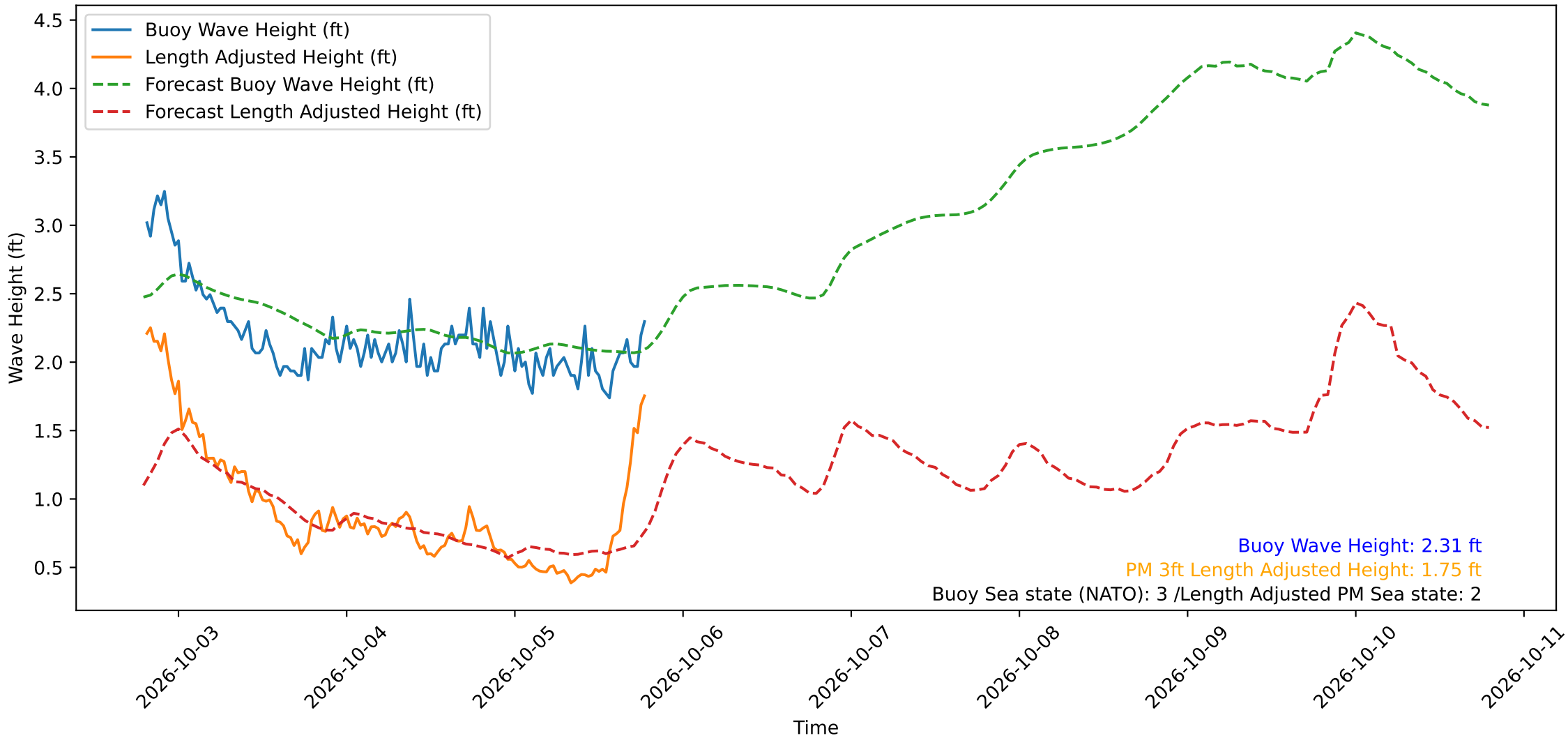
Wave Heights over Time for Red Beach at 2026-10-05 19:10:50
