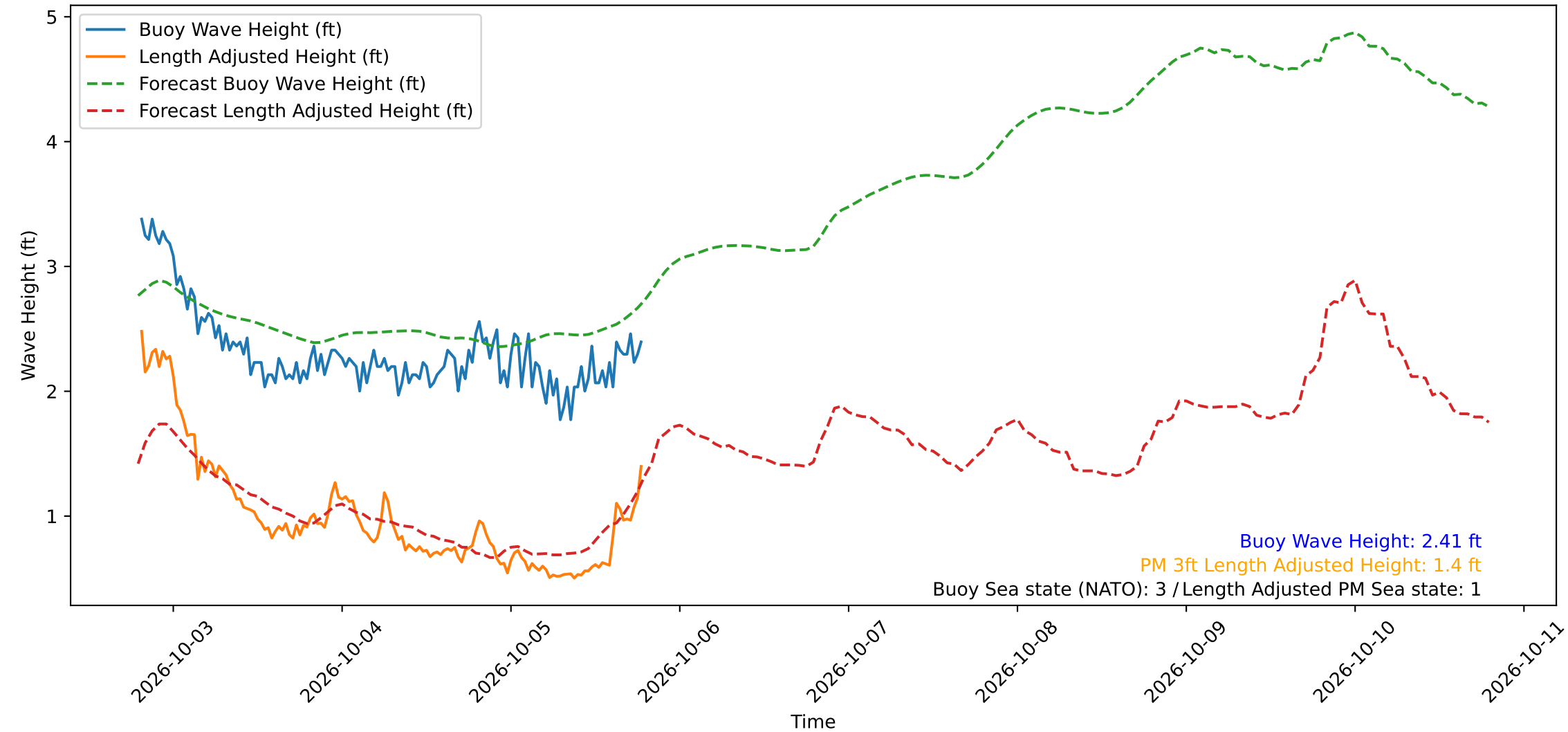
Wave Heights over Time for Green Beach at 2026-10-05 19:11:13
