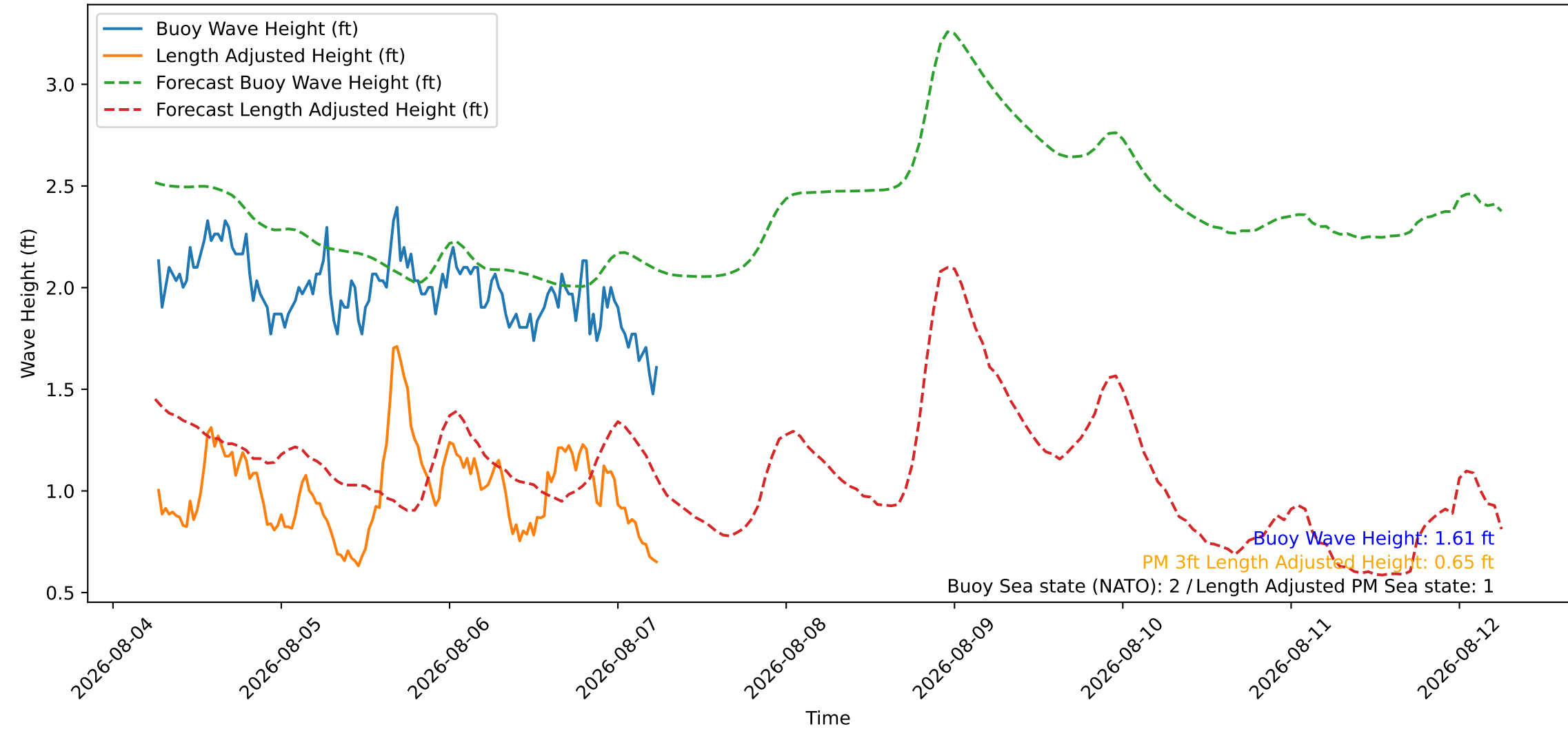
Wave Heights over Time for Red Beach at 2026-08-07 06:20:47
