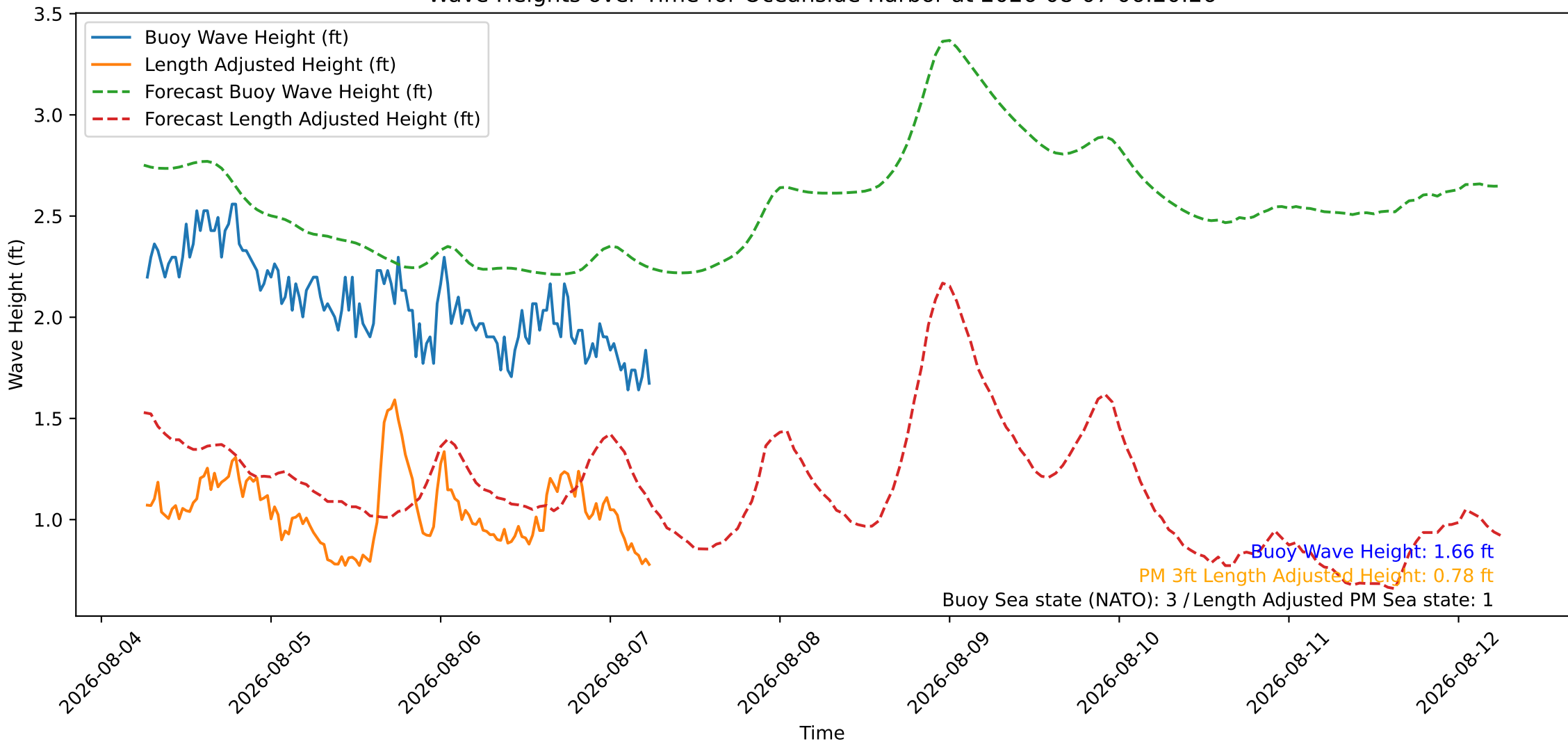
Wave Heights over Time for Oceanside Harbor at 2026-08-07 06:20:26
