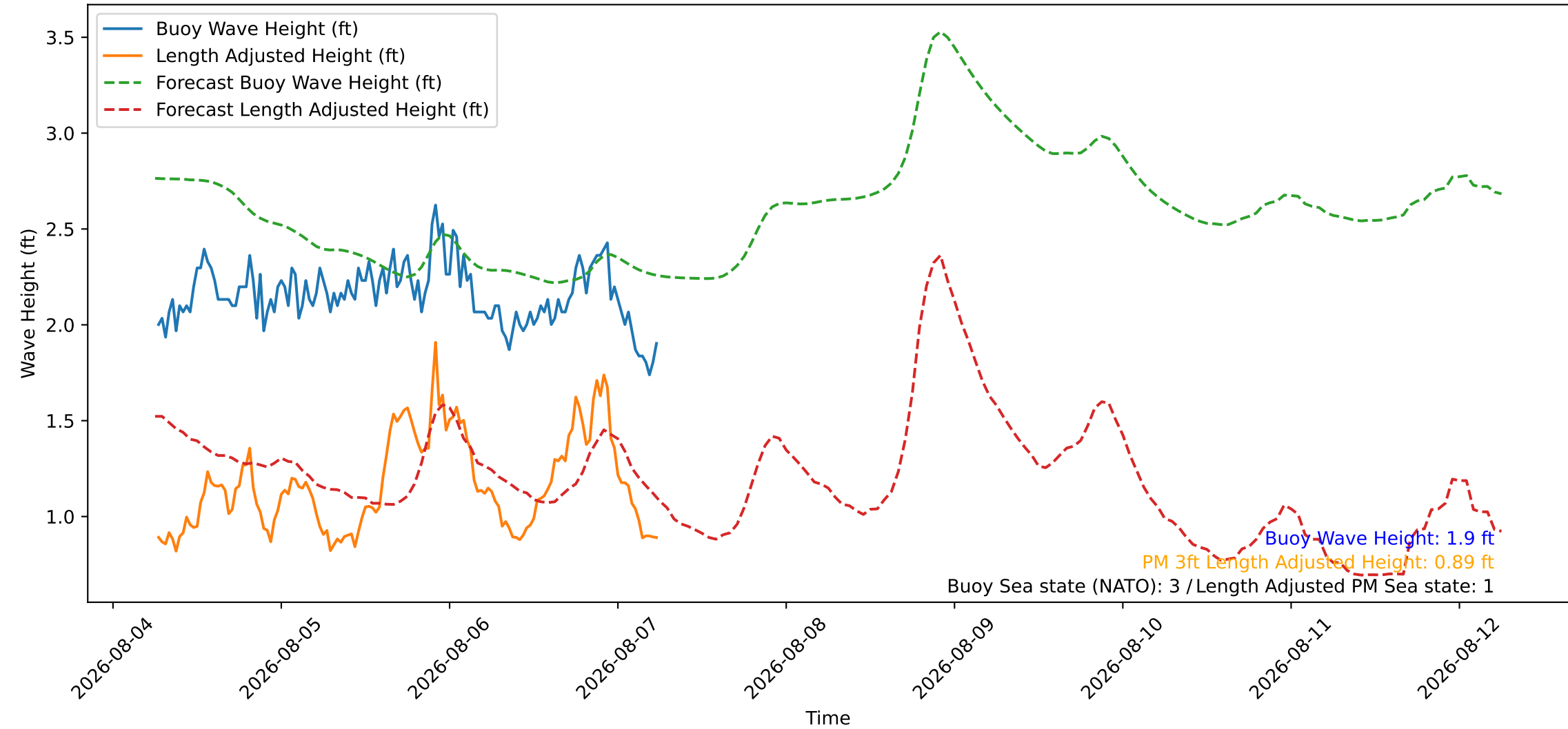
Wave Heights over Time for Green Beach at 2026-08-07 06:21:09
