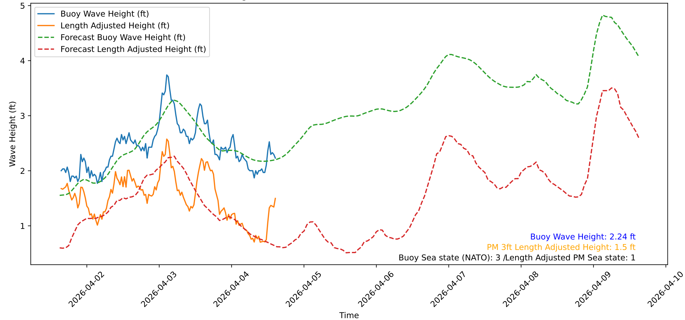
Wave Heights over Time for Red Beach at 2026-04-04 15:10:47
