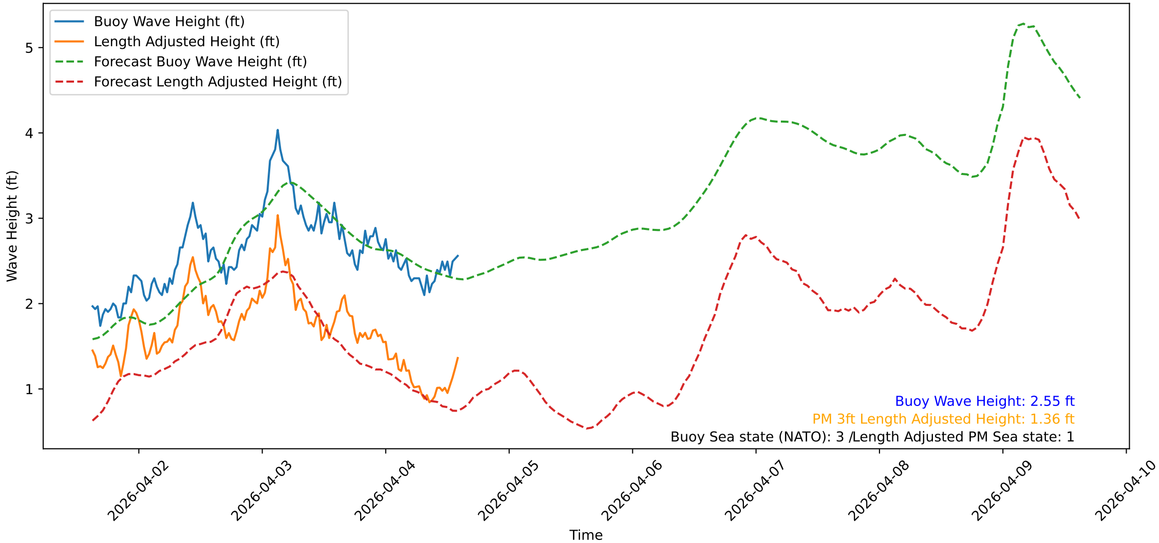
Wave Heights over Time for Oceanside Harbor at 2026-04-04 15:10:31
