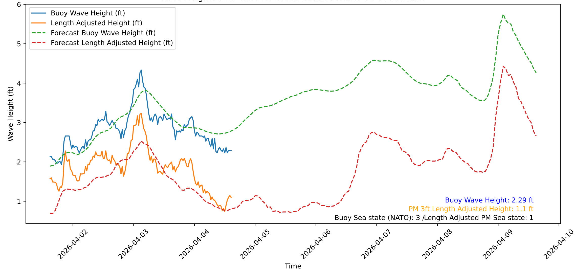
Wave Heights over Time for Green Beach at 2026-04-04 15:11:10
