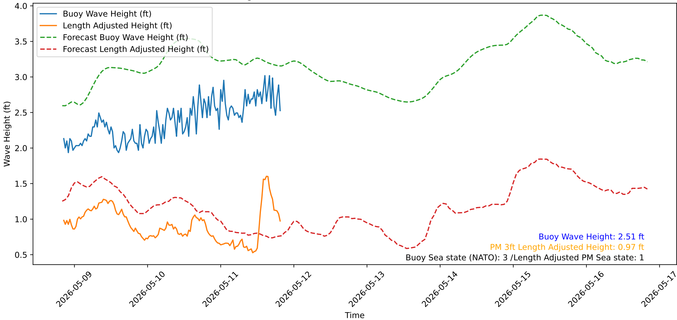
Wave Heights over Time for Red Beach at 2026-05-11 20:10:51
