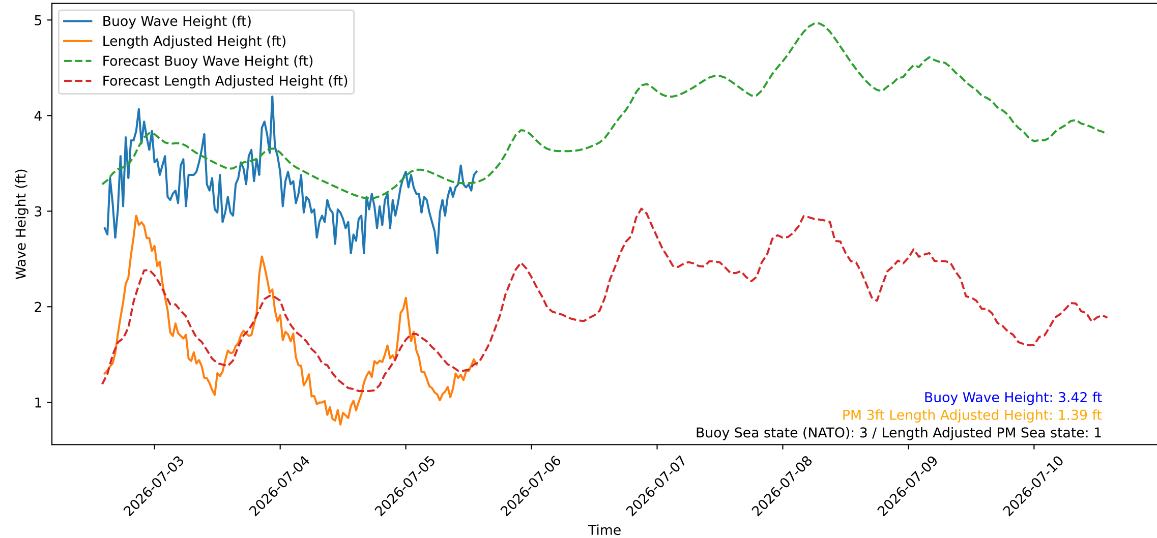
Wave Heights over Time for Green Beach at 2026-07-05 14:21:09
