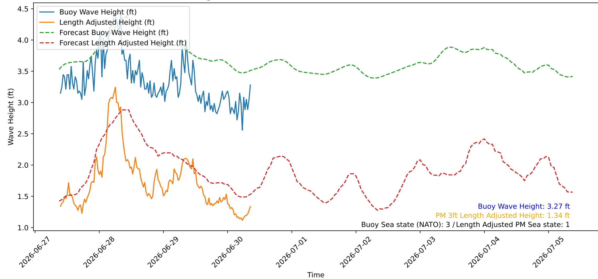
Wave Heights over Time for Oceanside Harbor at 2026-06-30 09:20:26
