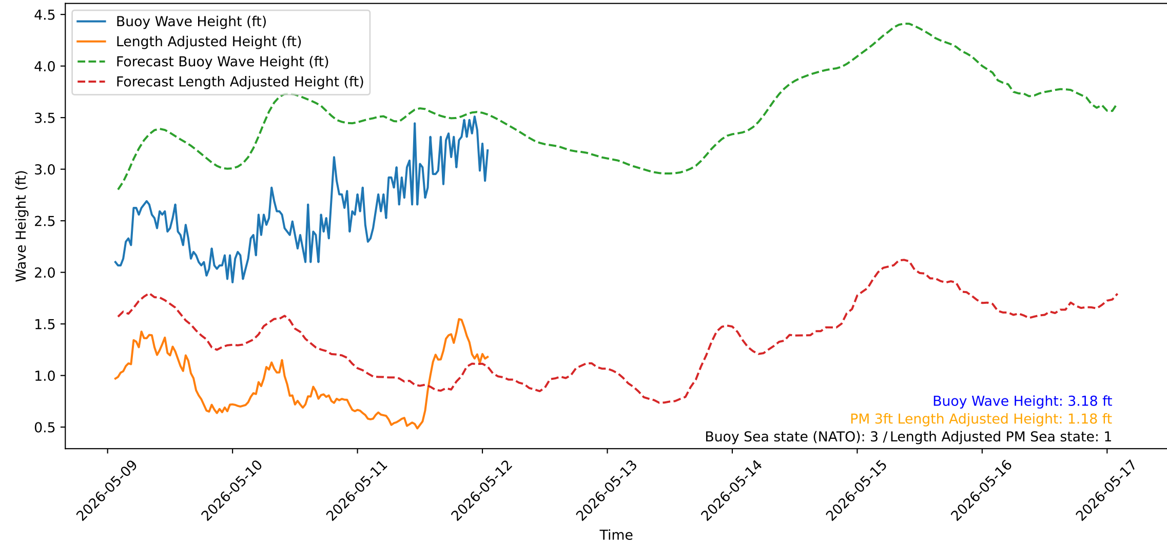
Wave Heights over Time for Green Beach at 2026-05-12 01:41:14
