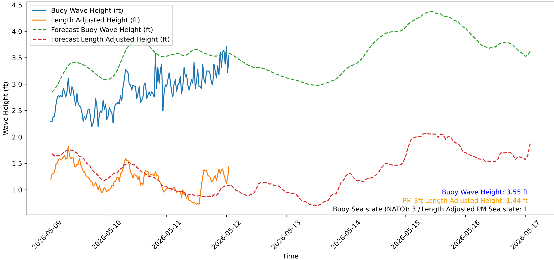
Wave Heights over Time for Oceanside Harbor at 2026-05-12 01:40:32
