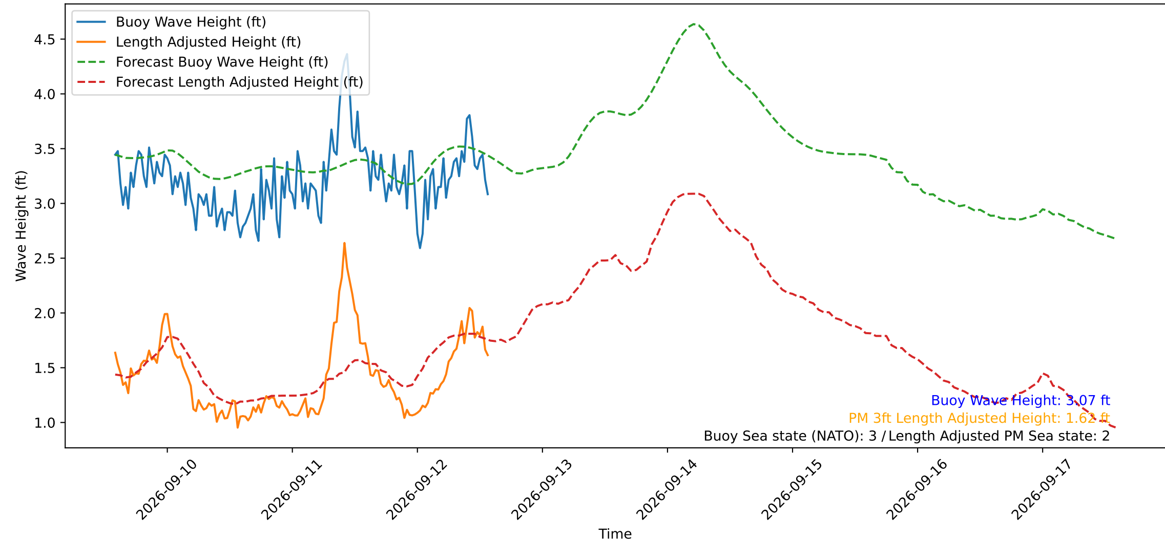
Wave Heights over Time for Oceanside Harbor at 2026-09-12 14:10:29
