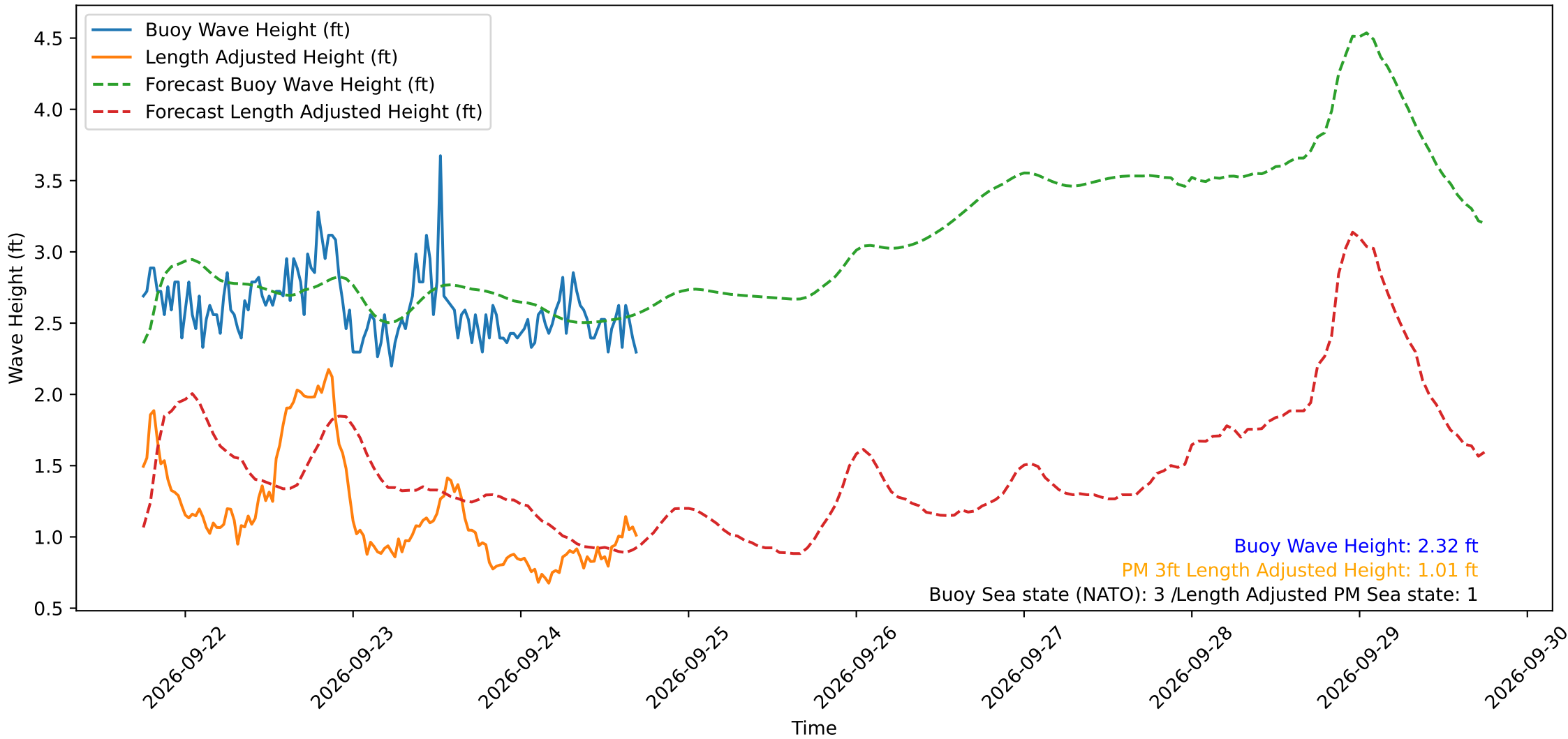
Wave Heights over Time for Red Beach at 2026-09-24 17:30:48
