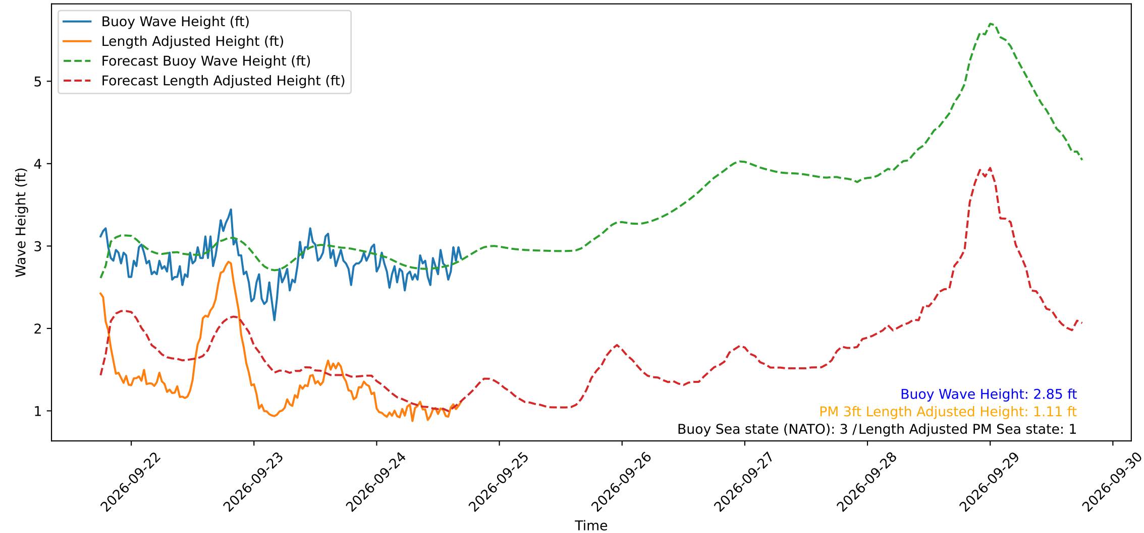
Wave Heights over Time for Green Beach at 2026-09-24 17:31:11
