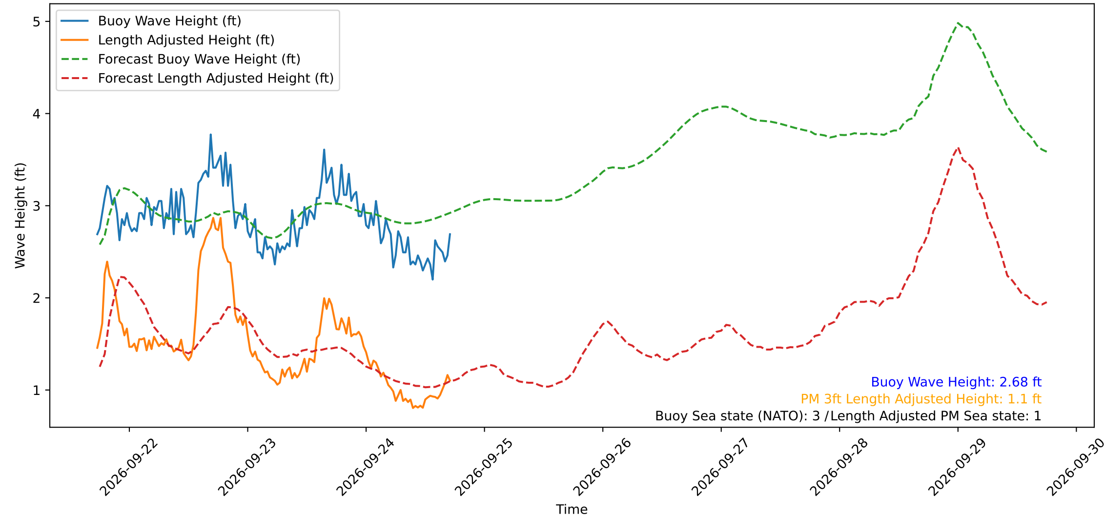
Wave Heights over Time for Oceanside Harbor at 2026-09-24 17:30:29
