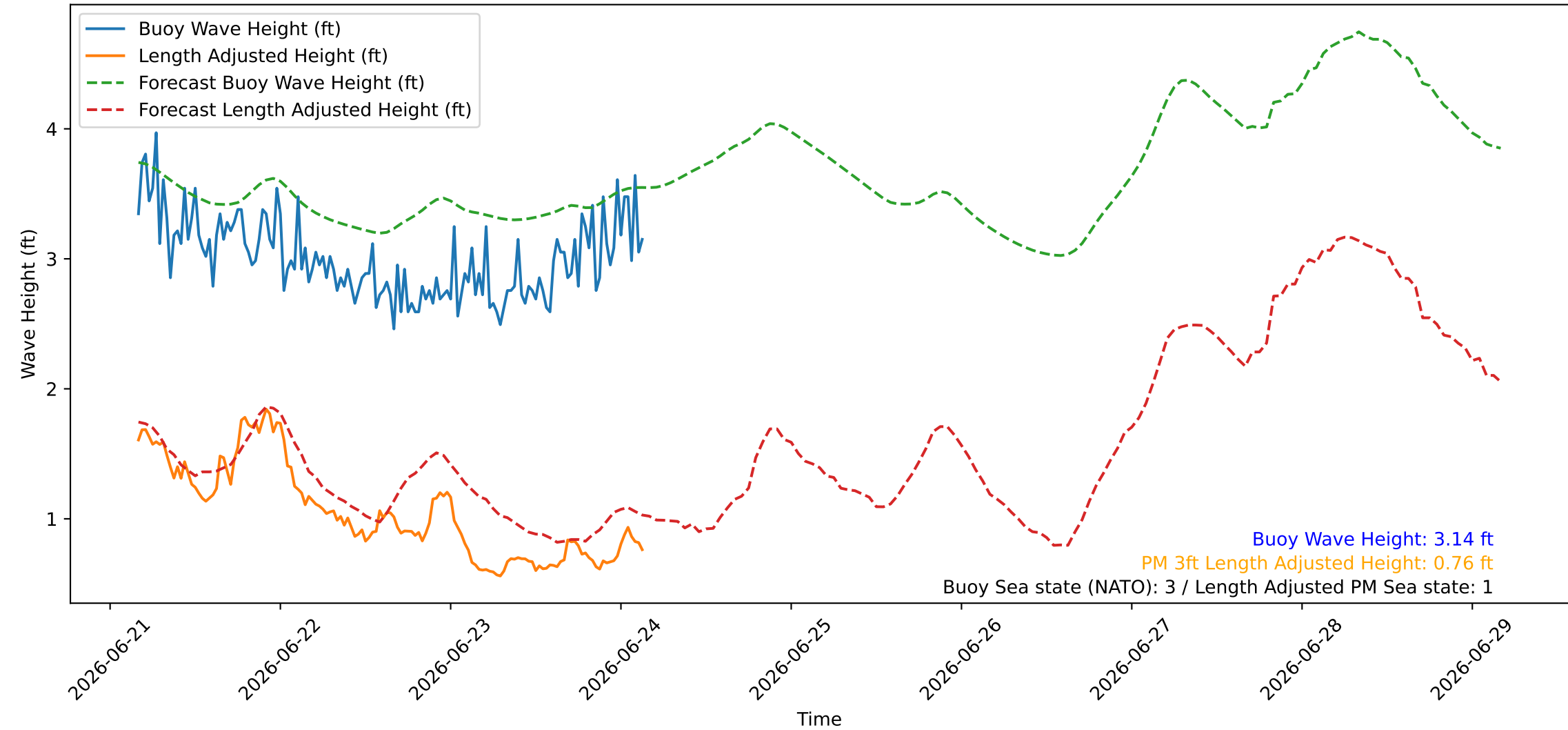
Wave Heights over Time for Green Beach at 2026-06-24 03:51:10
