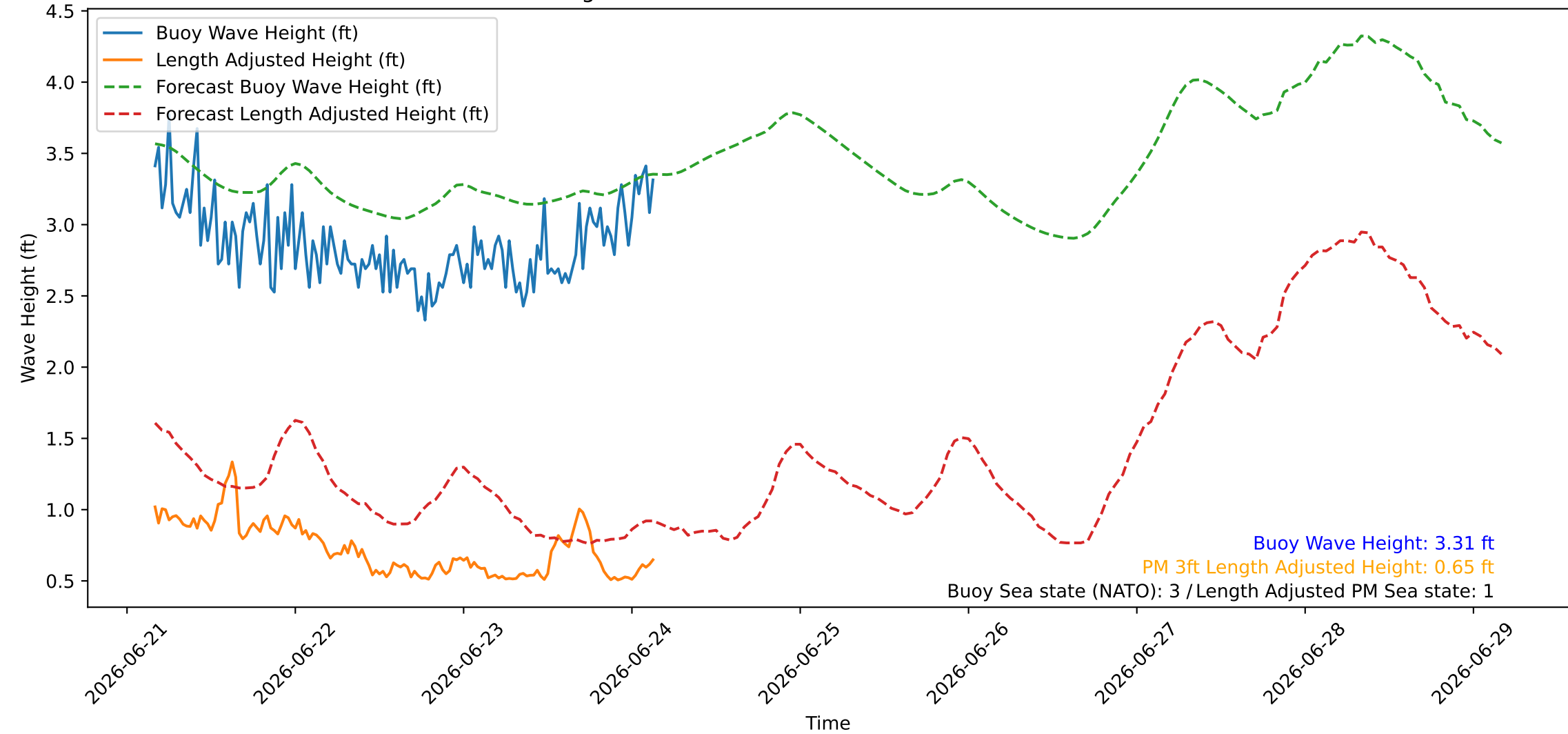
Wave Heights over Time for Red Beach at 2026-06-24 03:50:47
