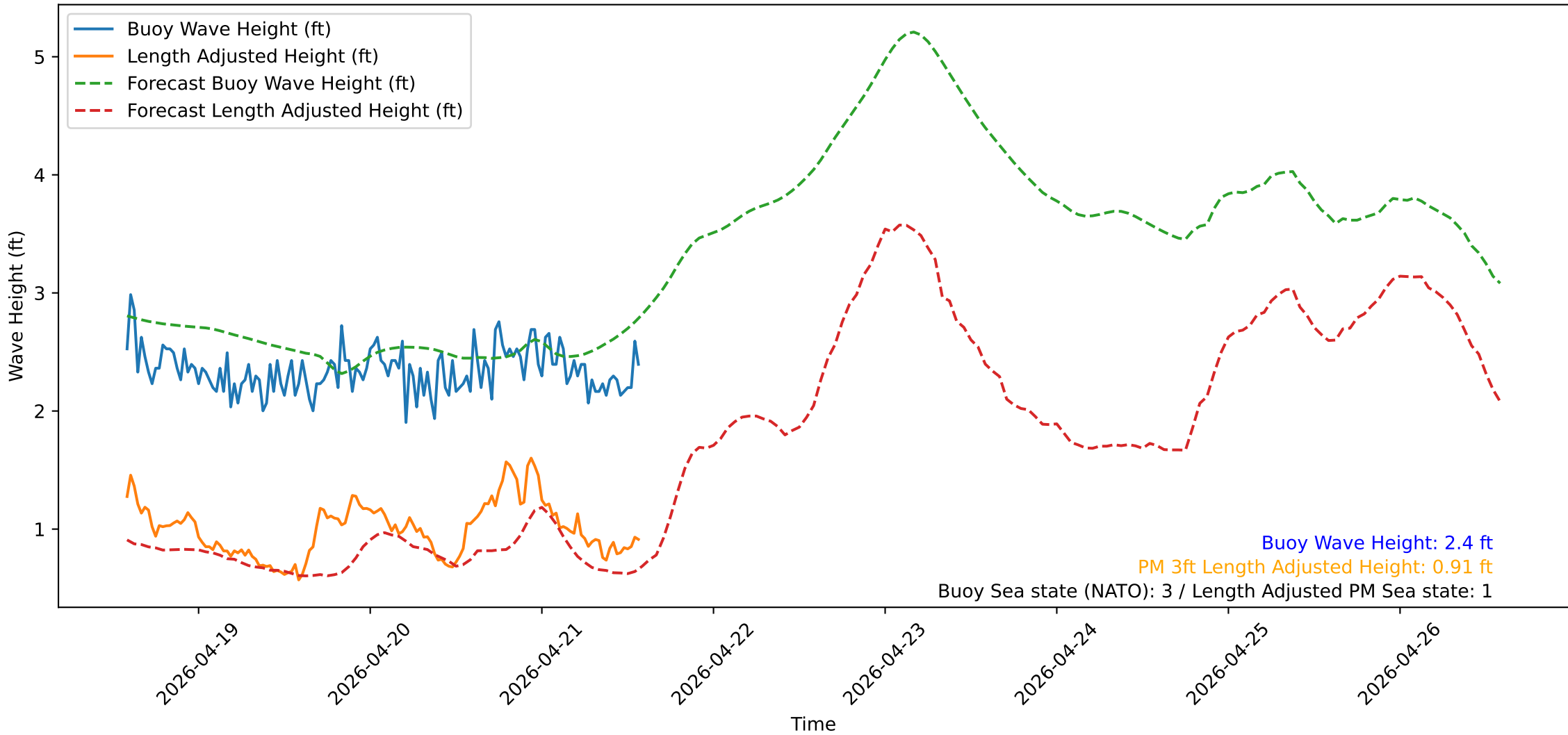
Wave Heights over Time for Oceanside Harbor at 2026-04-21 14:00:32
