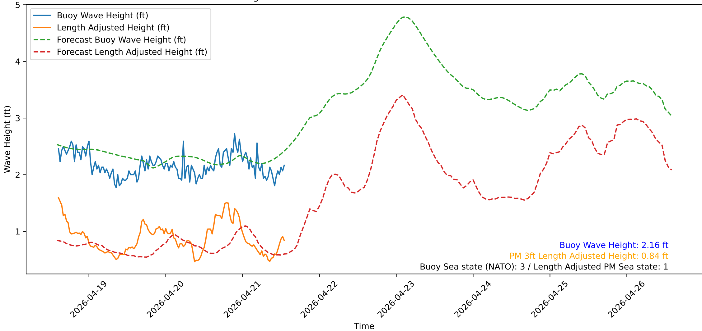
Wave Heights over Time for Red Beach at 2026-04-21 14:00:51
