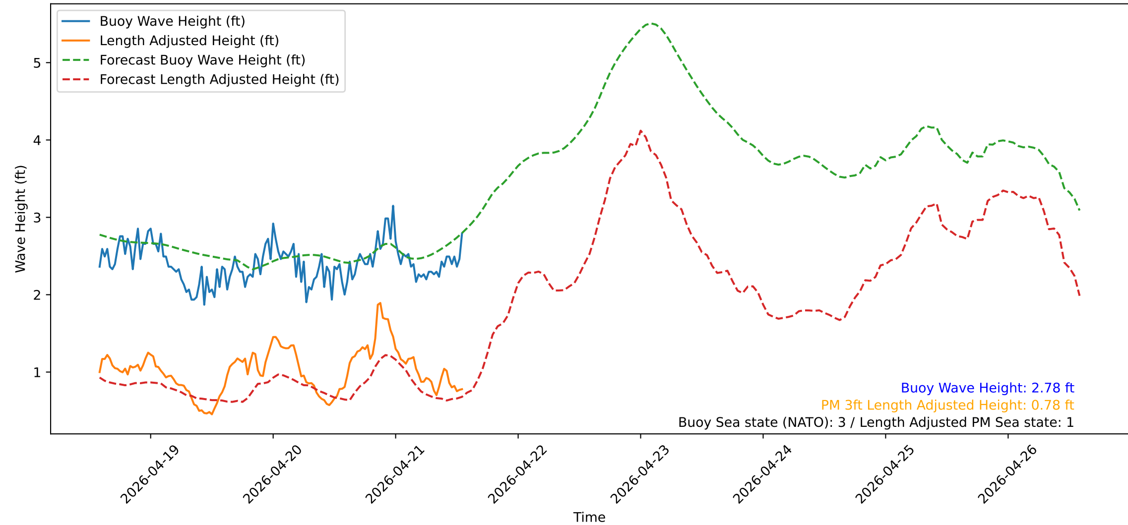
Wave Heights over Time for Green Beach at 2026-04-21 14:01:13
