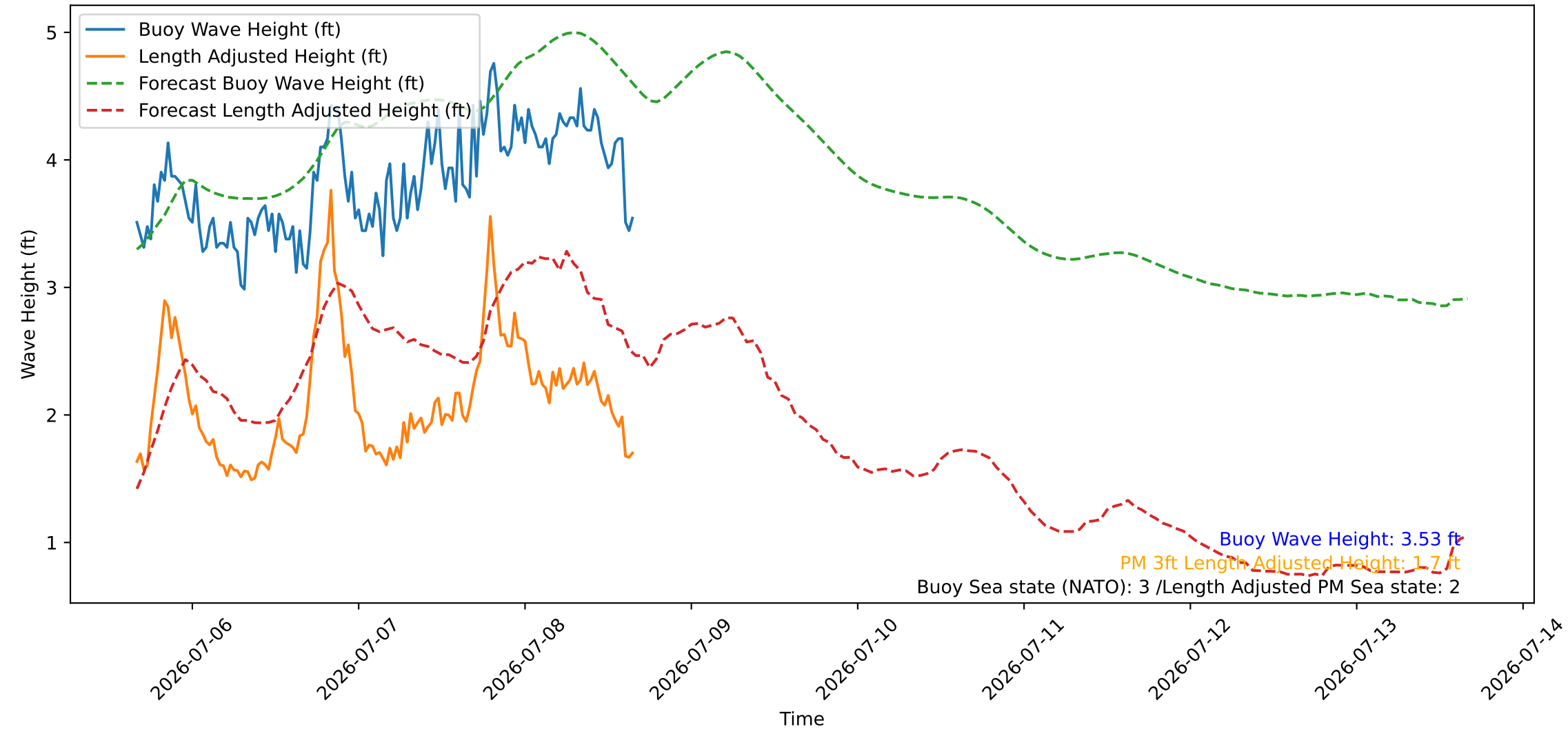
Wave Heights over Time for Green Beach at 2026-07-08 16:11:09
