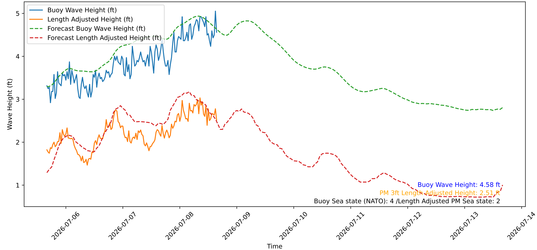
Wave Heights over Time for Oceanside Harbor at 2026-07-08 16:10:27
