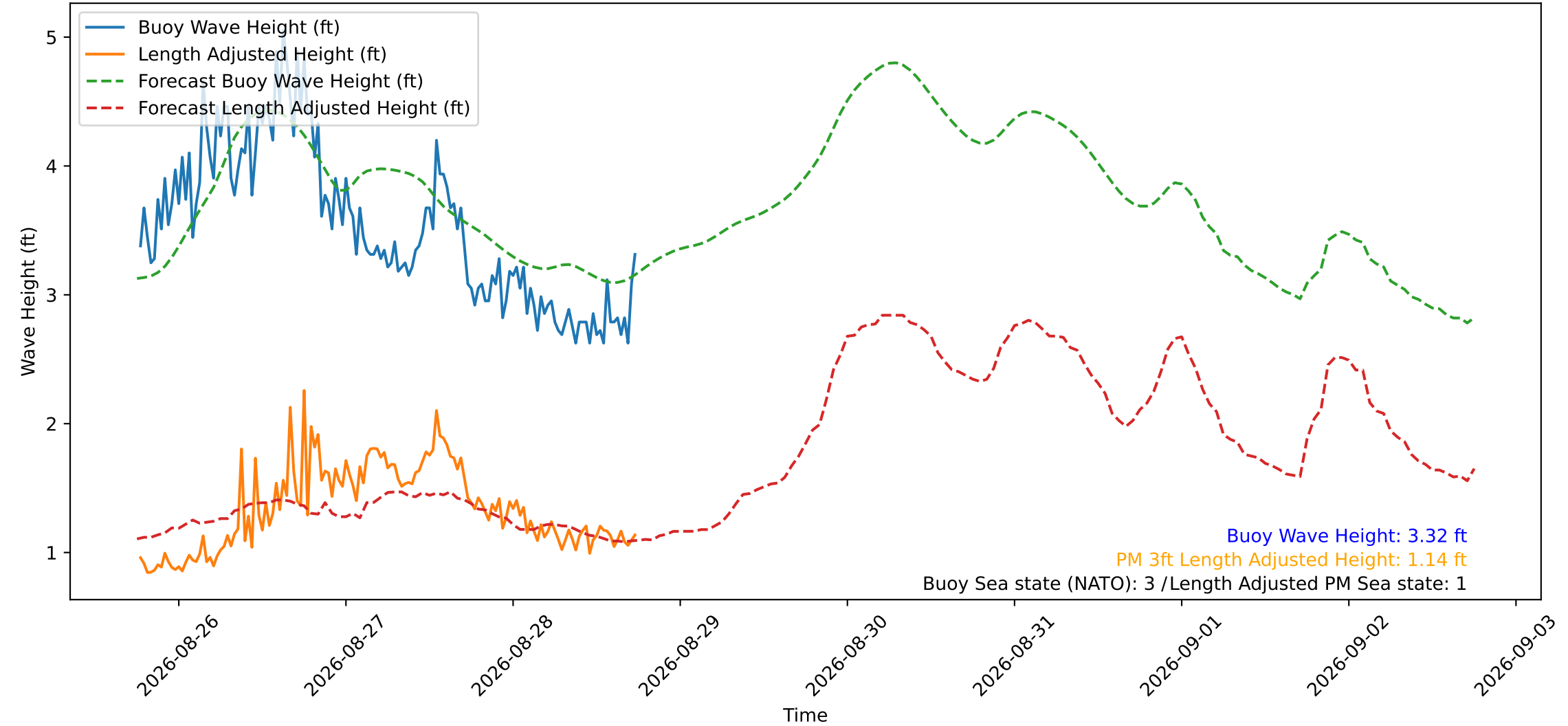
Wave Heights over Time for Red Beach at 2026-08-28 18:20:50
