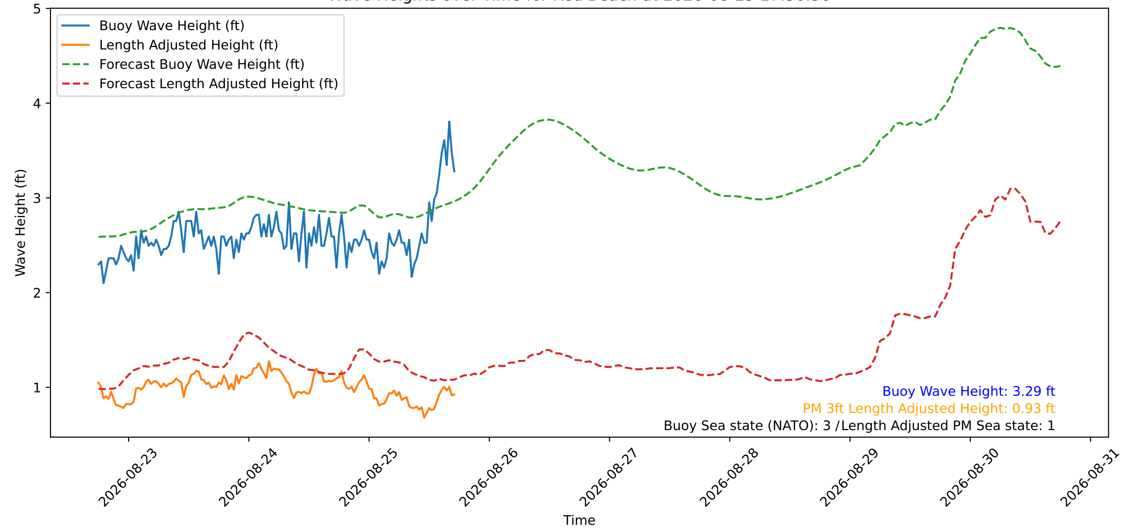
Wave Heights over Time for Red Beach at 2026-08-25 17:50:50
