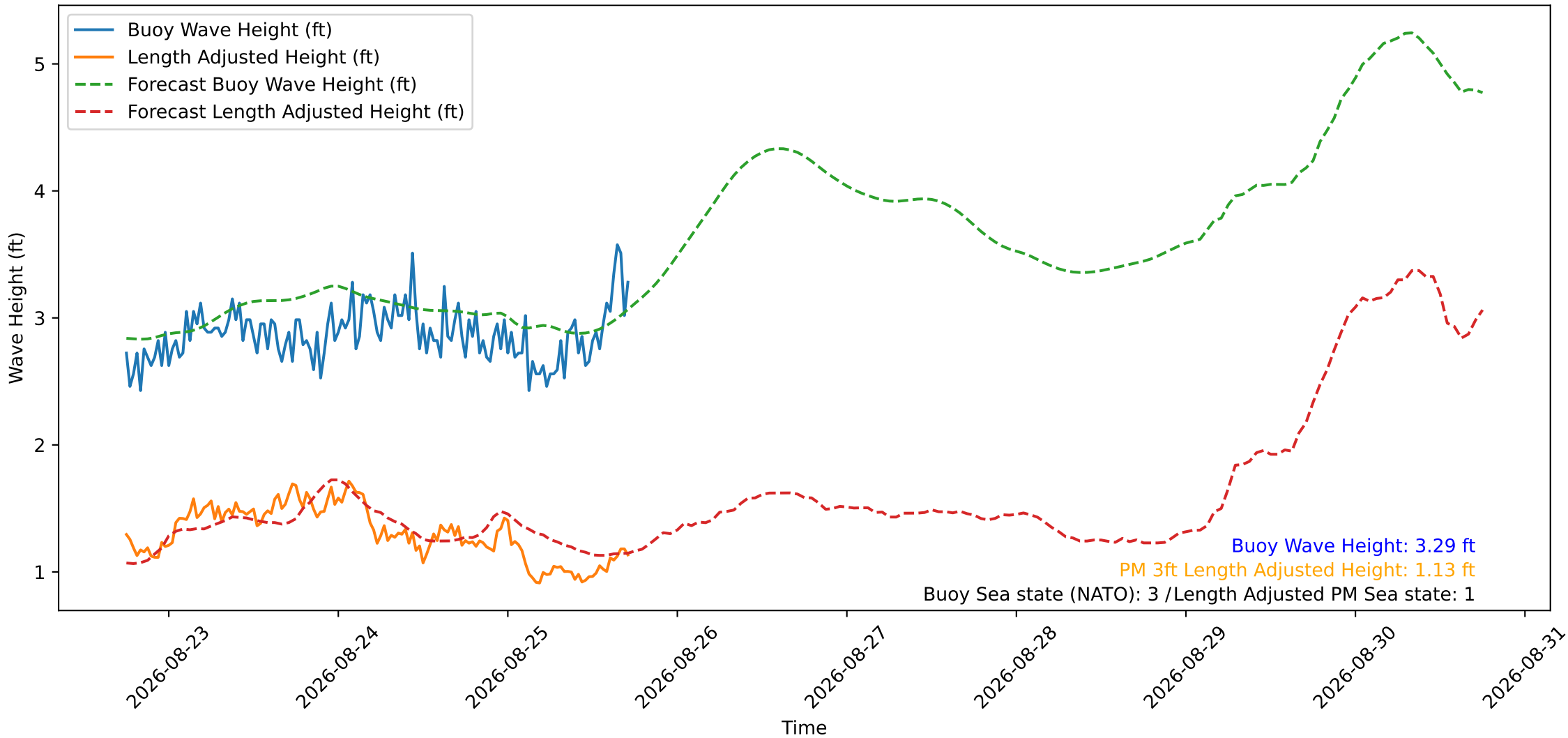
Wave Heights over Time for Oceanside Harbor at 2026-08-25 17:50:29
