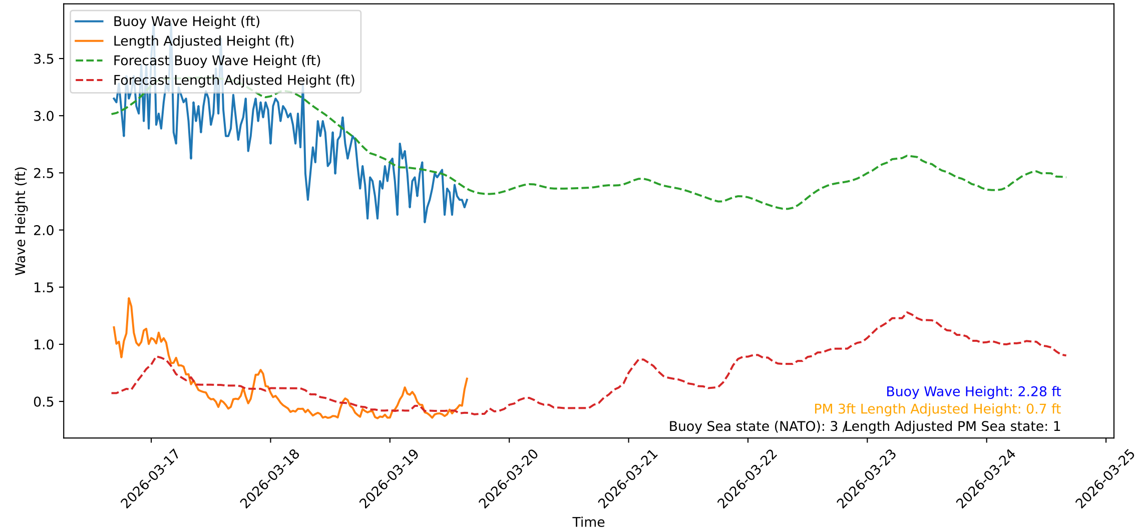
Wave Heights over Time for Red Beach at 2026-03-19 16:10:47
