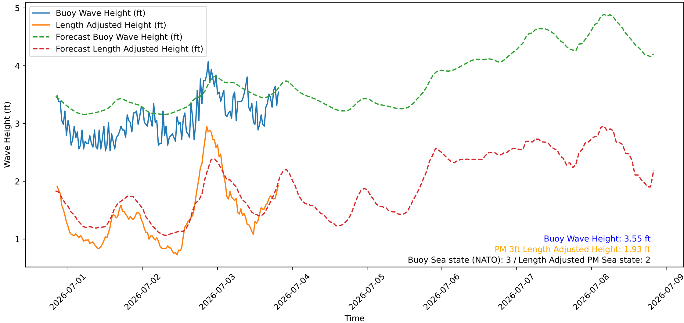
Wave Heights over Time for Green Beach at 2026-07-03 20:21:09
