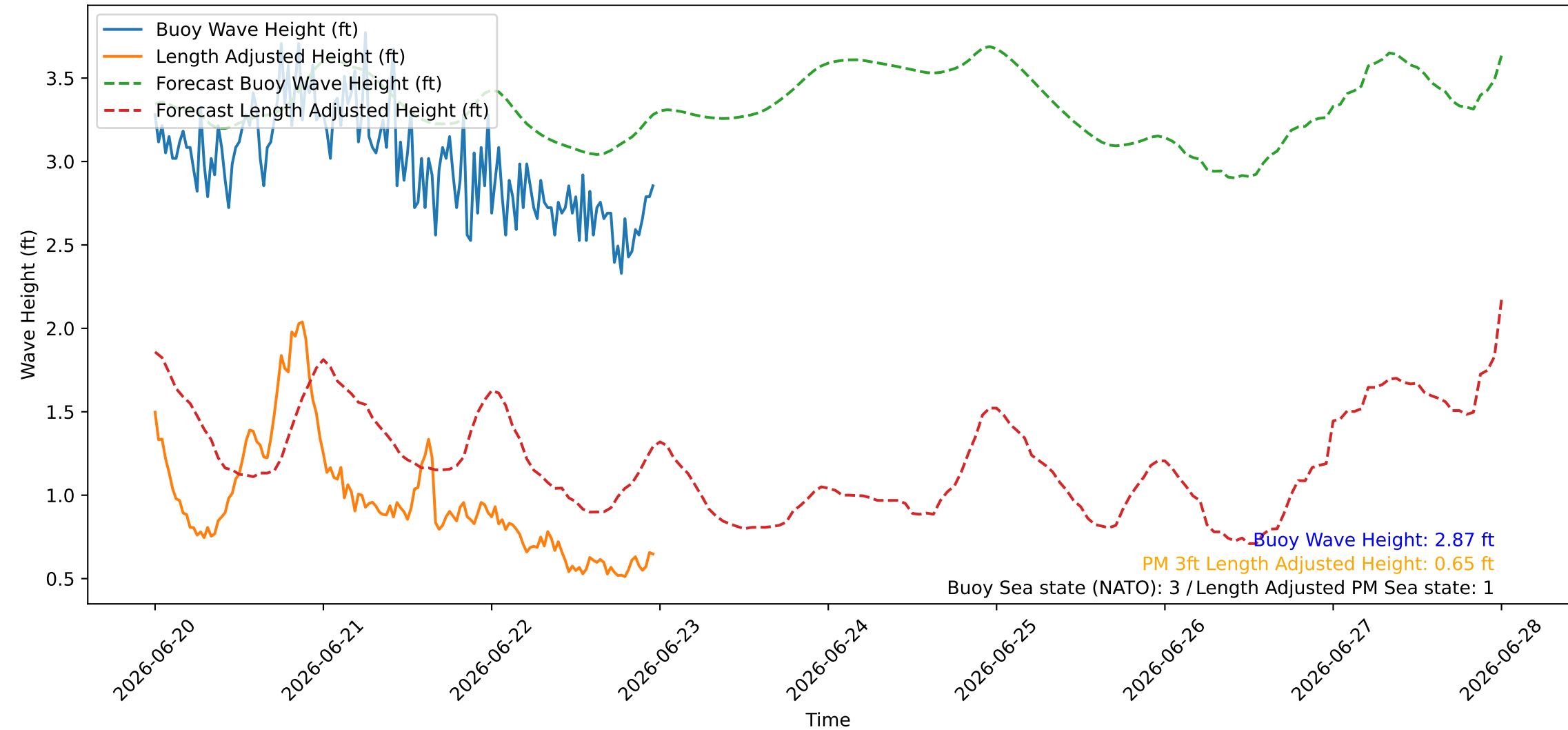
Wave Heights over Time for Red Beach at 2026-06-22 23:40:46
