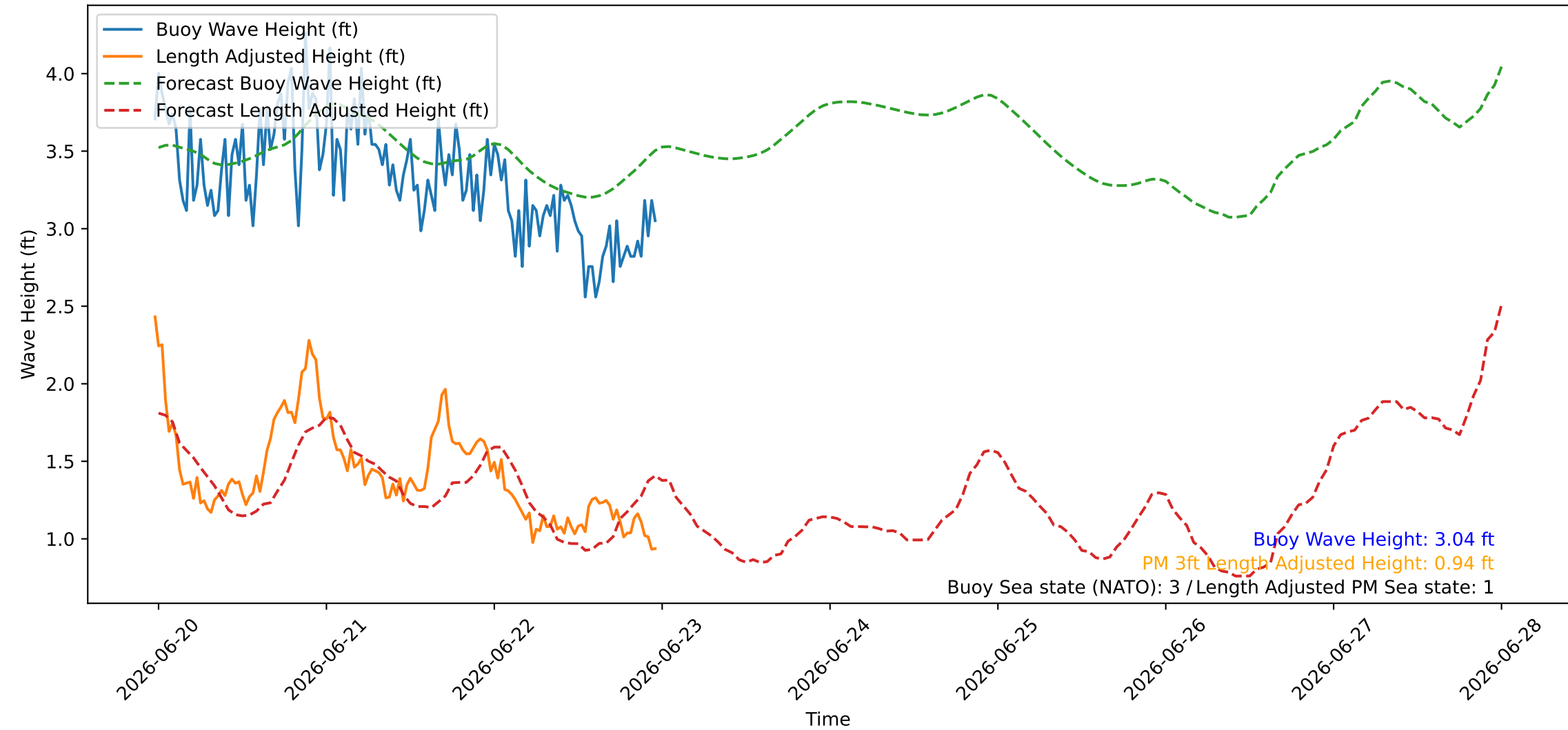
Wave Heights over Time for Oceanside Harbor at 2026-06-22 23:40:26
