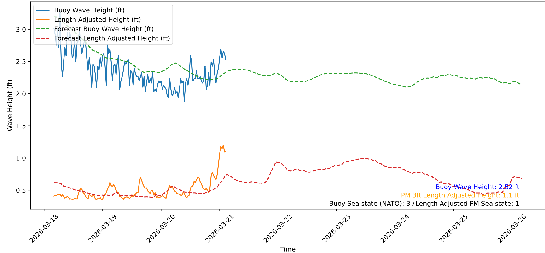
Wave Heights over Time for Red Beach at 2026-03-21 03:30:48
