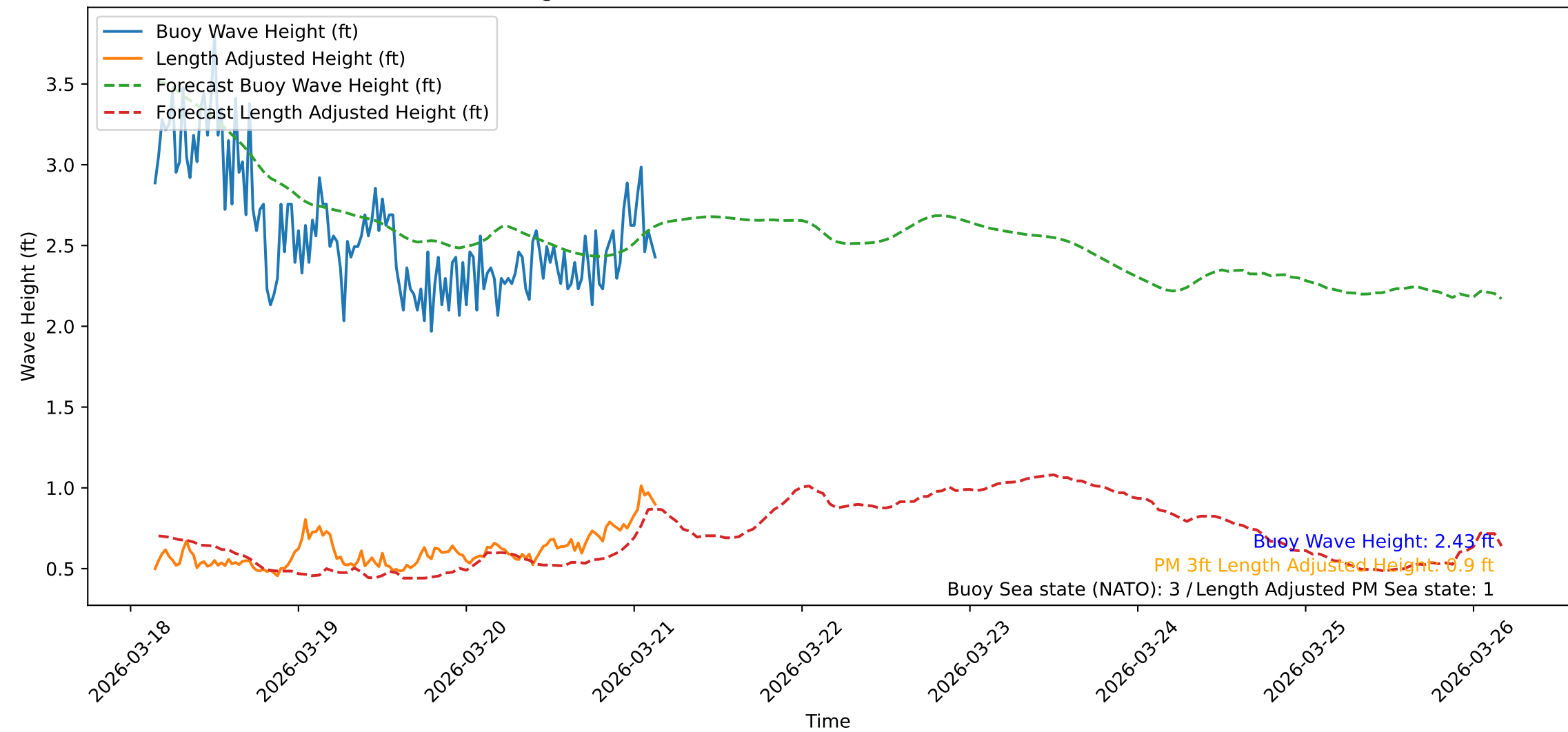
Wave Heights over Time for Oceanside Harbor at 2026-03-21 03:30:32
