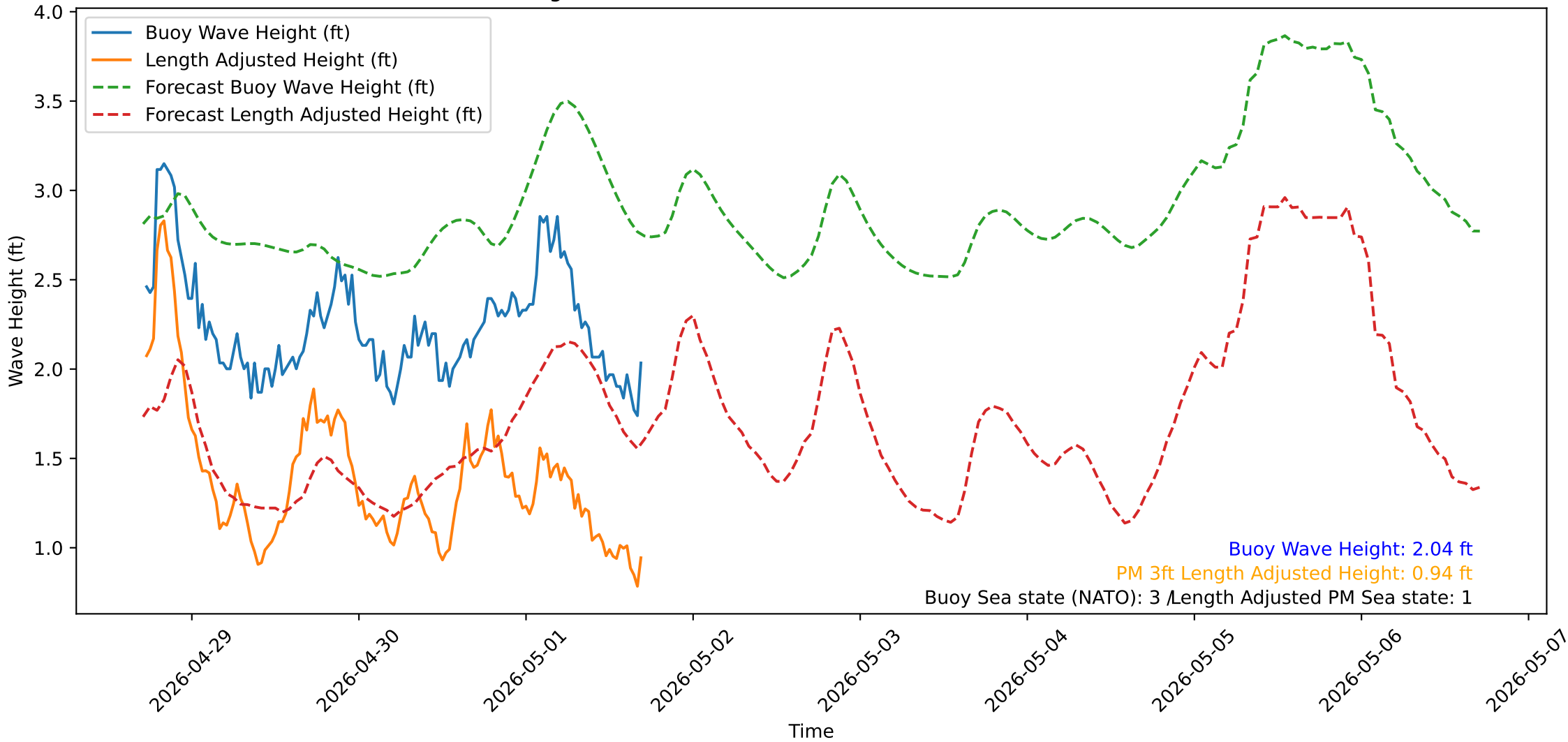
Wave Heights over Time for Green Beach at 2026-05-01 17:21:14
