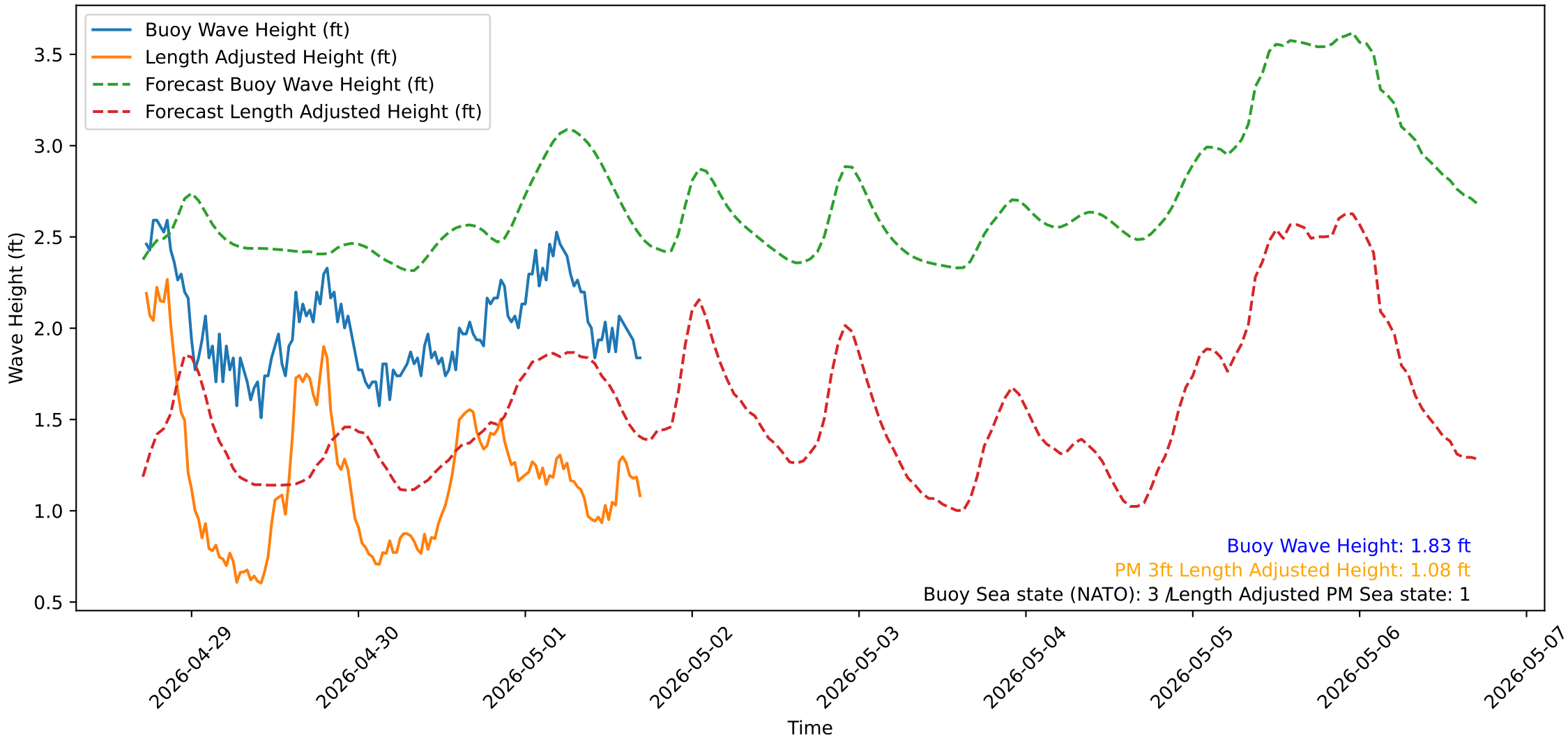
Wave Heights over Time for Red Beach at 2026-05-01 17:20:52
