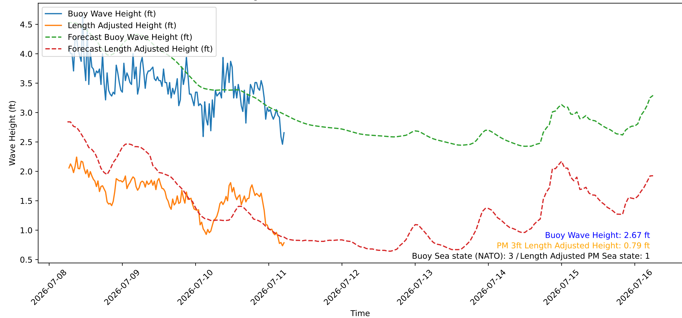
Wave Heights over Time for Red Beach at 2026-07-11 06:00:45
