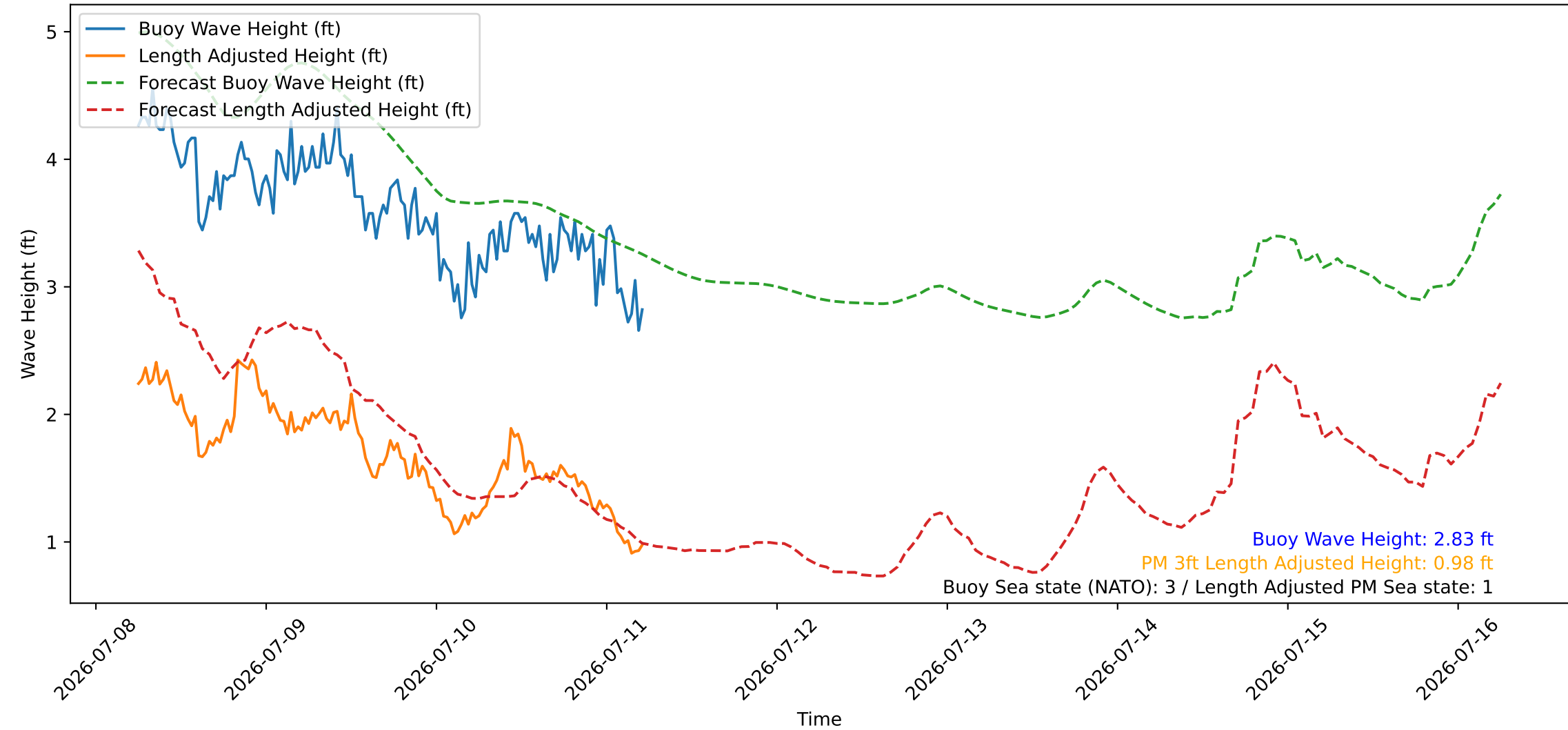
Wave Heights over Time for Green Beach at 2026-07-11 06:01:07
