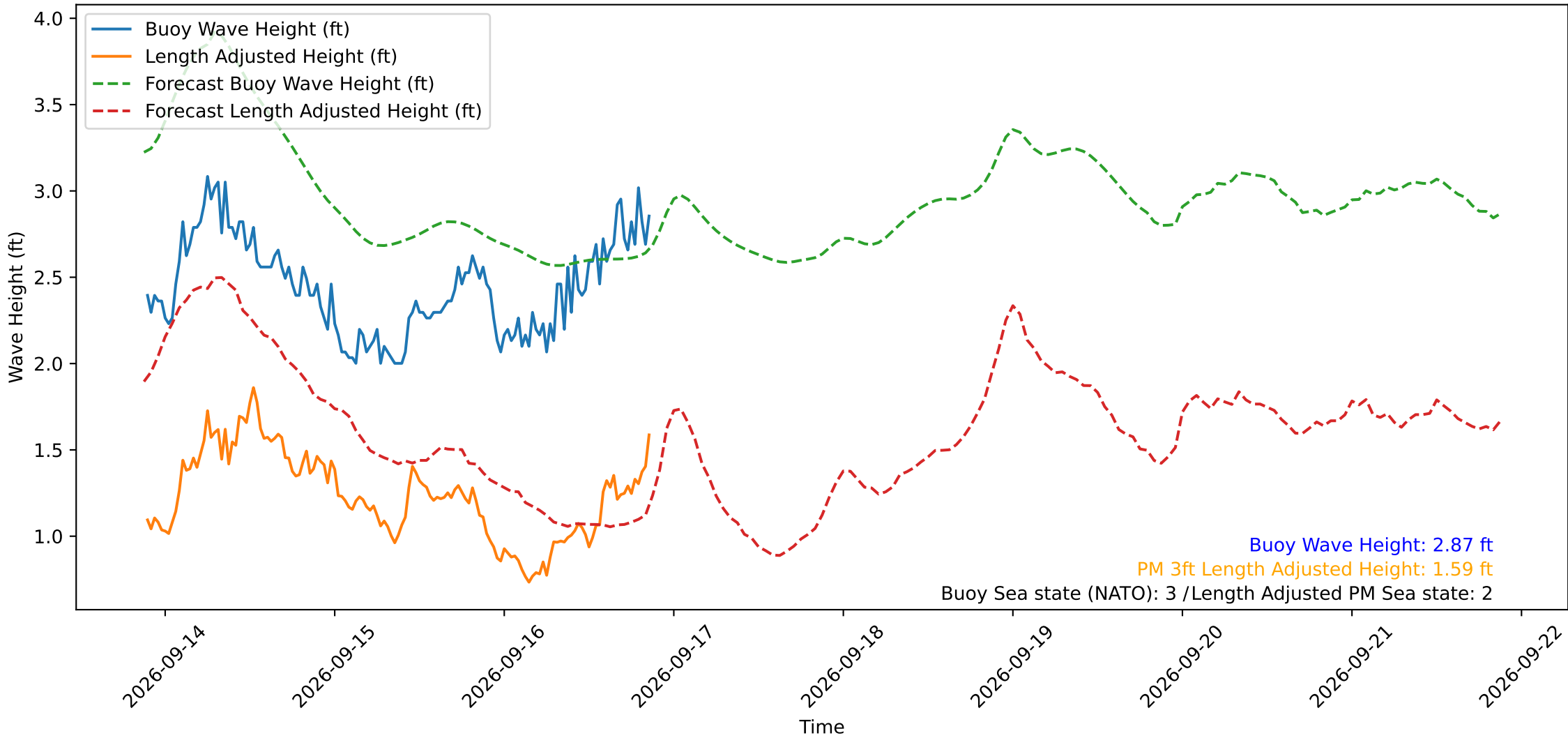
Wave Heights over Time for Red Beach at 2026-09-16 21:10:49
