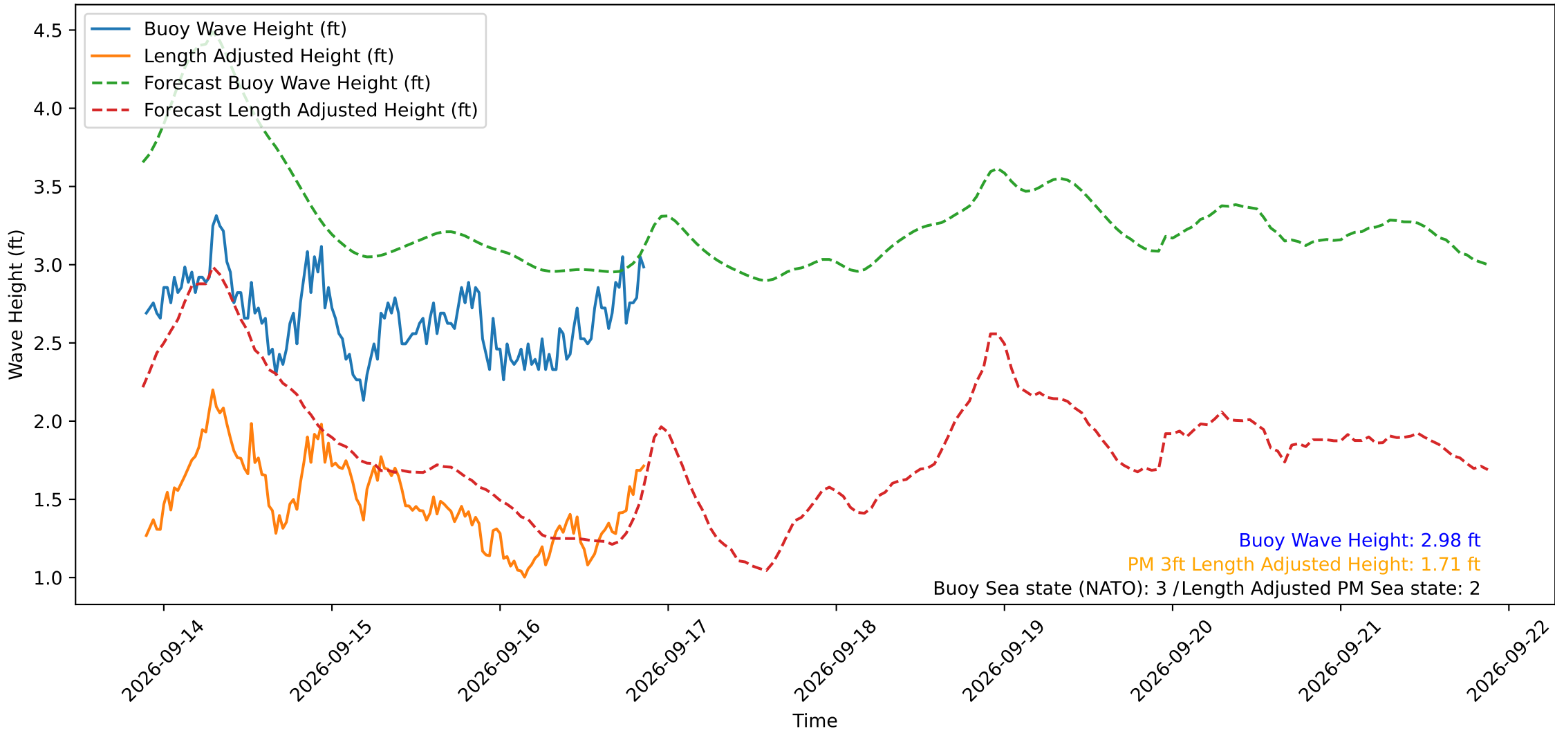
Wave Heights over Time for Green Beach at 2026-09-16 21:11:11
