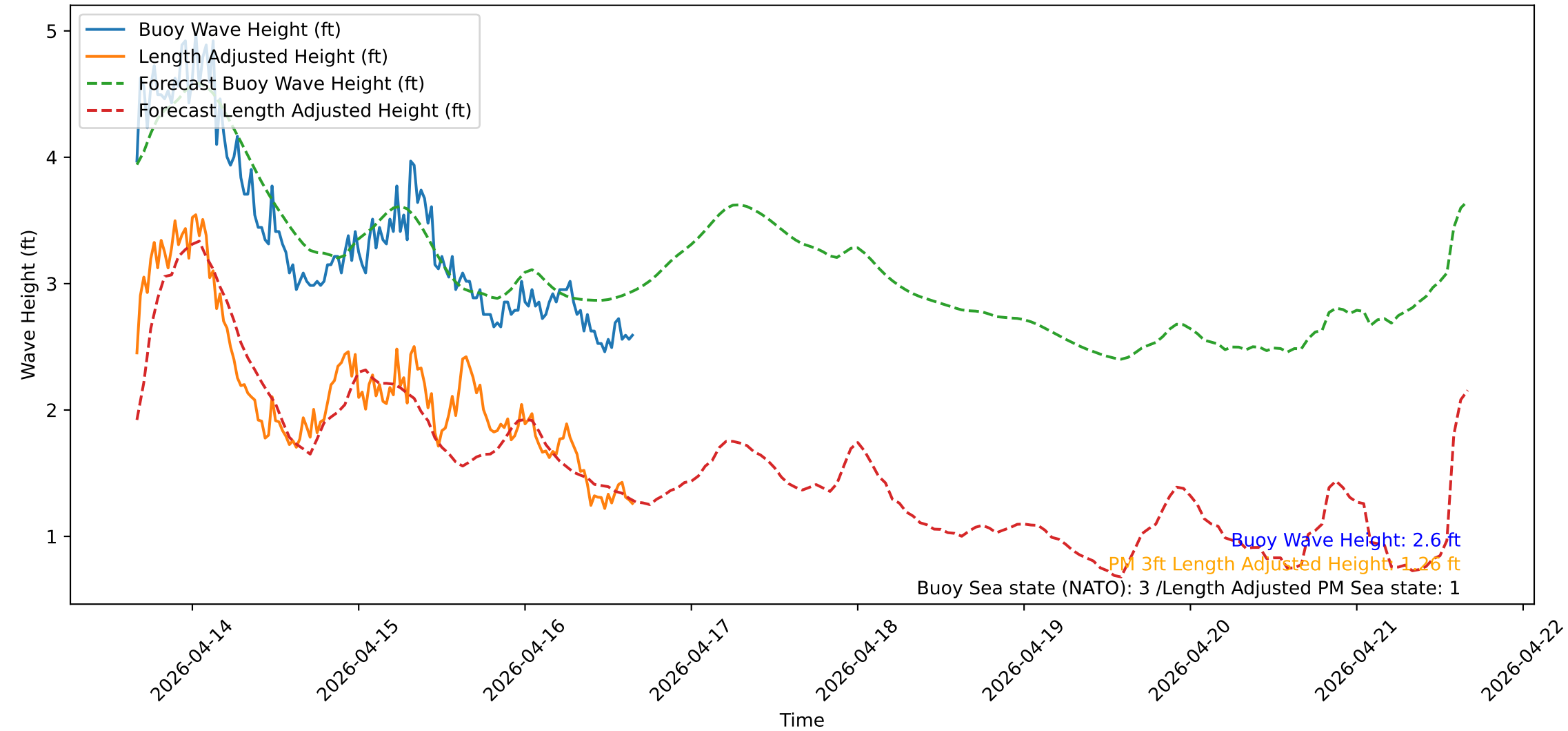
Wave Heights over Time for Green Beach at 2026-04-16 16:11:13
