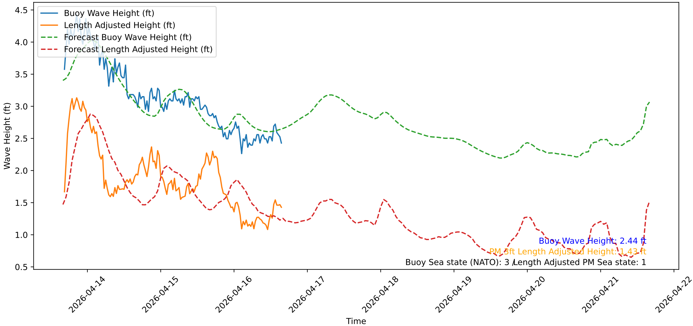
Wave Heights over Time for Red Beach at 2026-04-16 16:10:50
