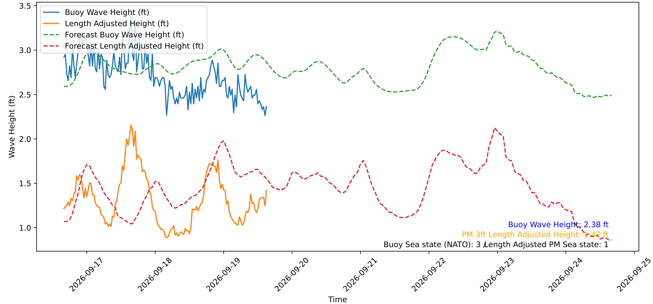
Wave Heights over Time for Red Beach at 2026-09-19 15:50:51
