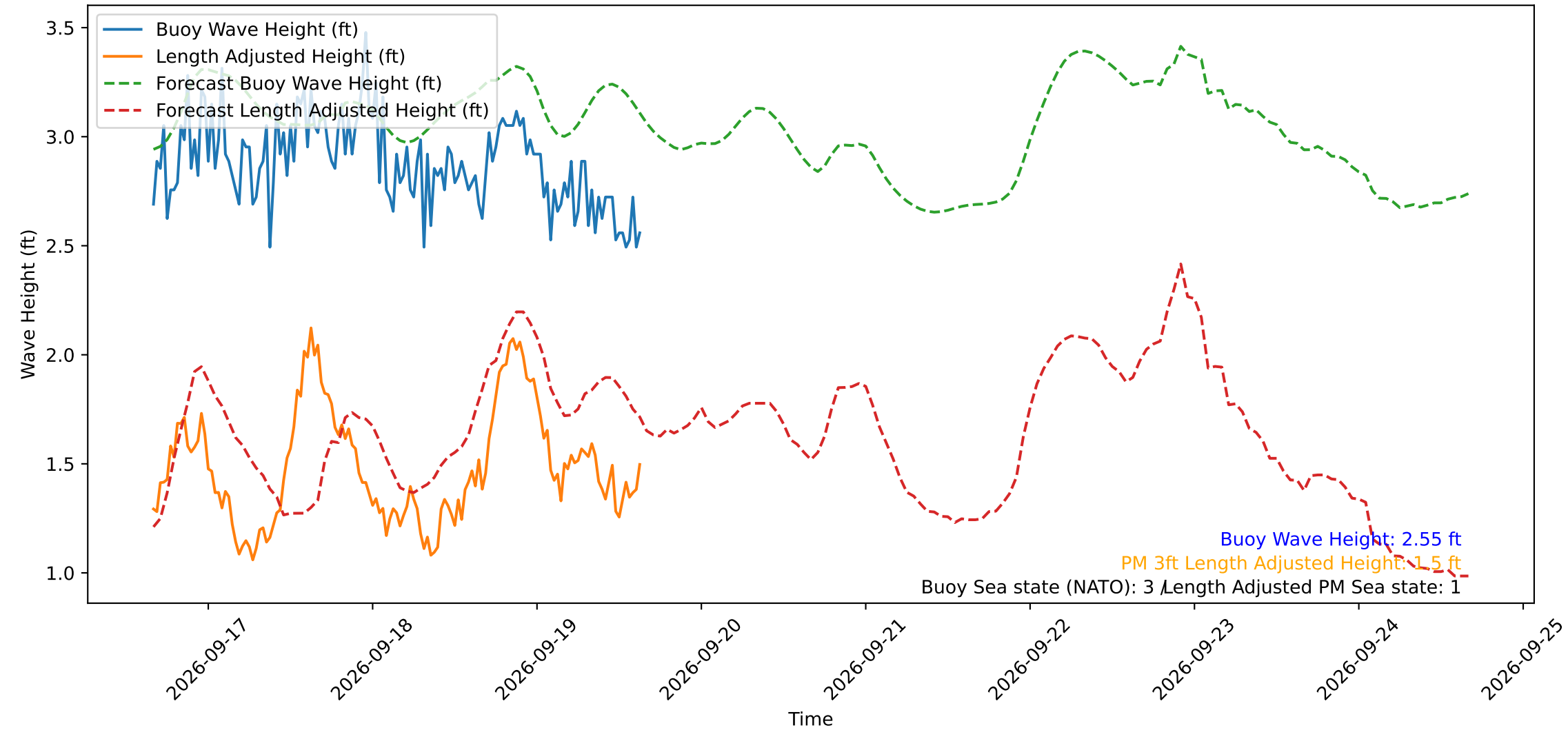
Wave Heights over Time for Green Beach at 2026-09-19 15:51:15
