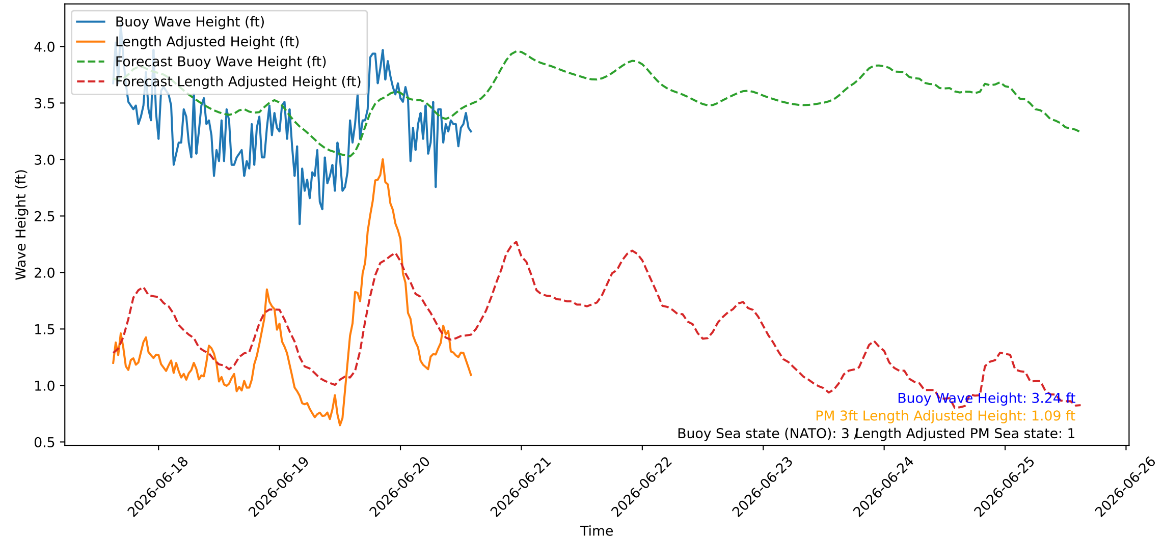
Wave Heights over Time for Green Beach at 2026-06-20 15:01:07
