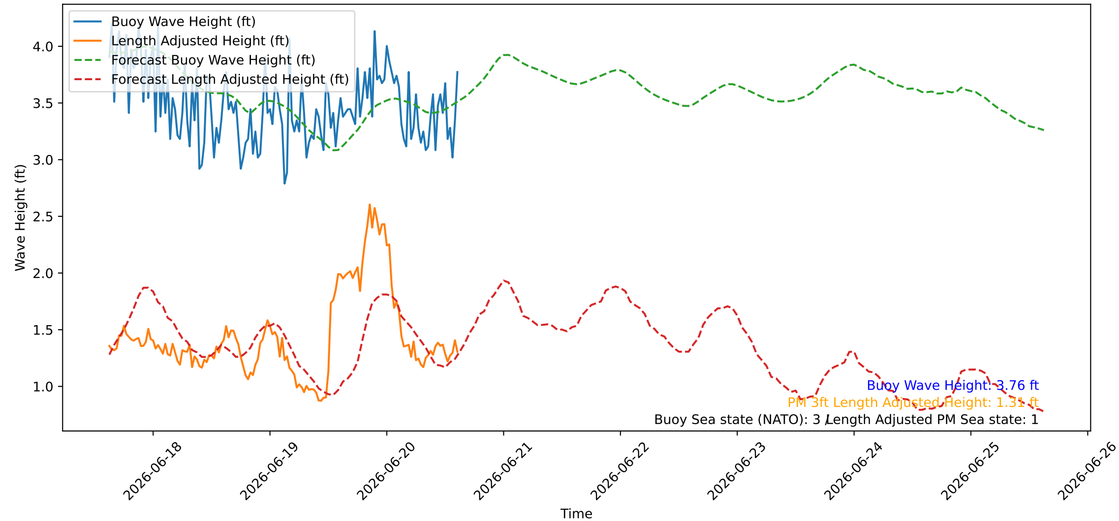
Wave Heights over Time for Oceanside Harbor at 2026-06-20 15:00:26
