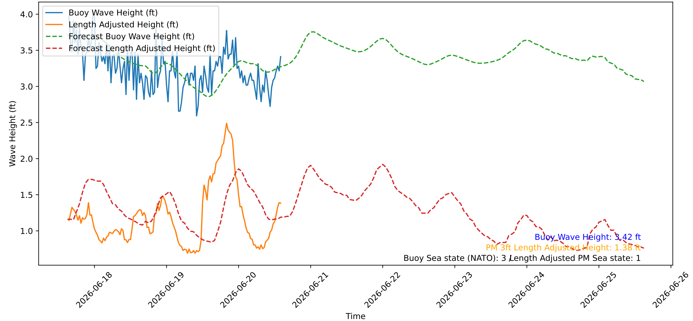
Wave Heights over Time for Red Beach at 2026-06-20 15:00:45
