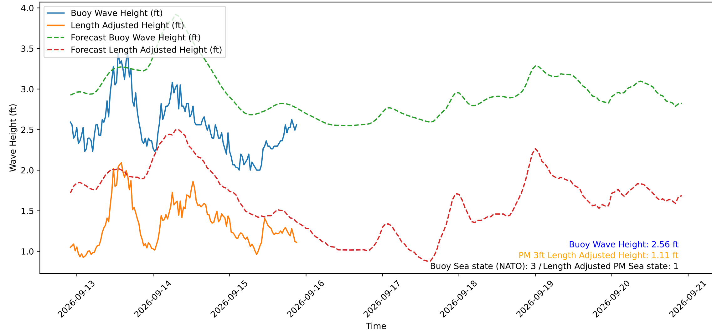
Wave Heights over Time for Red Beach at 2026-09-15 21:40:49
