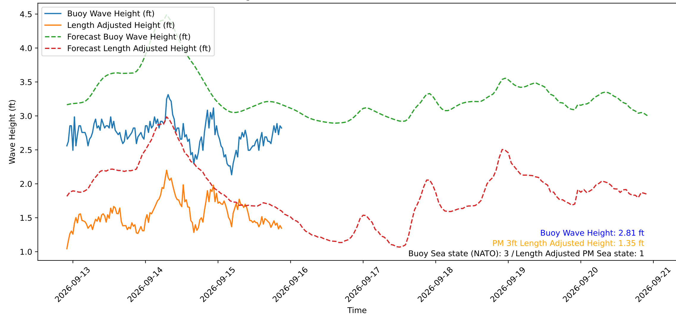
Wave Heights over Time for Green Beach at 2026-09-15 21:41:12
