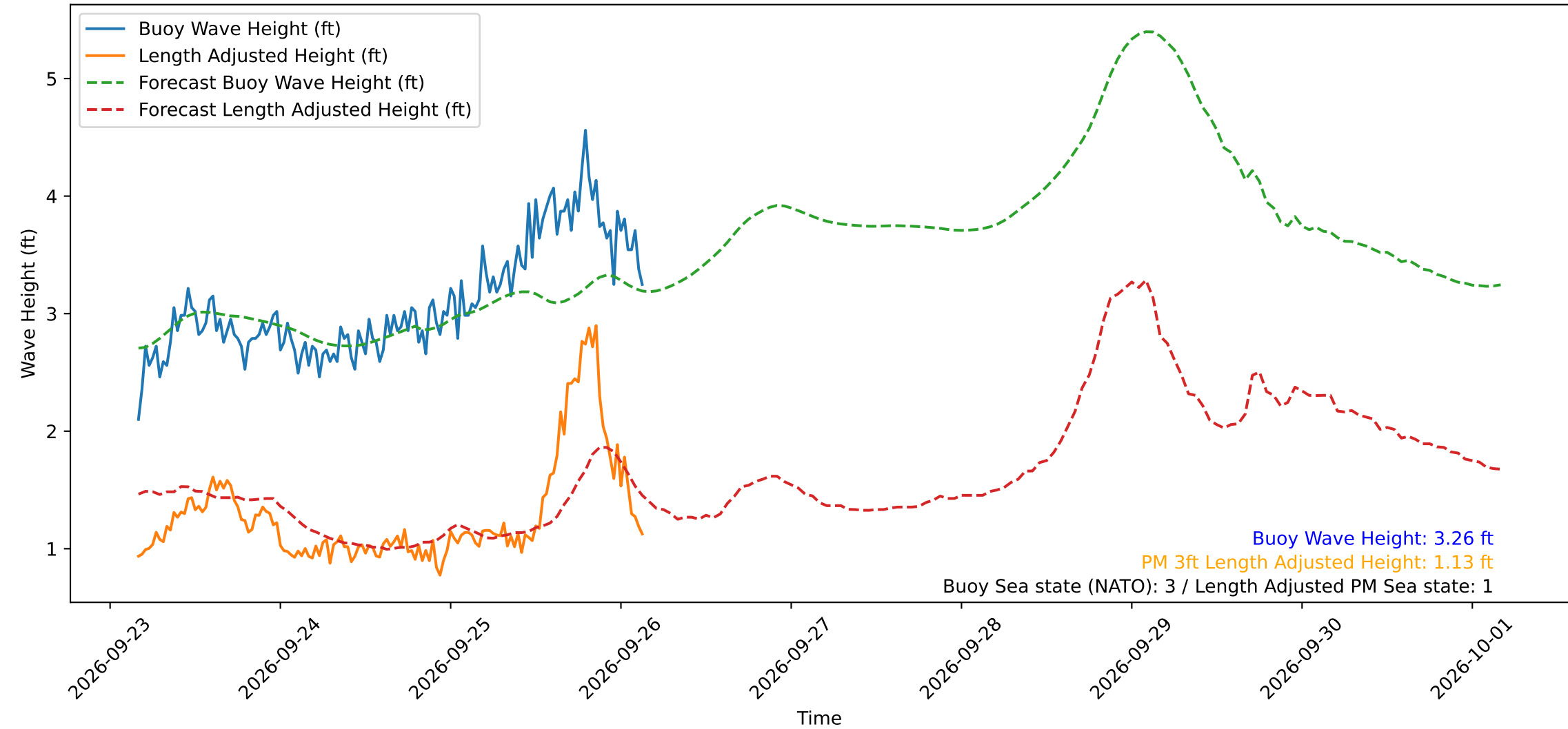
Wave Heights over Time for Green Beach at 2026-09-26 03:41:11
