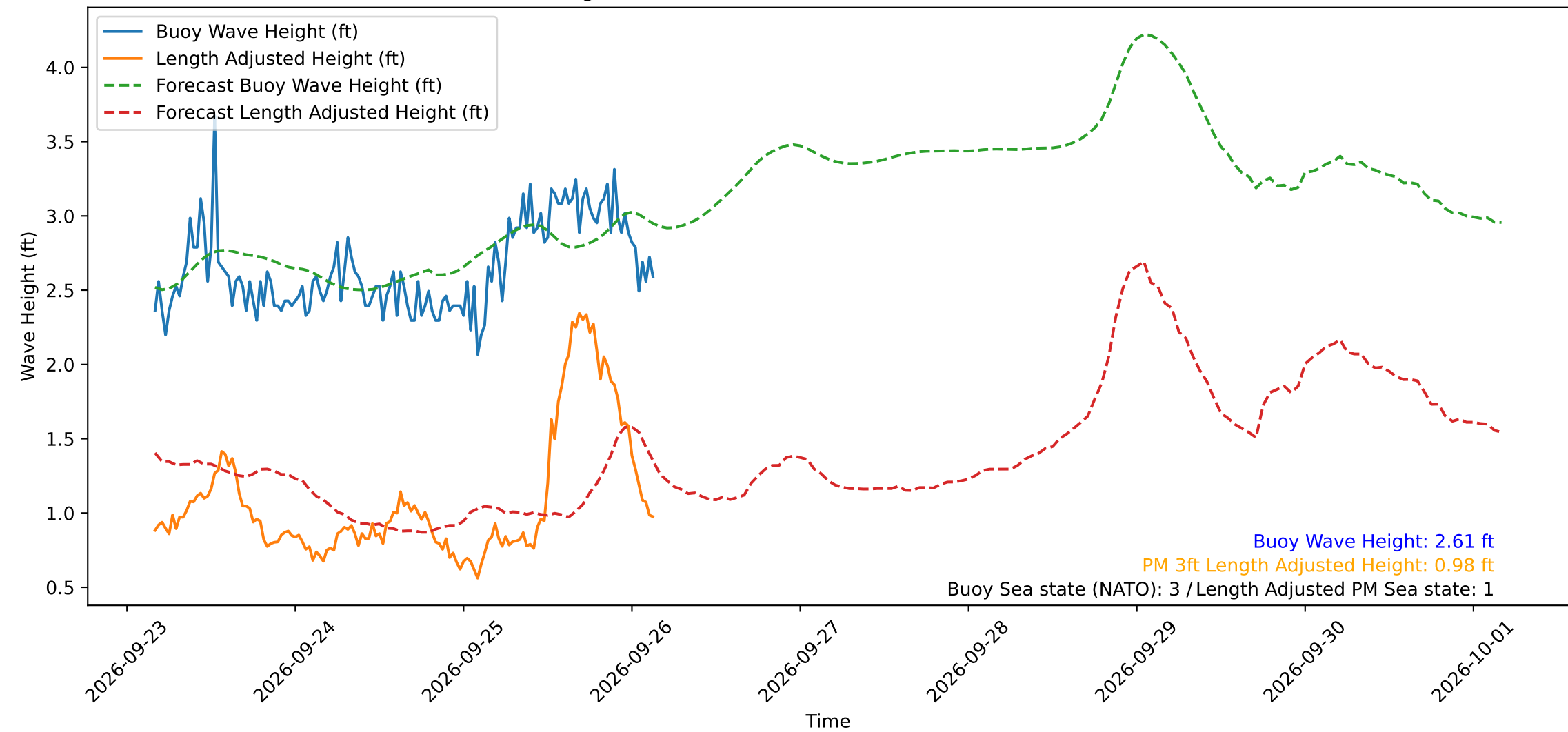
Wave Heights over Time for Red Beach at 2026-09-26 03:40:49
