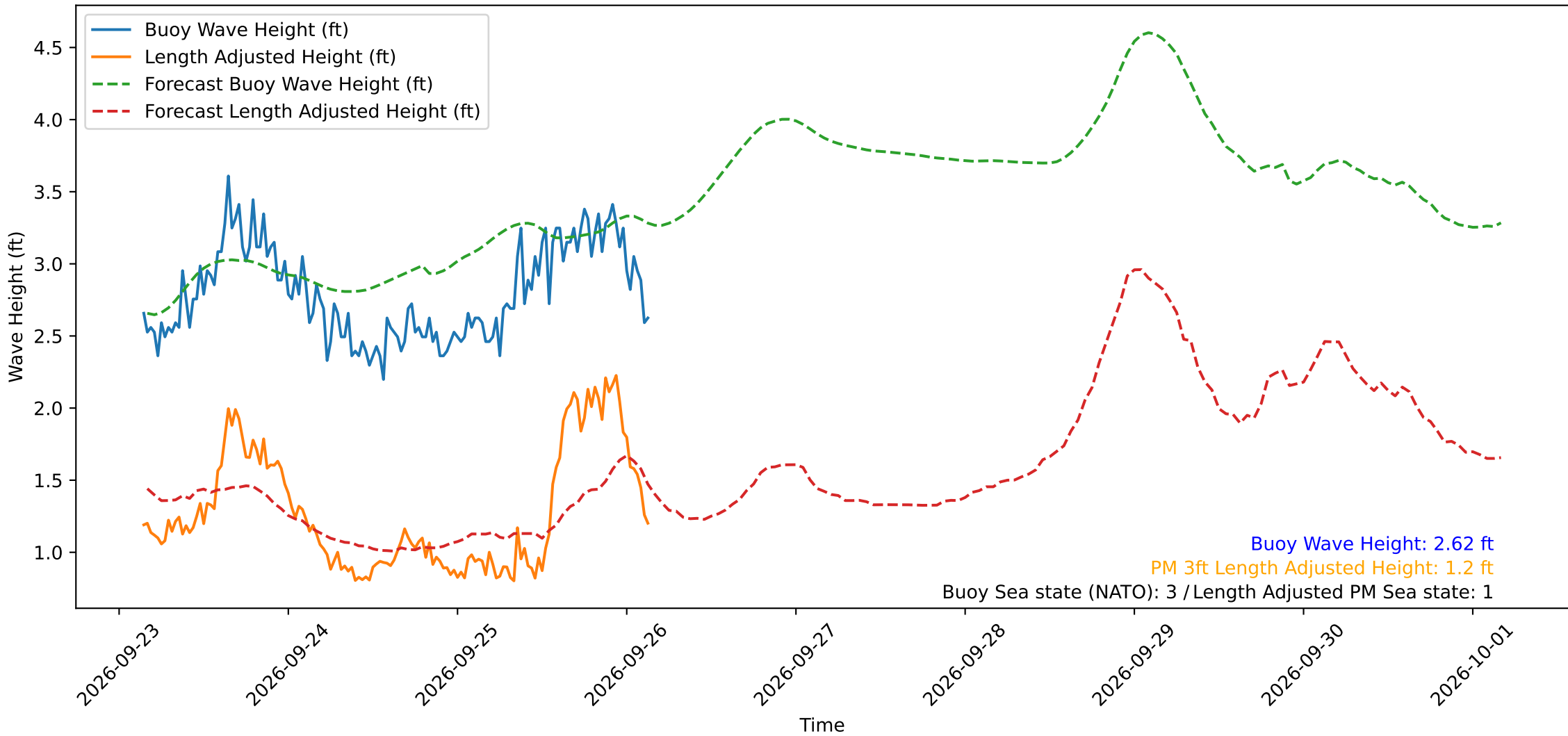
Wave Heights over Time for Oceanside Harbor at 2026-09-26 03:40:29
