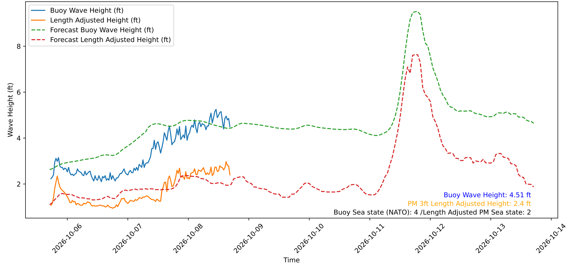
Wave Heights over Time for Green Beach at 2026-10-08 17:11:12
