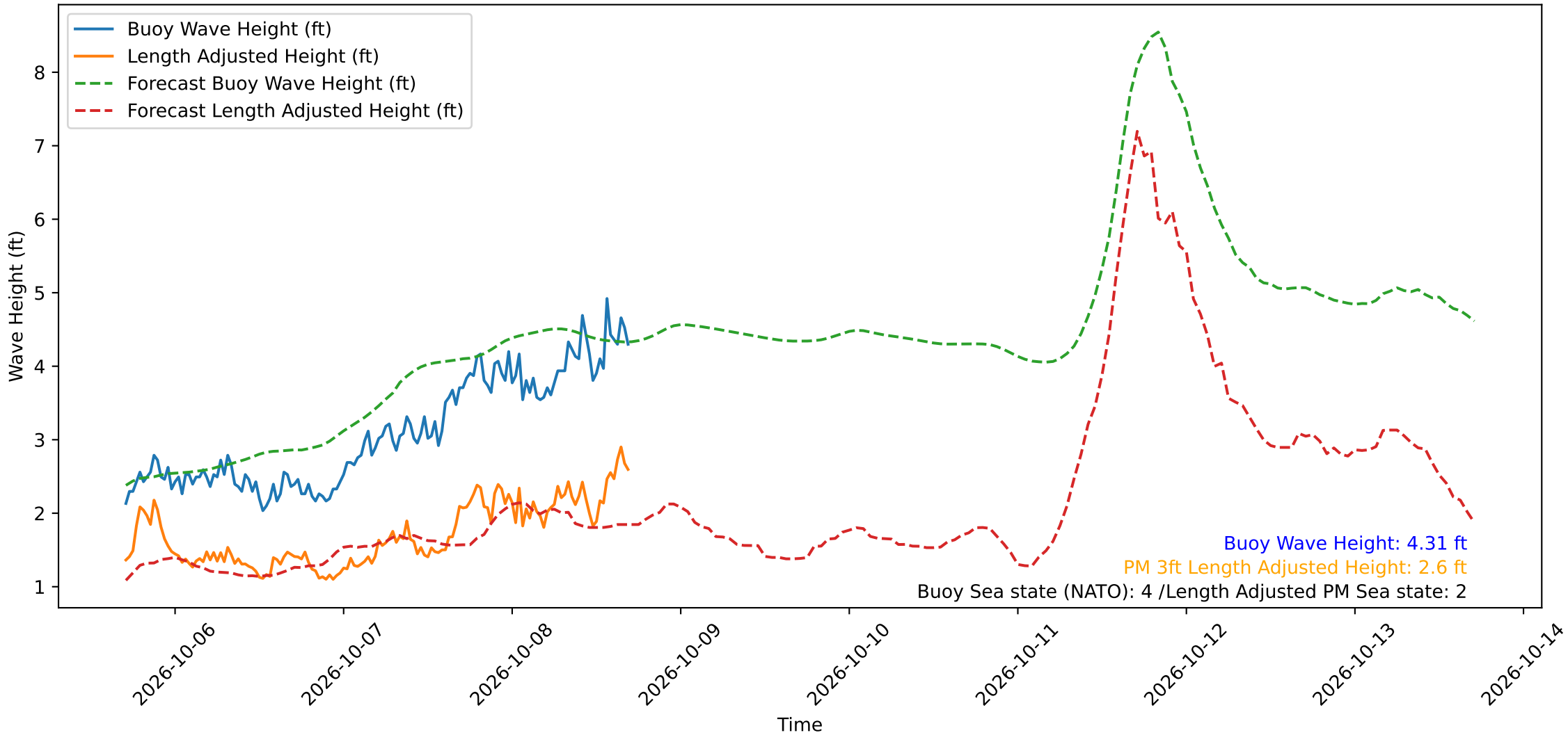
Wave Heights over Time for Oceanside Harbor at 2026-10-08 17:10:29
